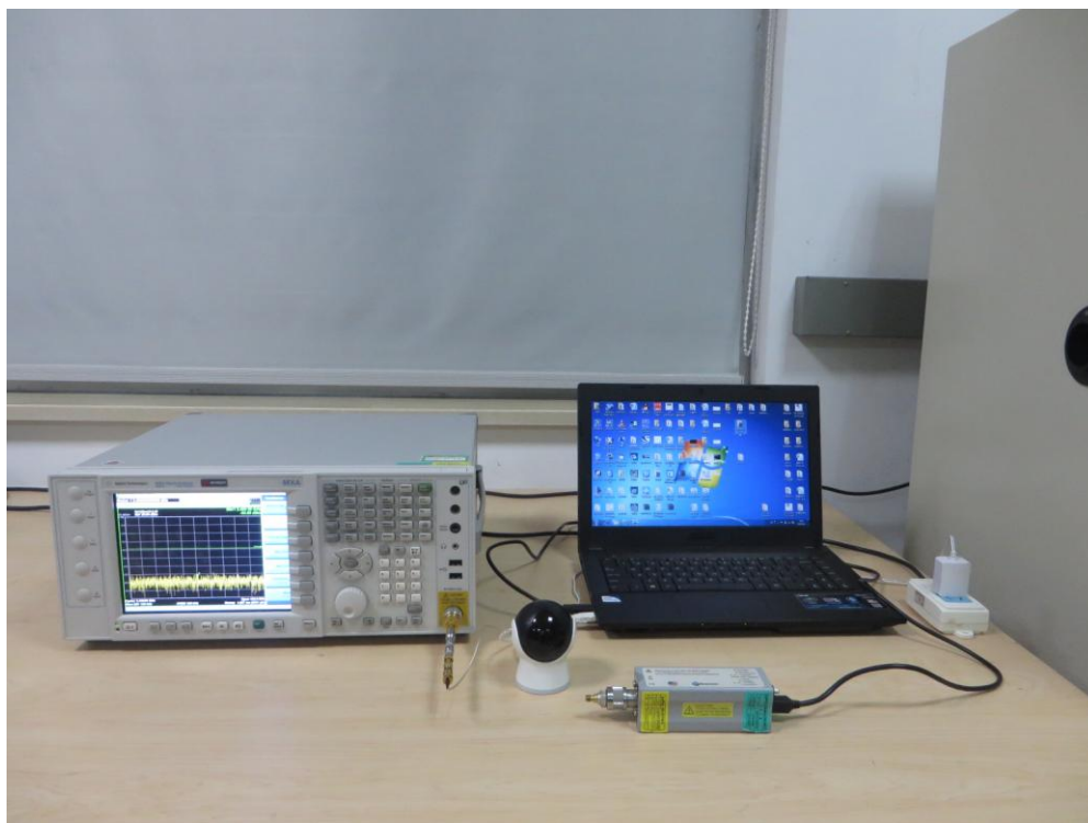
Description: Conducted Test Setup 2#
