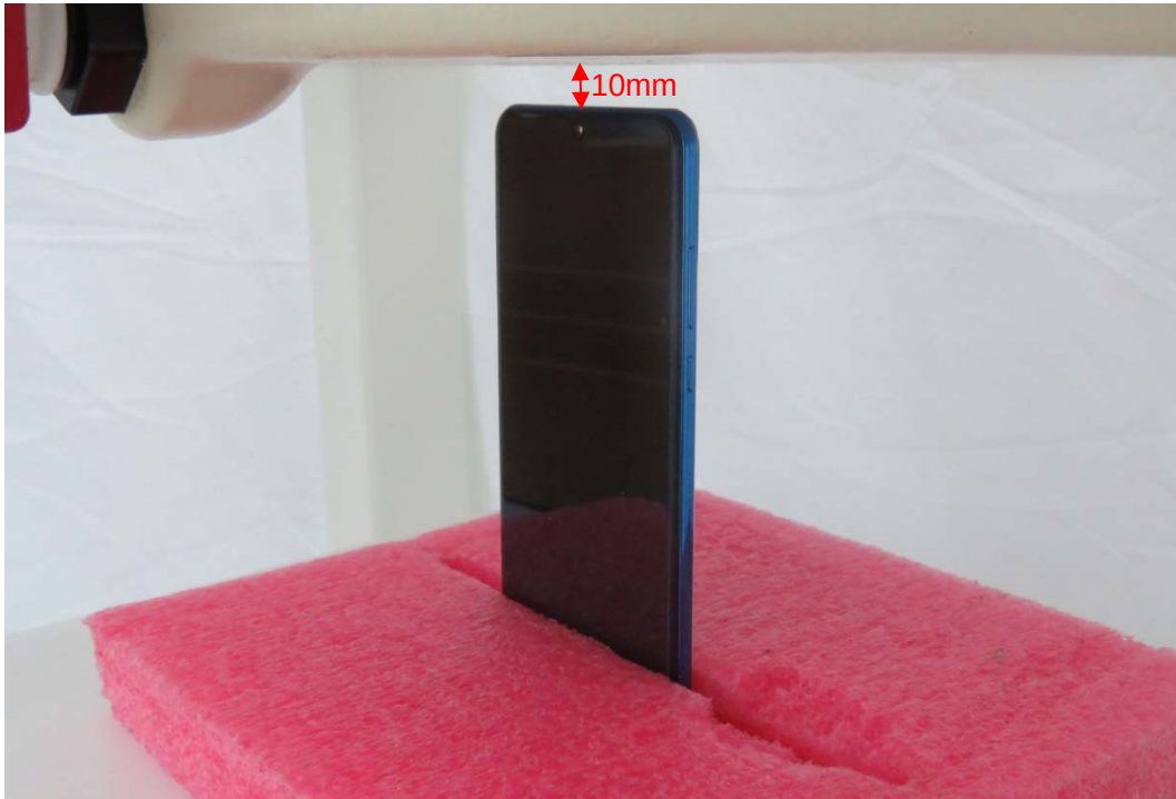
Picture 11: Top Edge, the distance from handset to the bottom of the Phantom is 10mm
