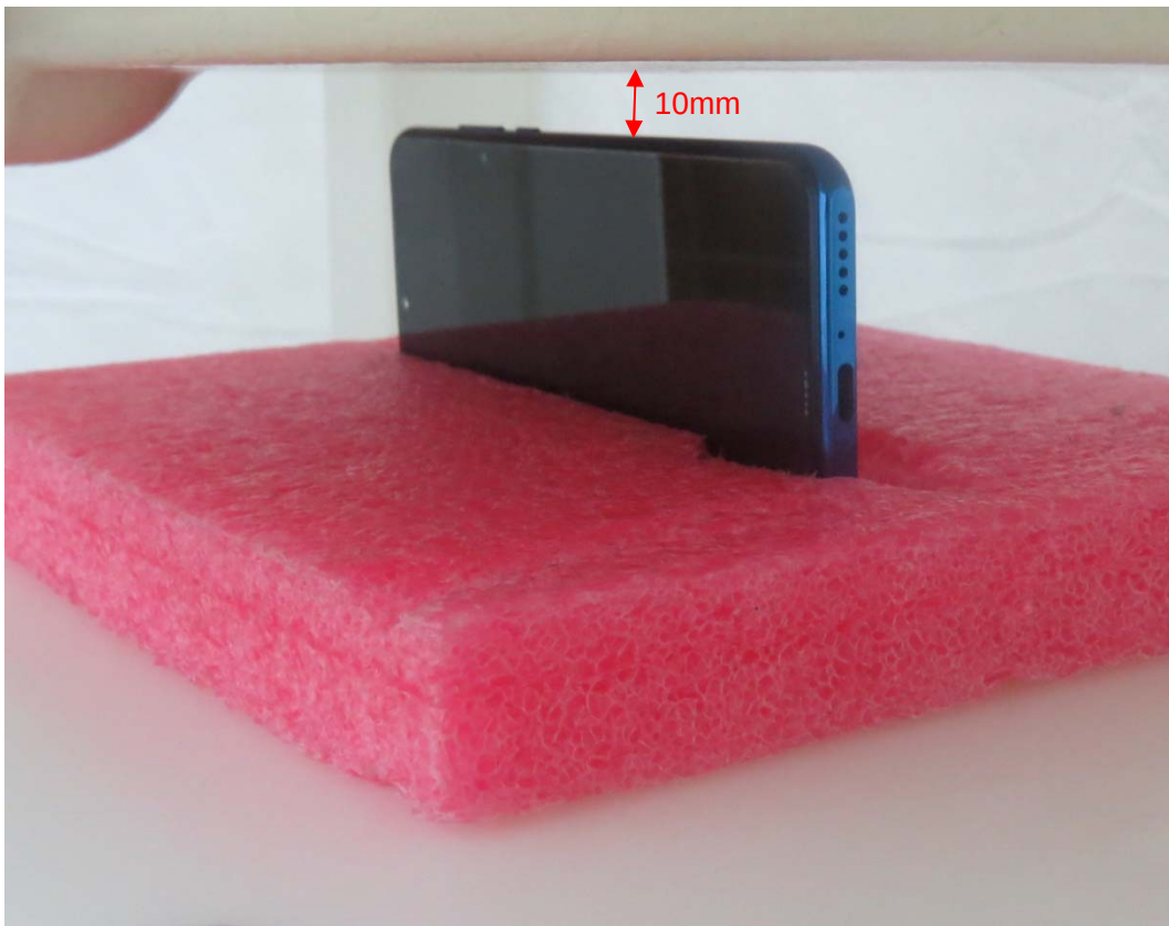
Picture 10: Right Edge, the distance from handset to the bottom of the Phantom is 10mm
