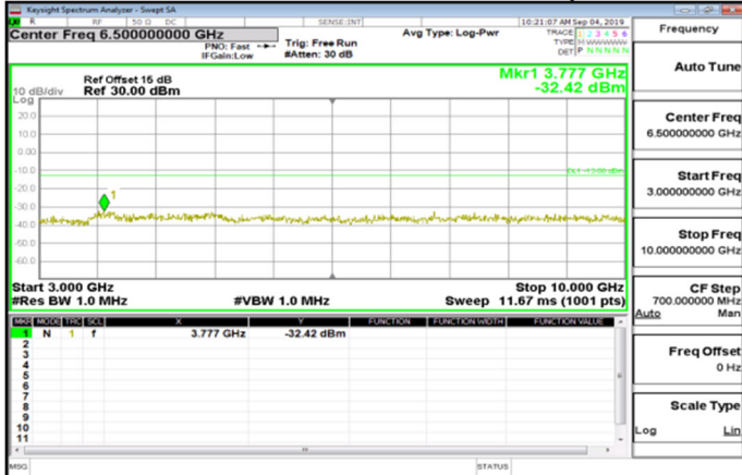
Cat_M1_3GHz~10GHz_Band26_Part90s_3MHz_QPSK_1_0_HighCH26775-822.5
