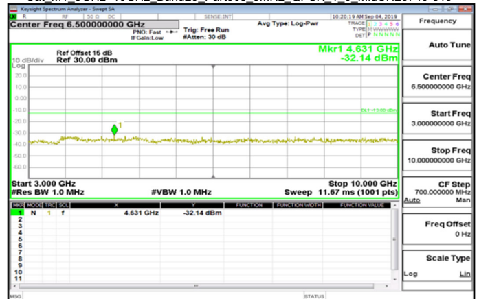
Cat M1_3GHz~10GHz_Band26_Part90s_3MHz_QPSK_1_0_MidCH26740-819
