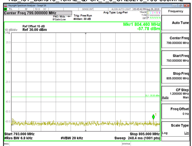
NB_IoT_Band13_15kHz_QPSK_1_0_CH23279_793-805MHz
