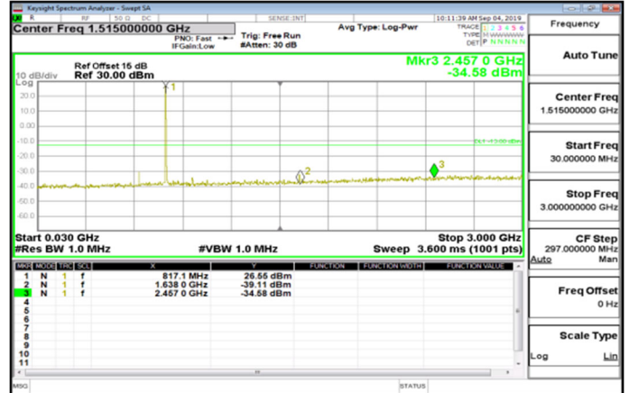
Cat_M1_30MHz~3GHz_Band26_Part90s_5MHz_QPSK_1_0_MidCH26740-819
