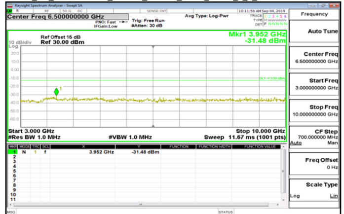
Cat_M1_3GHz~10GHz_Band26_Part90s_5MHz_QPSK_1_0_MidCH26740-819
