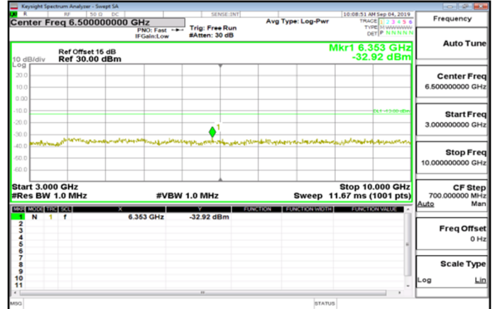
Cat_M1_3GHz~10GHz_Band26_Part90s_5MHz_QPSK_1_0_LowCH26715-816.5
