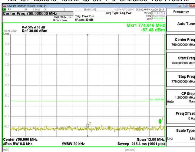
NB_IoT_Band13_15kHz_QPSK_1_0_CH23230_763-775MHz
