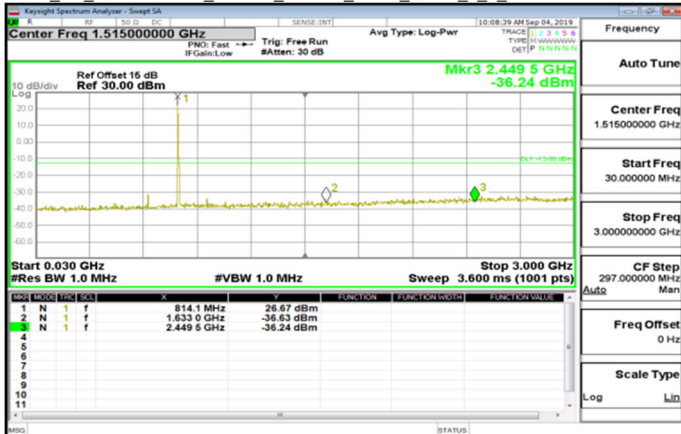
Cat_M1_30MHz~3GHz_Band26_Part90s_5MHz_QPSK_1_0_LowCH26715-816.5
