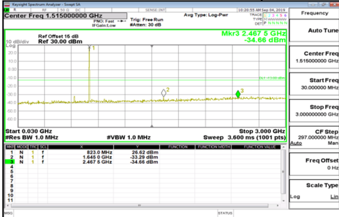
Cat_M1_30MHz~3GHz_Band26_Part90s_3MHz_QPSK_1_0_HighCH26775-822.5
