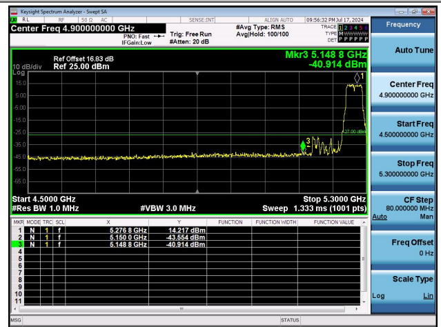
11N40MIMO-Ant1-5310-PASS
