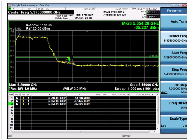
11AC80MIMO-Ant0-5290-PASS
