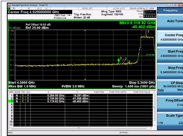
11AX80MIMO-Ant1-5290-PASS
