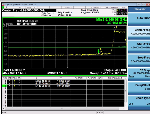
11AC80MIMO-Ant1-5290-PASS
