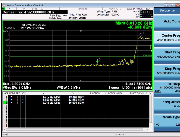
11AC160MIMO-Ant0-5250-PASS
