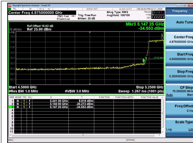
11AC160MIMO-Ant1-5250-PASS
