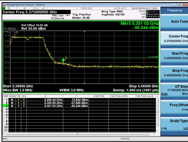
11A20MIMO-Ant0-5260-PASS
