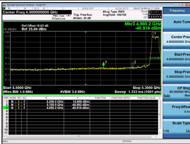
11AC40MIMO-Ant0-5310-PASS
