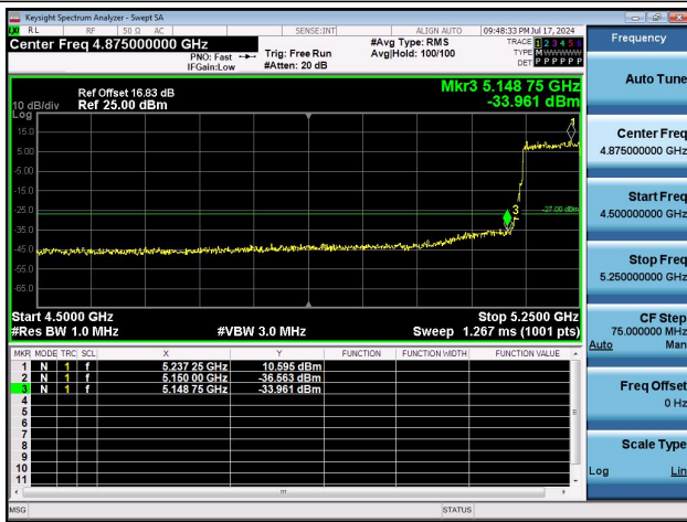
11AX160MIMO-Ant1-5250-PASS
