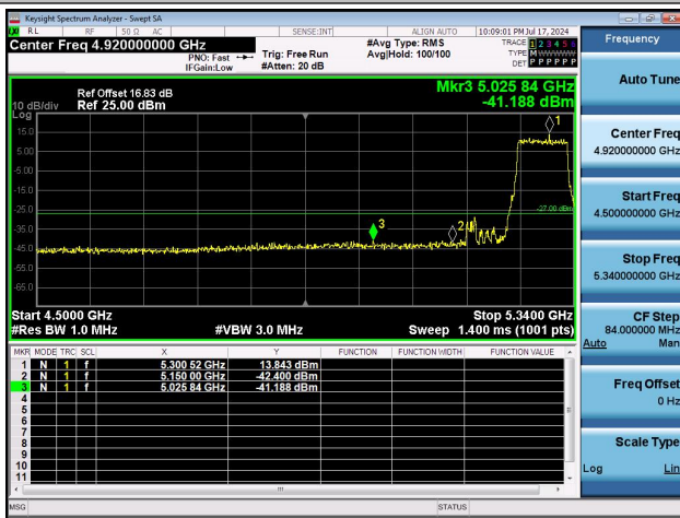
11AX160MIMO-Ant0-5250-PASS
