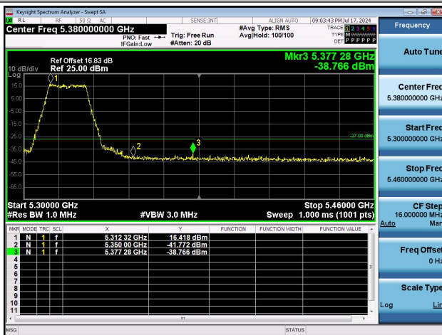
11AC40MIMO-Ant0-5270-PASS
