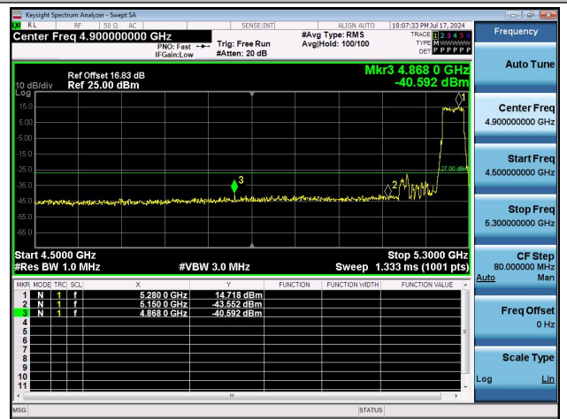
11AX40MIMO-Ant1-5310-PASS
