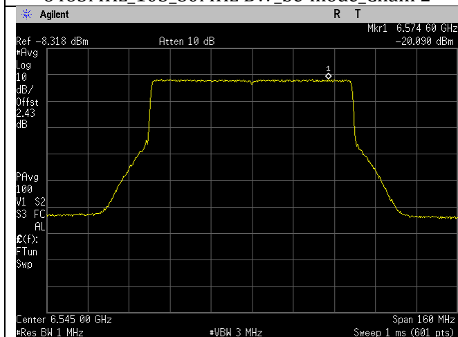
6545MHz_119_80MHz BW_be-mode_Chain 0
