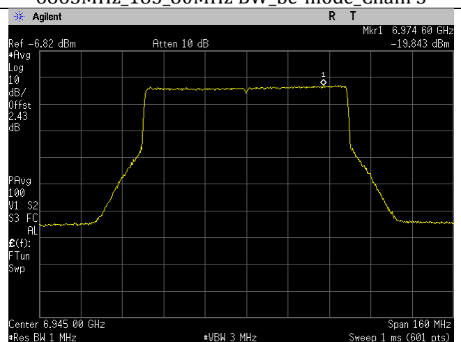
6945MHz_199_80MHz BW_be-mode_Chain 1
