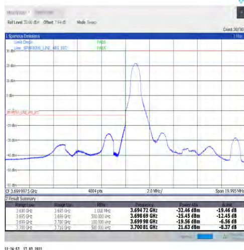
1-N77-3700-3980-30-10-L-4-CP-QPSK-Edge_1RB_Lef t-1@0-Ant1-PASS-see graph
