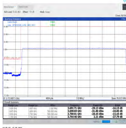
1-N77-3700-3980-30-60-L-6-CP-QPSK-Outer_Full -162@0-Ant1-PASS-see graph
