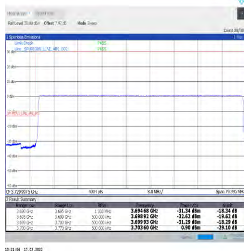
1-N77-3700-3980-30-70-L-6-CP-QPSK-Outer_Full -189@0-Ant1-PASS-see graph
