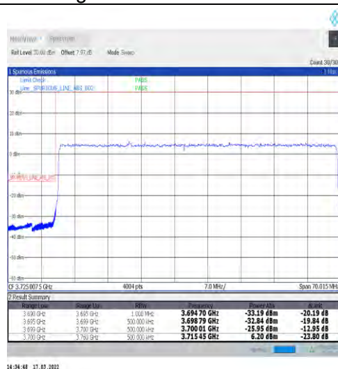
1-N77-3700-3980-30-60-L-3-DFT-PI2BPSK-Outer_Full-162@0-Ant1-PASS-see graph
