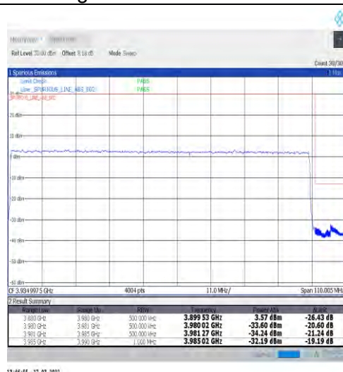
1-N77-3700-3980-30-100-H-3-DFT-PI2BPSK-Outer_Full-270@0-Ant1-PASS-see graph
