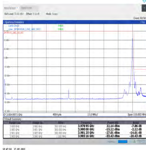
1-N77-3700-3980-30-100-H-5-CP-QPSK-Edge_1RB_Right-1@272-Ant1-PASS-see graph
