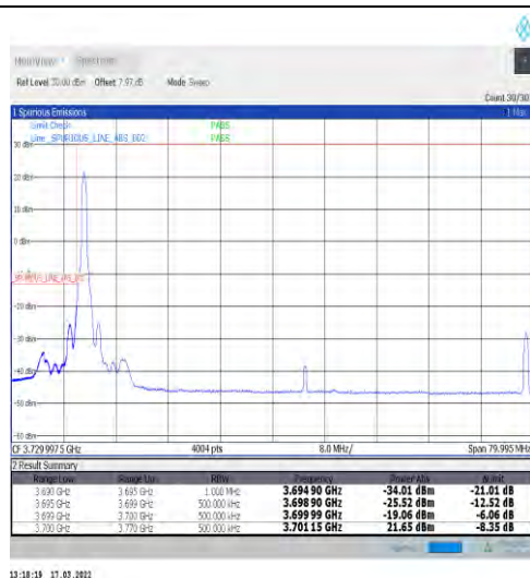
1-N77-3700-3980-30-70-L-1-DFT-PI2BPSK-Edge_1RB _Left-1@0-Ant1-PASS-see graph
