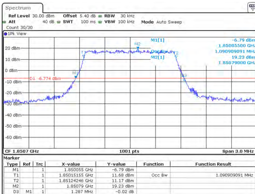
Band25-1.4MHz-QPSK-26047-6RB#0-1.091
