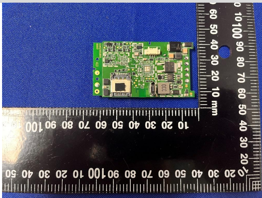
EUT WITHOUT SHIELDED SHELL
