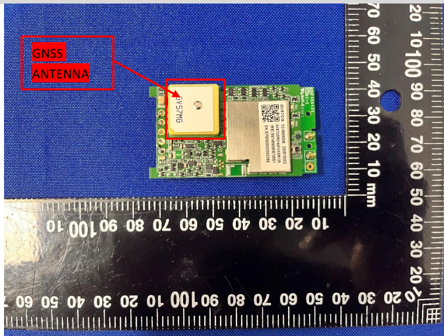
EUT WITH SHIELDED SHELL
