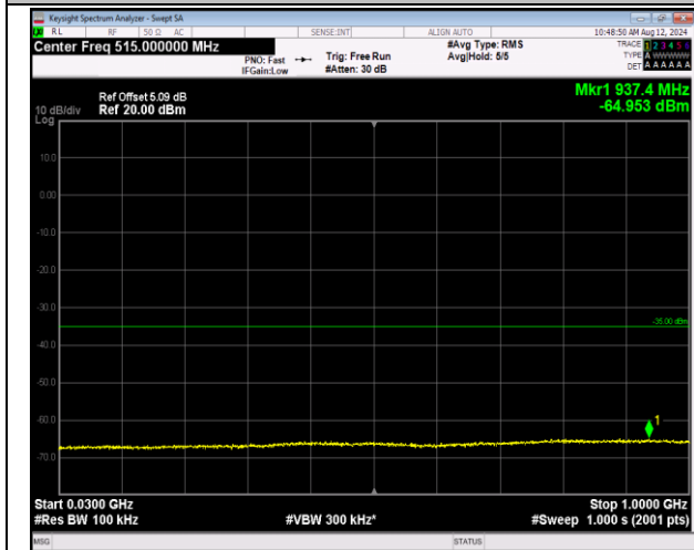
7-7-10MHz-20MHz-16QAM-16QAM-21206-21350-1RB#49 9-ORB#0-30~1000MHz-PASS
