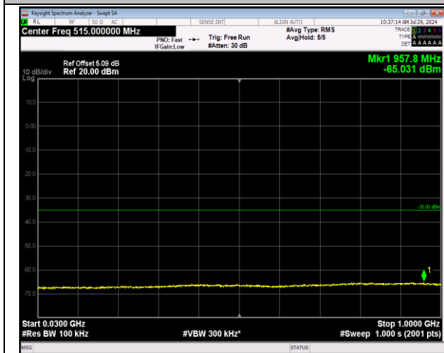
7-7-10MHz-20MHz-64QAM-64QAM-21006-21150-1RB#0 -1RB#99-30~1000MHz-PASS
