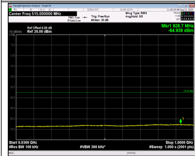
7-7-20MHz-10MHz-QPSK-QPSK-21051-21195-1RB#99-0 RB#0-30~1000MHz-PASS
