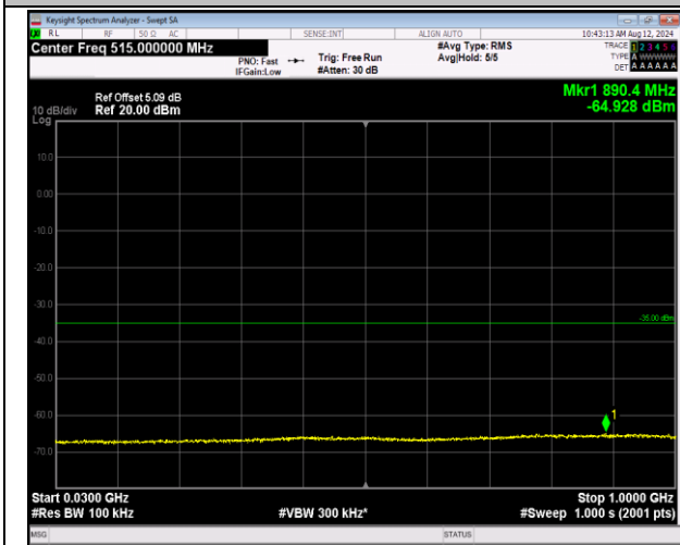
7-7-10MHz-20MHz-QPSK-QPSK-21006-21150-1RB#49-0 RB#0-30~1000MHz-PASS
