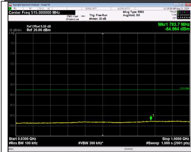
7-7-20MHz-10MHz-16QAM-16QAM-21051-21195-1RB#0 -ORB#0-30~1000MHz-PASS
