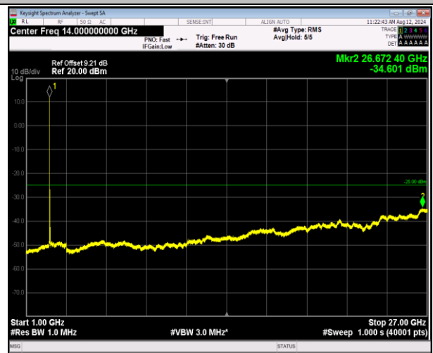
7-7-20MHz-10MHz-16QAM-16QAM-21051-21195-1RB#0-1 RB#49-1000~27000MHz-PASS
