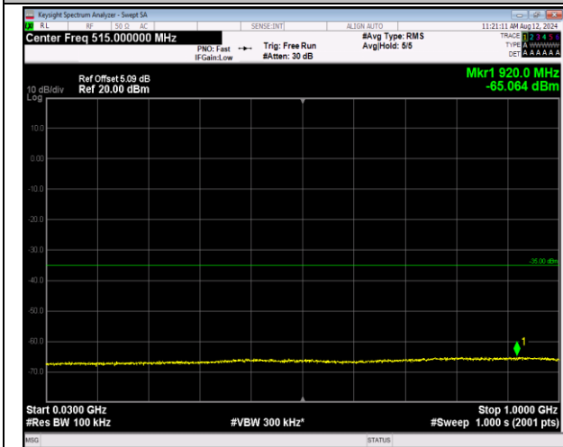
7-7-20MHz-10MHz-16QAM-16QAM-21051-21195-1RB#9 9-ORB#0-30~1000MHz-PASS
