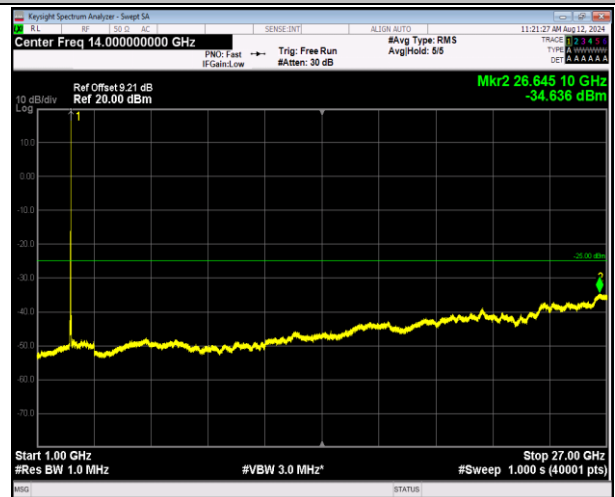
7-7-20MHz-10MHz-16QAM-16QAM-21051-21195-1RB#99- ORB#0-1000~27000MHz-PASS
