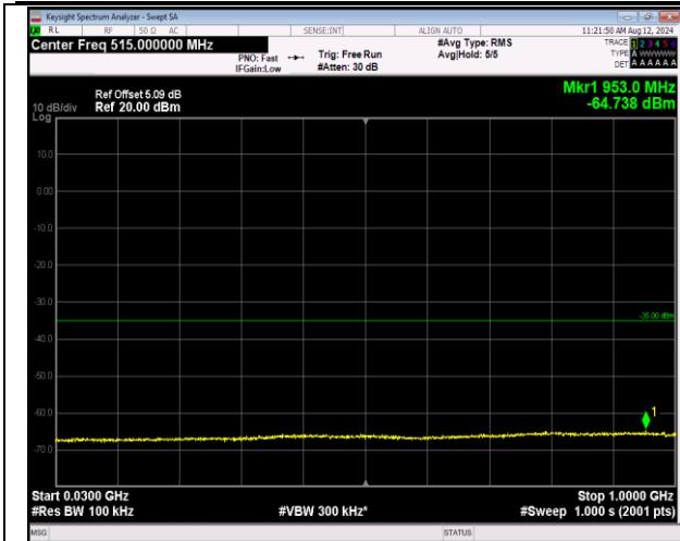
7-7-20MHz-10MHz-QPSK-QPSK-21051-21195-1RB#0-1 RB#49-30~1000MHz-PASS
