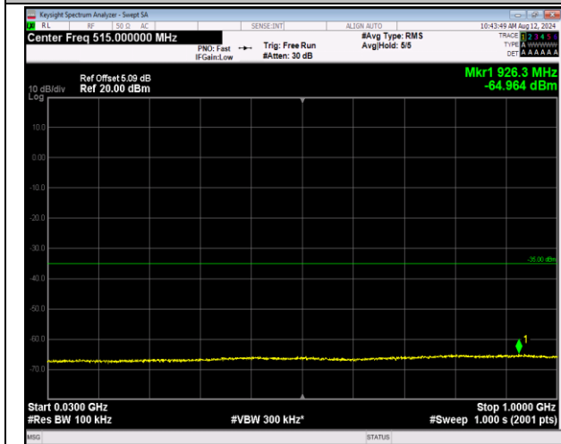
7-7-10MHz-20MHz-16QAM-16QAM-21006-21150-1RB#49-9-ORB#0-30~1000MHz-PASS
