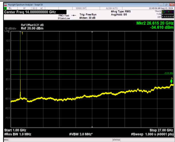
7-7-10MHz-20MHz-16QAM-16QAM-21206-21350-1RB#49- ORB#0-1000~27000MHz-PASS
