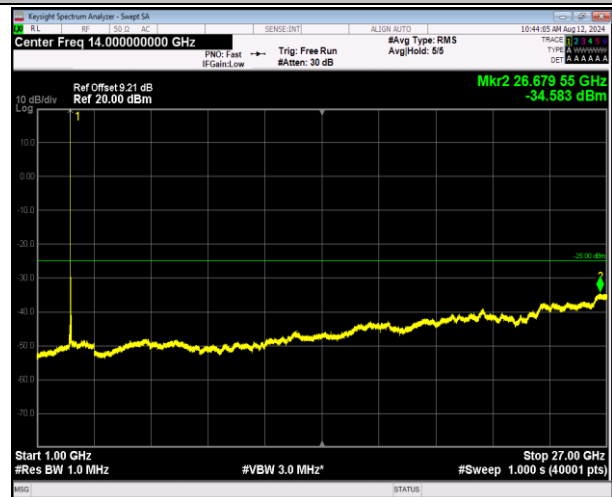
7-7-10MHz-20MHz-16QAM-16QAM-21006-21150-1RB#49-ORB#0-1000~27000MHz-PASS
