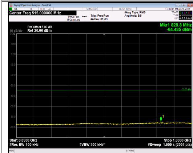
7-7-20MHz-10MHz-64QAM-64QAM-20850-20994-1RB#0 -1RB#49-30~1000MHz-PASS
