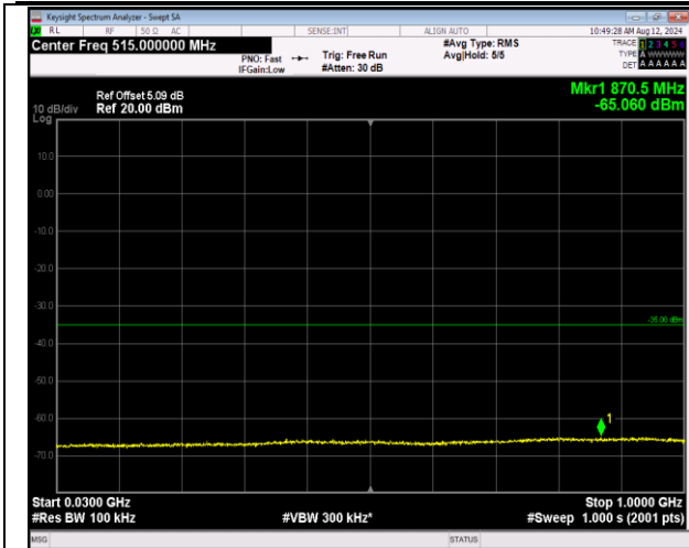
7-7-10MHz-20MHz-QPSK-QPSK-21206-21350-1RB#0-1 RB#99-30~1000MHz-PASS
