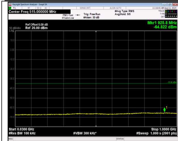
7-7-20MHz-10MHz-QPSK-QPSK-20850-20994-1RB#0-1 RB#49-30~1000MHz-PASS
