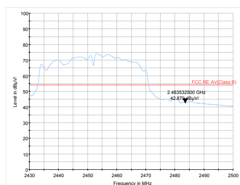
802.11n HT40 -Channel 9 Average
