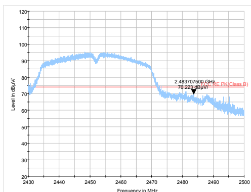
802.11n HT40 -Channel 9 Peak
