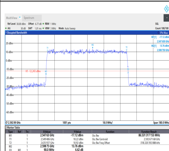
1-N41--30-90-M-3-DFT-16QAM-Outer_Full-2 43@0-Ant1-86.531-90.000-≤90-PASS
