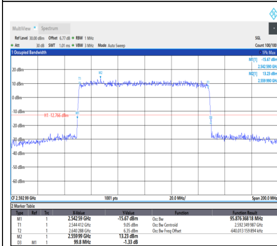
1-N41--30-100-M-3-DFT-16QAM-Outter_Full-270@0-Ant1-95.876-99.800-≤100-PASS
