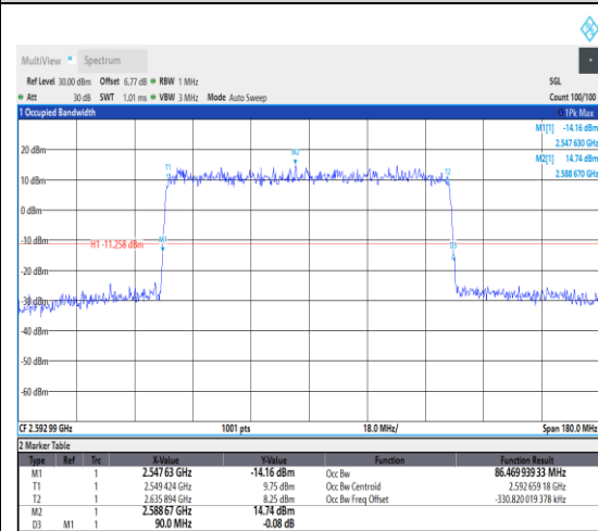
1-N41--30-90-M-1-DFT-QPSK-Outer_Full-24 3@0-Ant1-86.47-90.000-≤90-PASS
