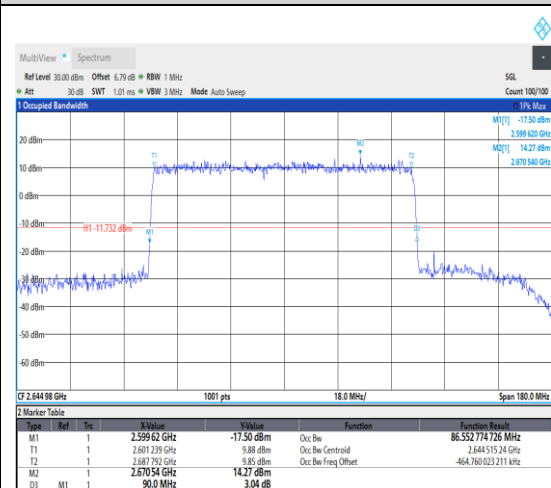
1-N41--30-90-H-4-DFT-64QAM-Outer_Full-2 43@0-Ant1-86.553-90.000-≤90-PASS
