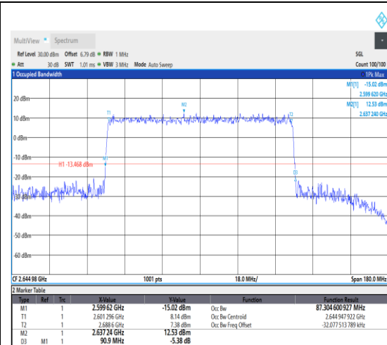
1-N41--30-90-H-8-CP-64QAM-Outer_Full-24 5@0-Ant1-87.305-90.900-≤90-PASS
