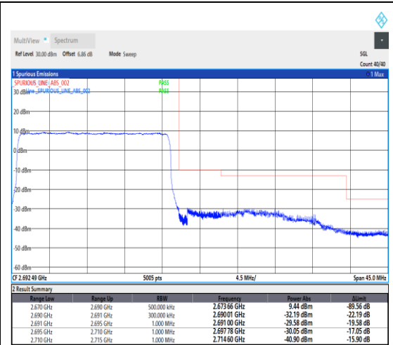
1-N41--30-20-H-3-DFT-PI2BPSK-Outer_Full-50@0-Ant1-1--PASS-see graph
