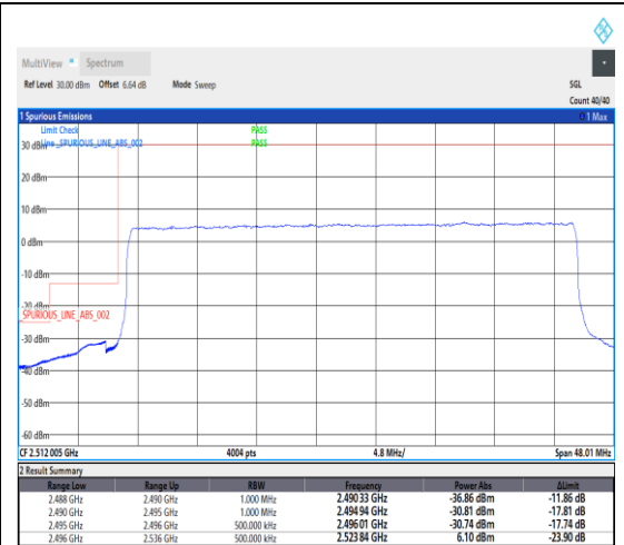
1-N41--30-40-L-3-DFT-PI2BPSK-Outer_Full- 100@0-Ant1-1--PASS-see graph
