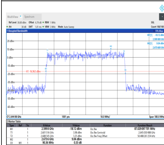
1-N41--30-90-H-9-CP-256QAM-Outer_Full-2 45@0-Ant1-87.029-90.360-≤90-PASS
