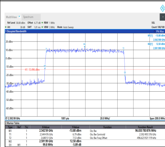
1-N41--30-100-M-4-DFT-64QAM-Outter_Full-270@0-Ant1-96.034-99.800-≤100-PASS
