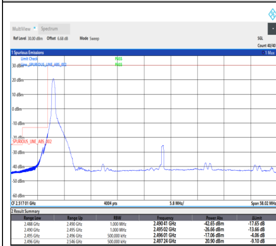
1-N41--30-50-L-4-CP-QPSK-Edge_1RB_Left -1@0-Ant1-1--PASS-see graph
