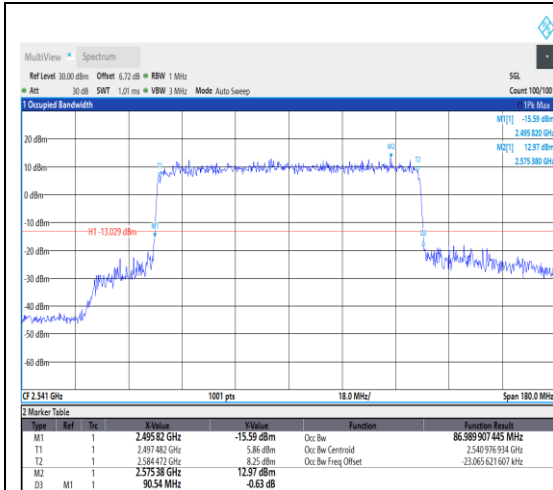
1-N41--30-90-L-7-CP-16QAM-Outer_Full-245 @0-Ant1-86.99-90.540-≤90-PASS
