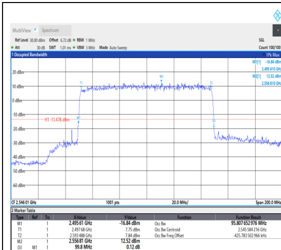
1-N41--30-100-L-4-DFT-64QAM-Outer_Full-270@0-Ant1-95.808-99.800≤100-PASS
