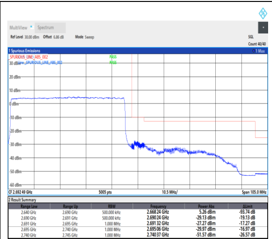
1-N41--30-50-H-3-DFT-PI2BPSK-Outer_Full-128@0-Ant1-1--PASS-see graph
