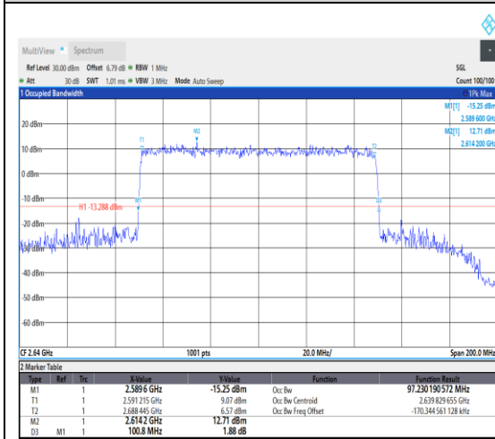
1-N41--30-100-H-6-CP-QPSK-Outer_Full-273@0-Ant1-97.23-100.800-≤100-PASS
