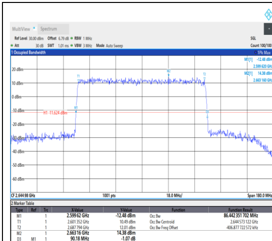
1-N41--30-90-H-1-DFT-QPSK-Outer_Full-24 3@0-Ant1-86.442-90.180-≤90-PASS
