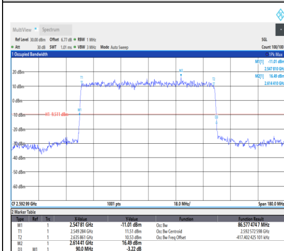
1-N41--30-90-M-2-DFT-PI2BPSK-Outer_Full- 243@0-Ant1-86.577-90.000-≤90-PASS
