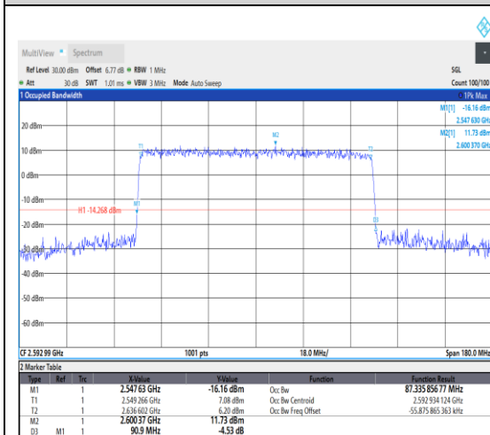
1-N41--30-90-M-8-CP-64QAM-Outer_Full-24 5@0-Ant1-87.336-90.900-≤90-PASS
