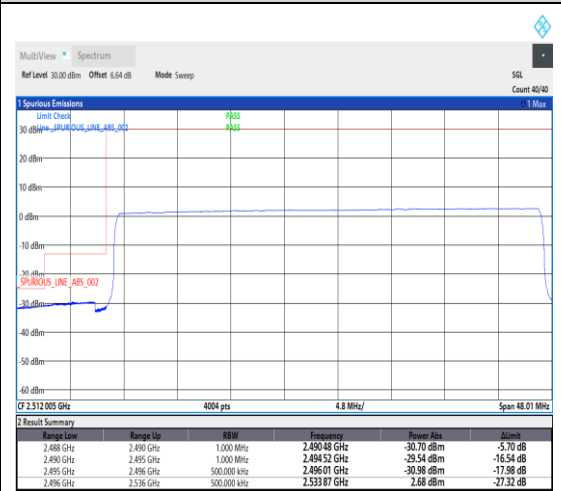
1-N41--30-40-L-6-CP-QPSK-Outer_Full-106 @0-Ant1-1--PASS-see graph
