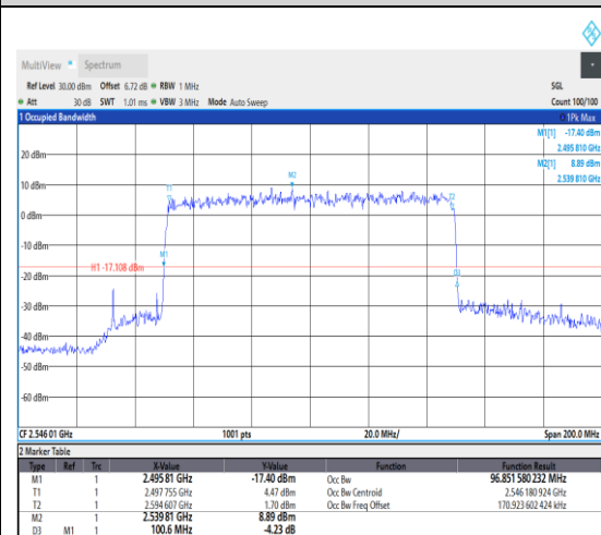
1-N41--30-100-L-9-CP-256QAM-Outer_Full-273@0-Ant1-96.852-100.600≤100-PASS
