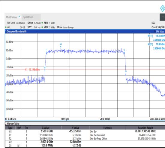
1-N41--30-100-H-7-CP-16QAM-Outer_Full-273@0-Ant1-96.861-100.800-≤100-PASS
