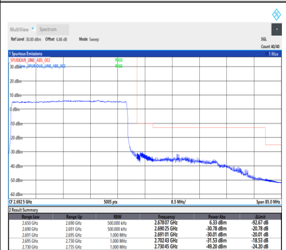
1-N41--30-40-H-3-DFT-PI2BPSK-Outer_Full- 100@0-Ant1-1--PASS-see graph
