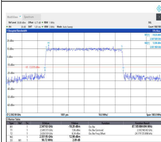
1-N41--30-90-M-6-CP-QPSK-Outer_Full-245 @0-Ant1-87.186-90.720-≤90-PASS
