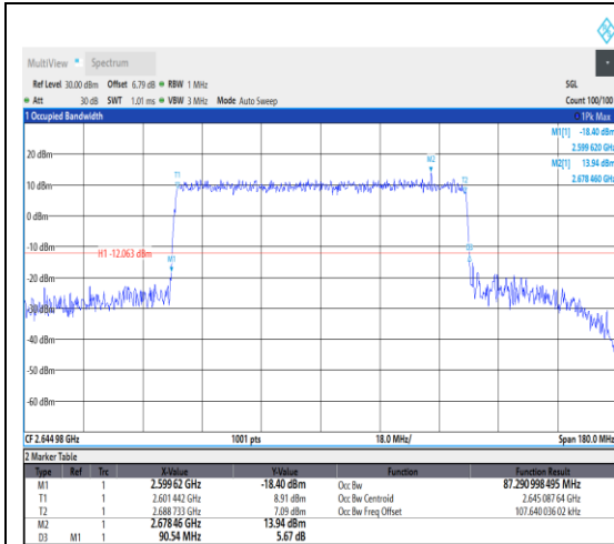
1-N41--30-90-H-7-CP-16QAM-Outer_Full-24 5@0-Ant1-87.291-90.540-≤90-PASS
