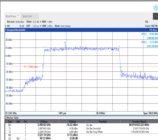
1-N41--30-90-L-8-CP-64QAM-Outer_Full-245 @0-Ant1-86.917-90.720-≤90-PASS
