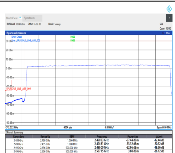
1-N41--30-60-L-3-DFT-PI2BPSK-Outer_Full-162@0-Ant1-1--PASS-see graph
