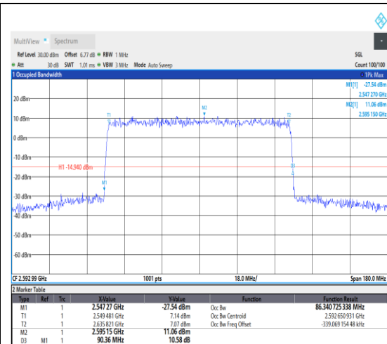
1-N41--30-90-M-5-DFT-256QAM-Outer_Full- 243@0-Ant1-86.341-90.360-≤90-PASS
