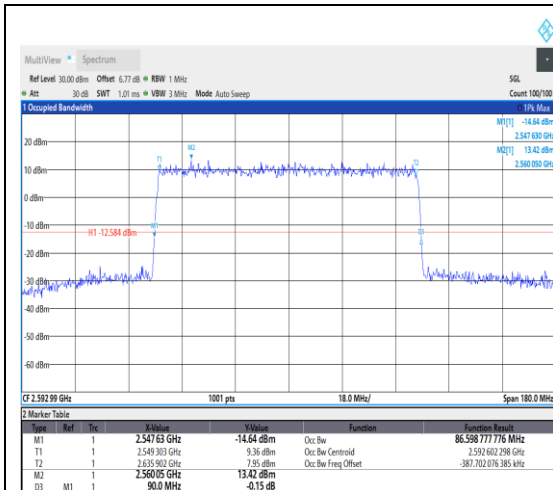
1-N41--30-90-M-4-DFT-64QAM-Outer_Full-2 43@0-Ant1-86.599-90.000-≤90-PASS
