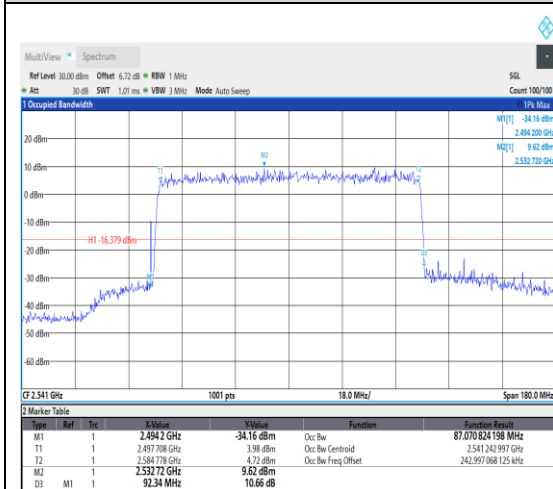
1-N41--30-90-L-9-CP-256QAM-Outer_Full-24 5@0-Ant1-87.071-92.340-≤90-PASS
