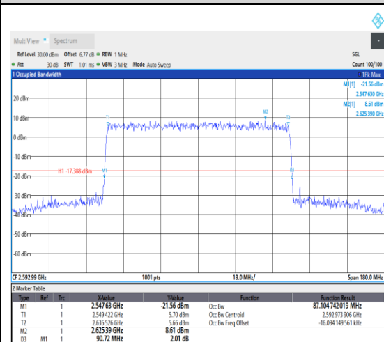
1-N41--30-90-M-9-CP-256QAM-Outer_Full-2 45@0-Ant1-87.105-90.720-≤90-PASS
