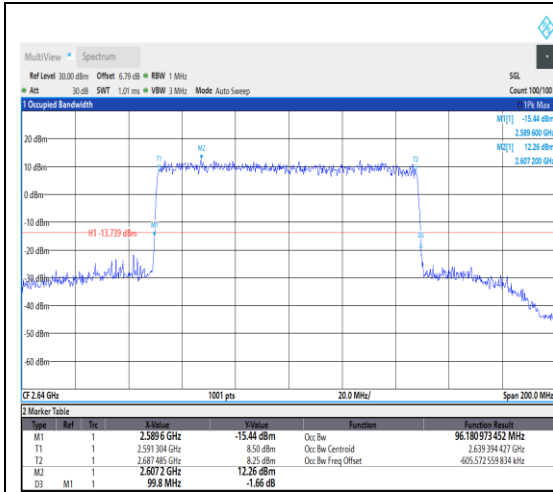
1-N41--30-100-H-4-DFT-64QAM-Outer_Full-270@0-Ant1-96.181-99.800-≤100-PASS
