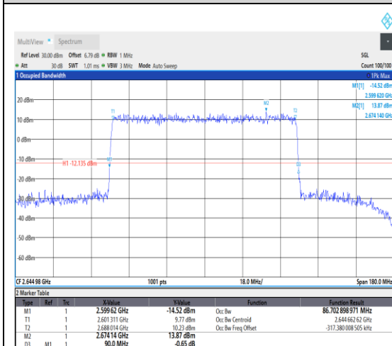
1-N41--30-90-H-3-DFT-16QAM-Outer_Full-2 43@0-Ant1-86.703-90.000-≤90-PASS
