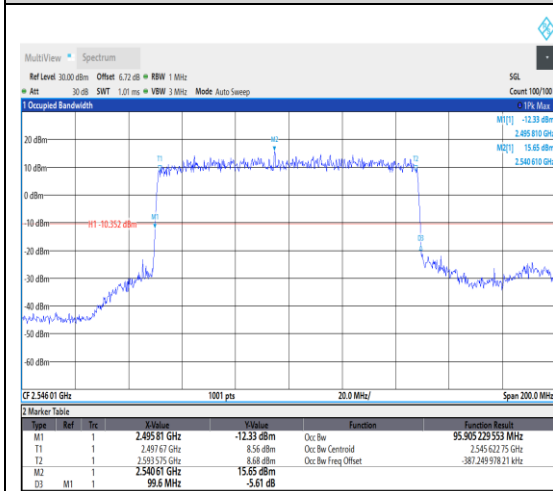
1-N41--30-100-L-2-DFT-PI2BPSK-Outer_Full -270@0-Ant1-95.905-99.600-≤100-PASS
