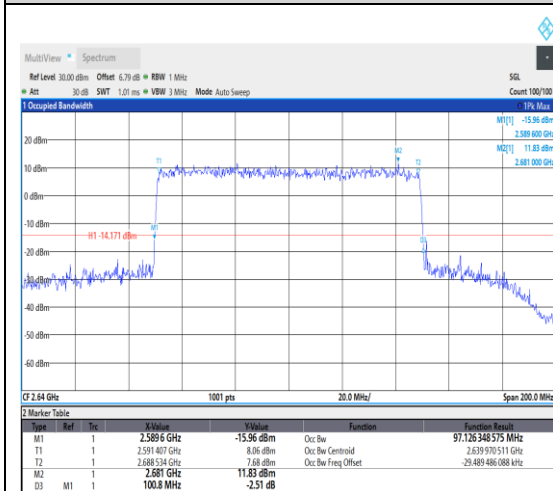
1-N41--30-100-H-8-CP-64QAM-Outer_Full-273@0-Ant1-97.126-100.800-≤100-PASS
