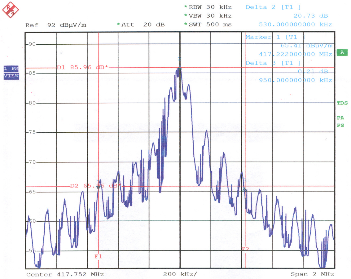
<Plot of occupied bandwidth >
