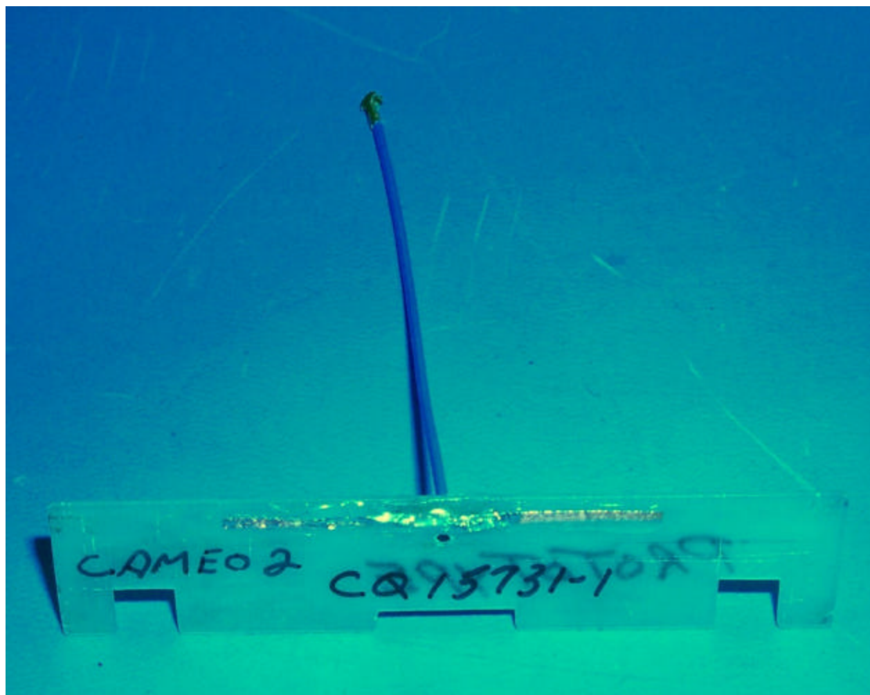
CQ15731 antenna for the Cameo 2 printer
