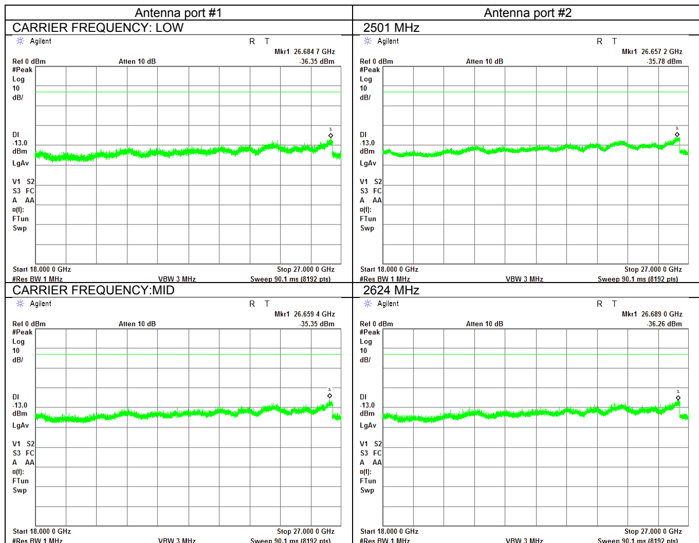
Plot 7.4.11 Spurious emission measurements in 18000 - 27000 MHz range
