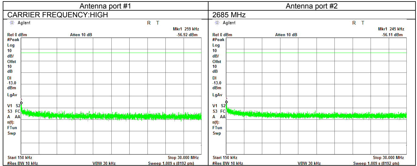
Plot 7.4.4 Spurious emission measurements in 0.15 - 30 MHz range
