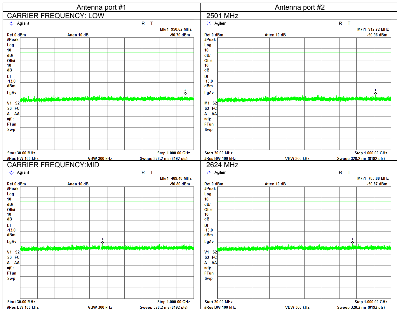
Plot 7.4.5 Spurious emission measurements in 30 - 1000 MHz range
