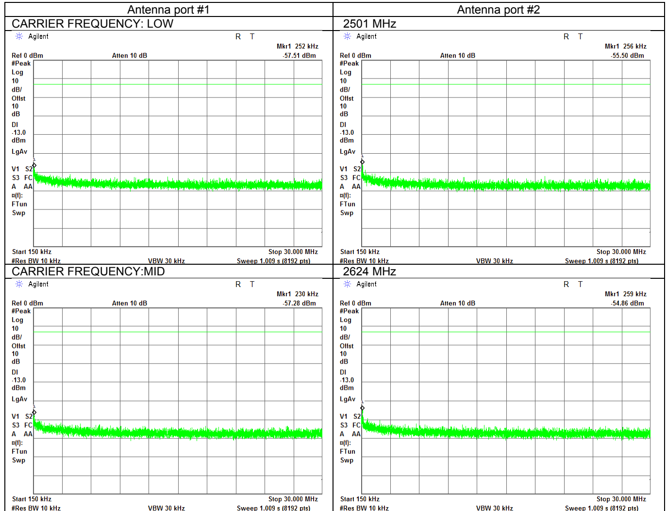
Plot 7.4.3 Spurious emission measurements in 0.15 - 30 MHz range
