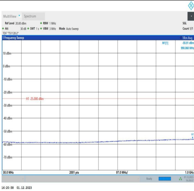
7-7-15MHz-15MHz-16QAM-16QAM-21225-21375-75RB#0-75 RB#0-30~1000MHz-PASS
