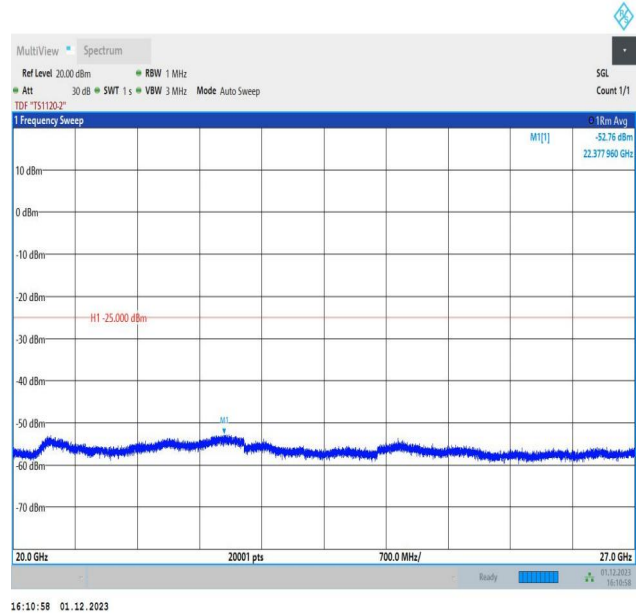
7-7-15MHz-15MHz-16QAM-16QAM-21025-21175-1RB#0-1RB #74-20000~27000MHz-PASS
