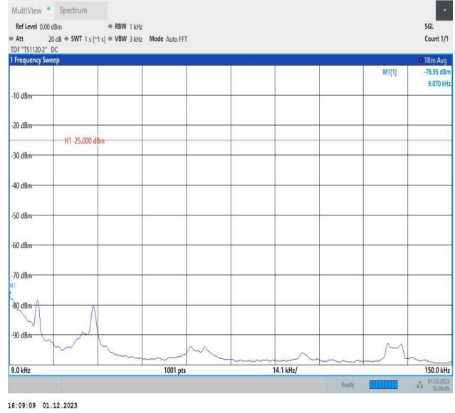
7-7-15MHz-15MHz-64QAM-64QAM-21025-21175-1RB#74-0R B#0-0.009~0.15MHz-PASS
