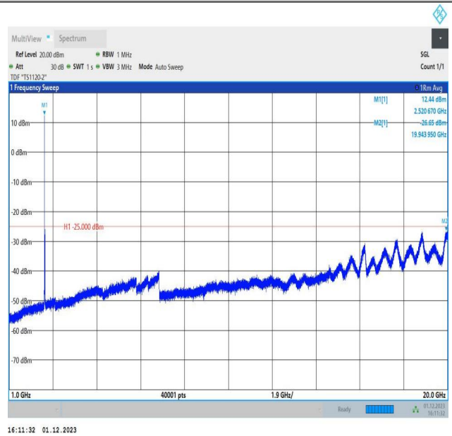
7-7-15MHz-15MHz-64QAM-64QAM-21025-21175-1RB#0-1RB #74-1000~20000MHz-PASS
