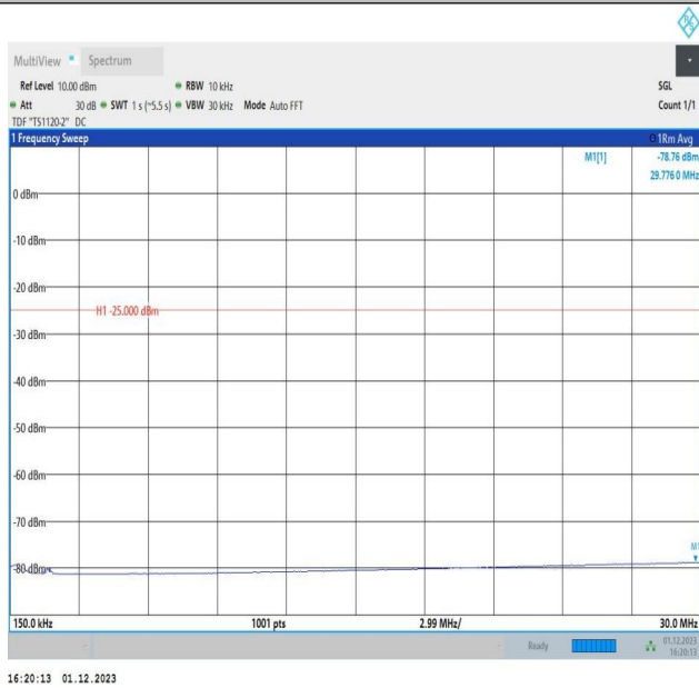
7-7-15MHz-15MHz-QPSK-QPSK-21225-21375-75RB#0-75RB #0-0.15~30MHz-PASS
