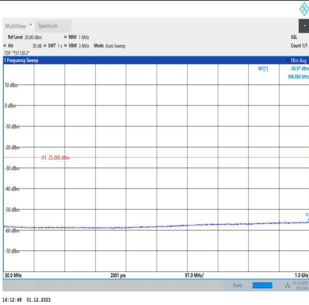
7-7-15MHz-15MHz-16QAM-16QAM-21025-21175-75RB#0-75 RB#0-30~1000MHz-PASS
