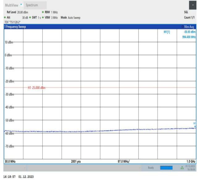
7-7-15MHz-15MHz-16QAM-16QAM-21225-21375-1RB#0-1RB #74-30~1000MHz-PASS
