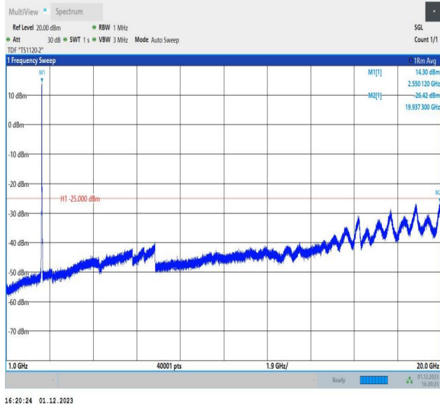
7-7-15MHz-15MHz-QPSK-QPSK-21225-21375-75RB#0-75RB #0-1000~20000MHz-PASS
