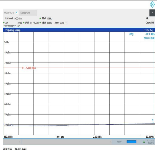
7-7-15MHz-15MHz-16QAM-16QAM-21225-21375-75RB#0-75 RB#0-0.15~30MHz-PASS
