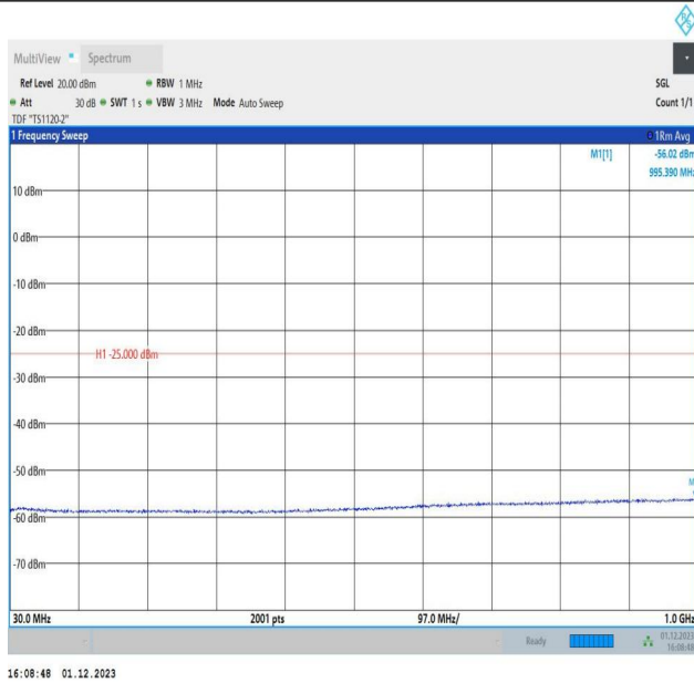
7-7-15MHz-15MHz-16QAM-16QAM-21025-21175-1RB#74-0R B#0-30~1000MHz-PASS
