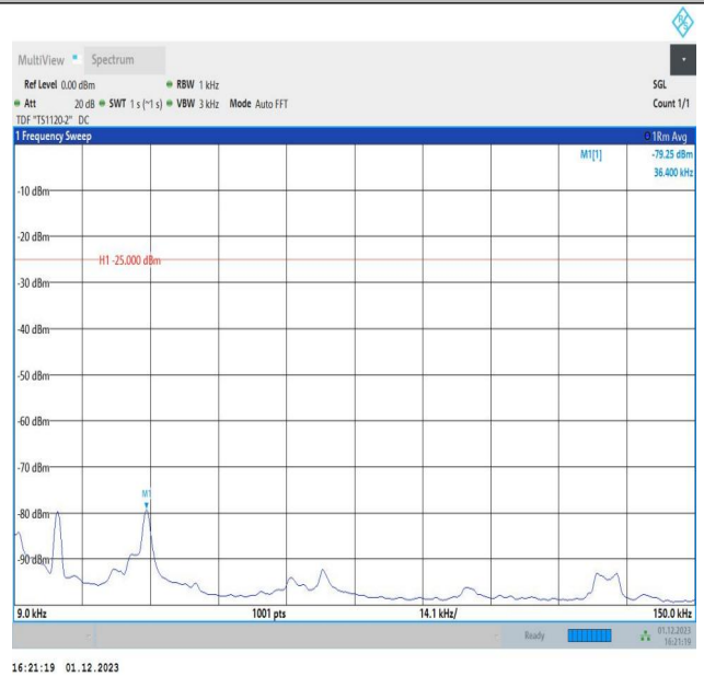
7-7-15MHz-15MHz-64QAM-64QAM-21225-21375-75RB#0-75 RB#0-0.009~0.15MHz-PASS
