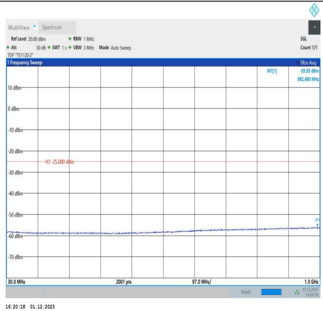
7-7-15MHz-15MHz-QPSK-QPSK-21225-21375-75RB#0-75RB #0-30~1000MHz-PASS
