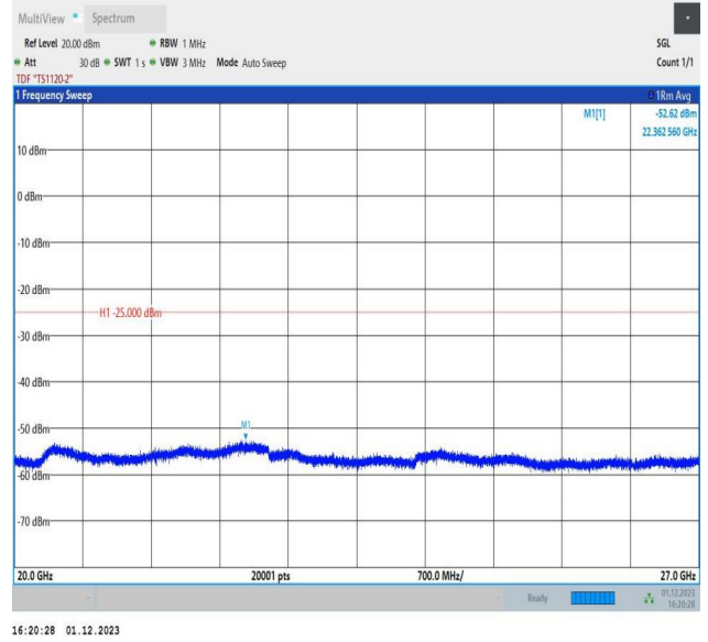
7-7-15MHz-15MHz-QPSK-QPSK-21225-21375-75RB#0-75RB #0-20000~27000MHz-PASS
