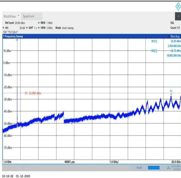
7-7-15MHz-15MHz-QPSK-QPSK-21225-21375-1RB#74-0RB# 0-1000~20000MHz-PASS
