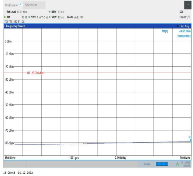
7-7-15MHz-15MHz-16QAM-16QAM-21025-21175-1RB#74-0R B#0-0.15~30MHz-PASS
