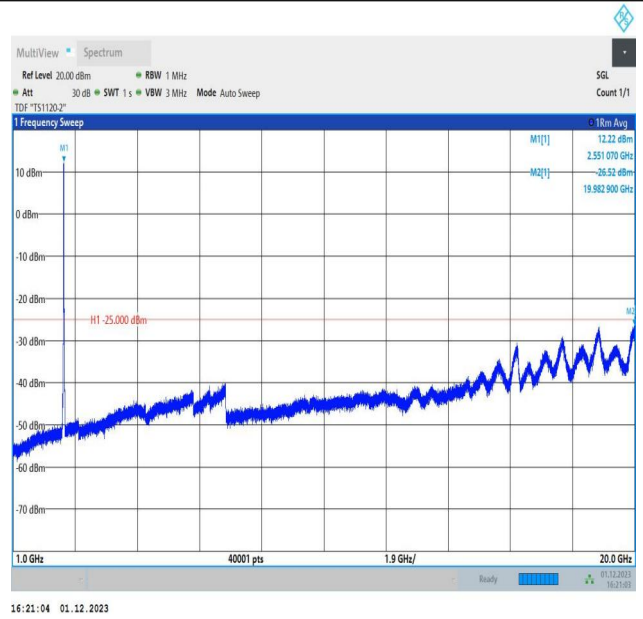
7-7-15MHz-15MHz-16QAM-16QAM-21225-21375-75RB#0-75 RB#0-1000~20000MHz-PASS
