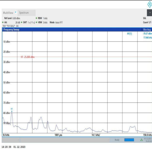
7-7-15MHz-15MHz-16QAM-16QAM-21225-21375-75RB#0-75 RB#0-0.009~0.15MHz-PASS
