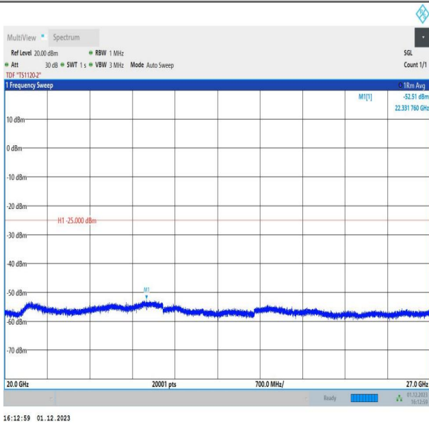
7-7-15MHz-15MHz-16QAM-16QAM-21025-21175-75RB#0-75 RB#0-20000~27000MHz-PASS
