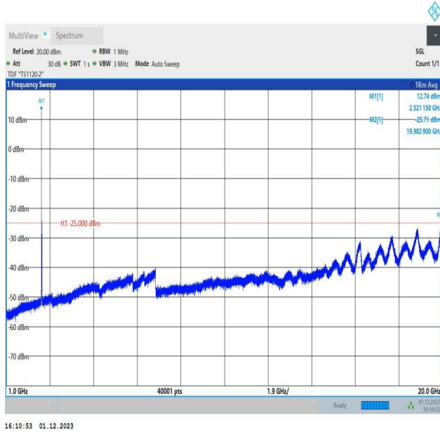
7-7-15MHz-15MHz-16QAM-16QAM-21025-21175-1RB#0-1RB #74-1000~20000MHz-PASS
