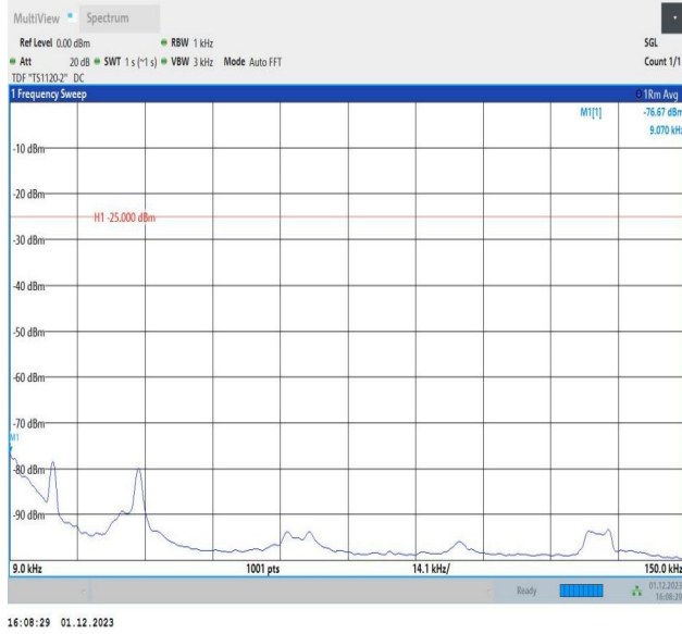
7-7-15MHz-15MHz-16QAM-16QAM-21025-21175-1RB#74-0R B#0-0.009~0.15MHz-PASS
