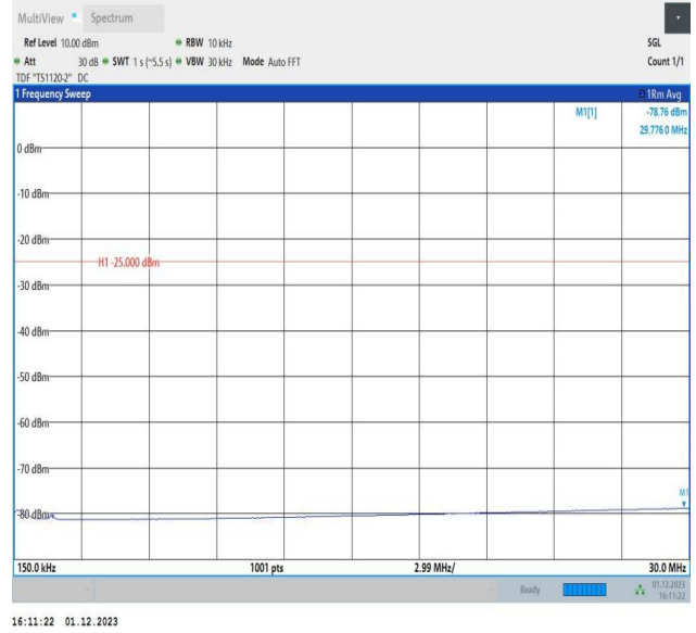
7-7-15MHz-15MHz-64QAM-64QAM-21025-21175-1RB#0-1RB #74-0.15~30MHz-PASS
