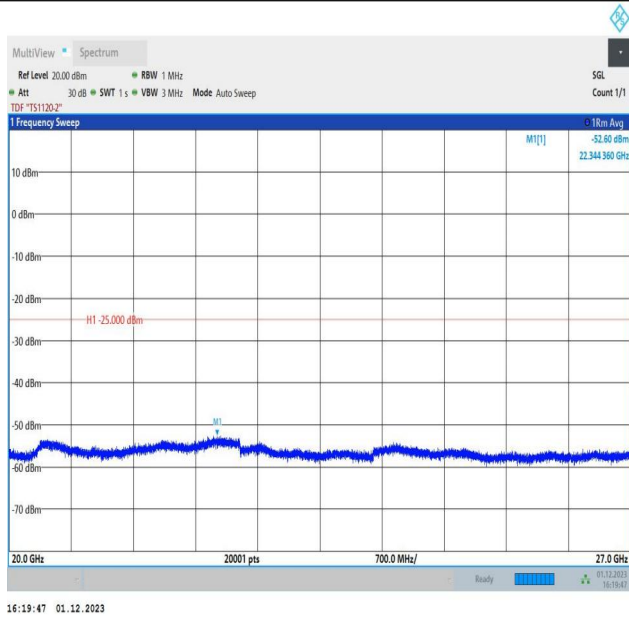
7-7-15MHz-15MHz-64QAM-64QAM-21225-21375-1RB#0-1RB #74-20000~27000MHz-PASS
