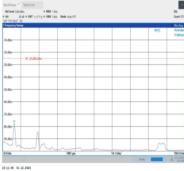
7-7-15MHz-15MHz-64QAM-64QAM-21025-21175-1RB#0-1RB #74-0.009~0.15MHz-PASS
