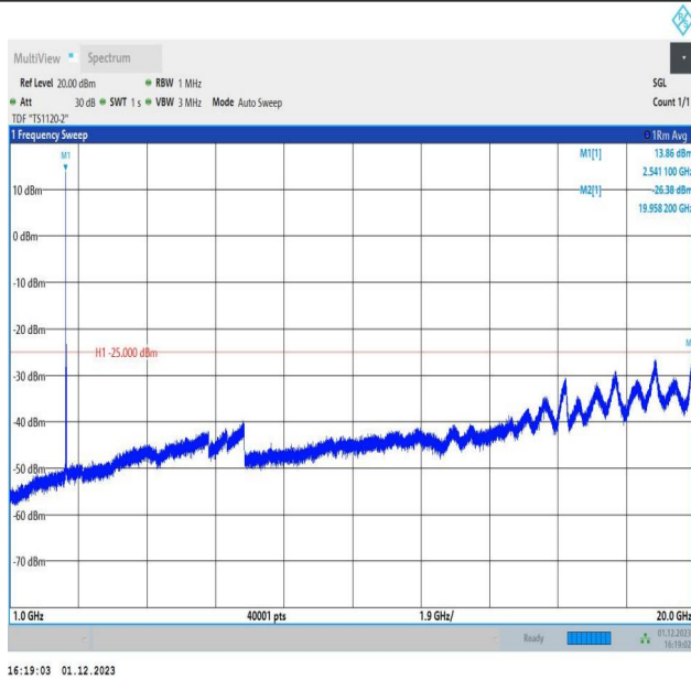
7-7-15MHz-15MHz-16QAM-16QAM-21225-21375-1RB#0-1RB #74-1000~20000MHz-PASS
