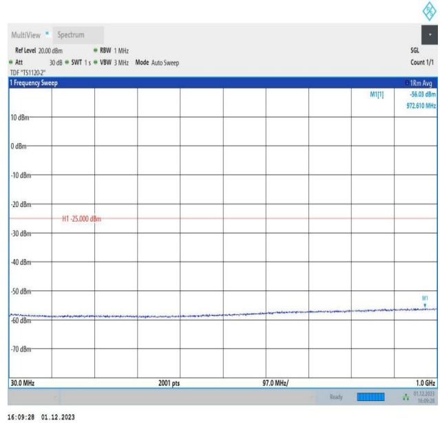
7-7-15MHz-15MHz-64QAM-64QAM-21025-21175-1RB#74-0R B#0-30~1000MHz-PASS
