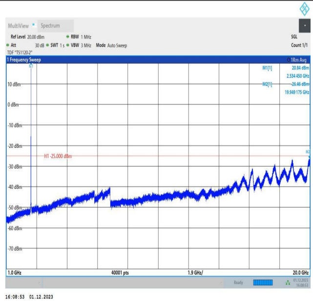
7-7-15MHz-15MHz-16QAM-16QAM-21025-21175-1RB#74-0R B#0-1000~20000MHz-PASS
