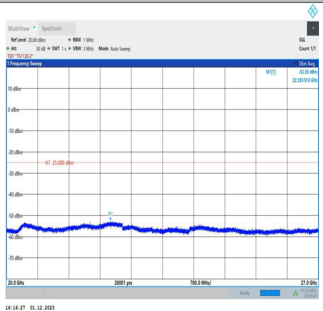
7-7-15MHz-15MHz-QPSK-QPSK-21225-21375-1RB#74-0RB# 0-20000~27000MHz-PASS
