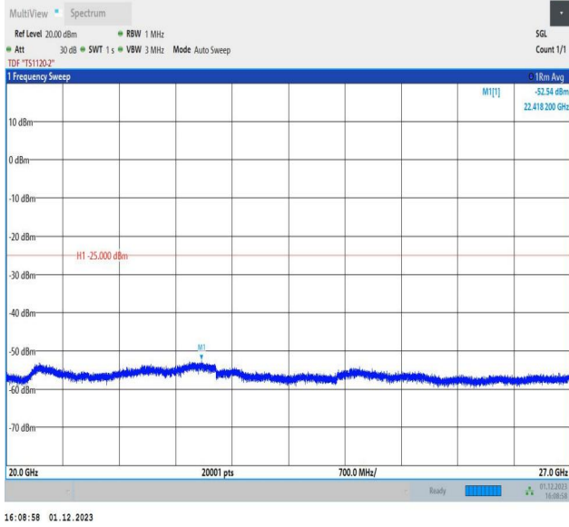
7-7-15MHz-15MHz-16QAM-16QAM-21025-21175-1RB#74-0R B#0-20000~27000MHz-PASS
