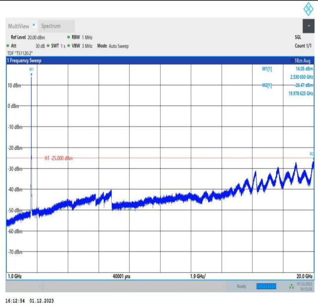
7-7-15MHz-15MHz-16QAM-16QAM-21025-21175-75RB#0-75 RB#0-1000~20000MHz-PASS
