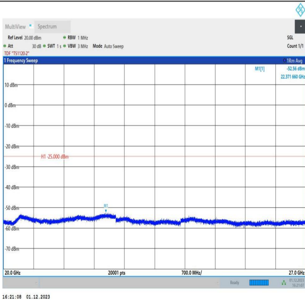
7-7-15MHz-15MHz-16QAM-16QAM-21225-21375-75RB#0-75 RB#0-20000~27000MHz-PASS
