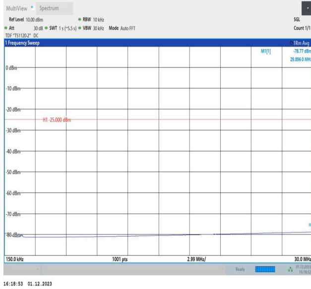
7-7-15MHz-15MHz-16QAM-16QAM-21225-21375-1RB#0-1RB #74-0.15~30MHz-PASS
