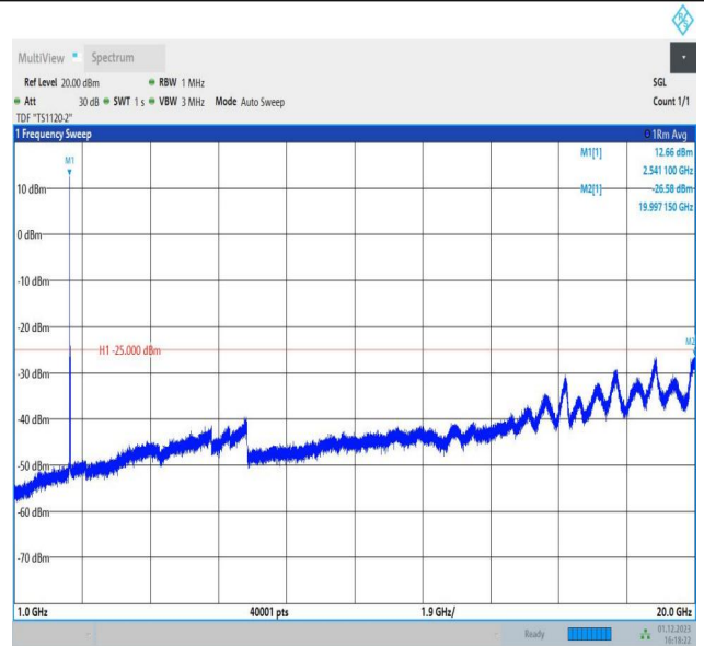
7-7-15MHz-15MHz-QPSK-QPSK-21225-21375-1RB#0-1RB#7 4-1000~20000MHz-PASS
