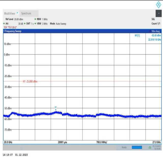
7-7-15MHz-15MHz-16QAM-16QAM-21225-21375-1RB#0-1RB #74-20000~27000MHz-PASS
