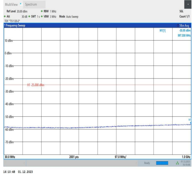
7-7-15MHz-15MHz-16QAM-16QAM-21025-21175-1RB#0-1RB #74-30~1000MHz-PASS
