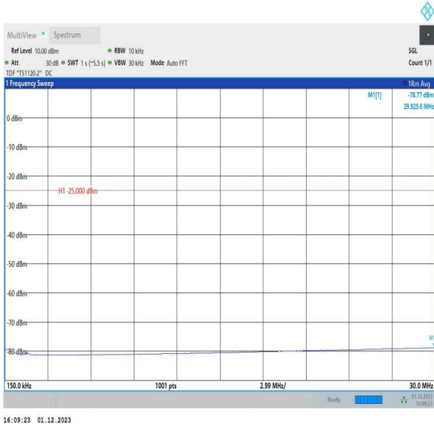
7-7-15MHz-15MHz-64QAM-64QAM-21025-21175-1RB#74-0R B#0-0.15~30MHz-PASS
