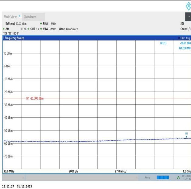
7-7-15MHz-15MHz-64QAM-64QAM-21025-21175-1RB#0-1RB #74-30~1000MHz-PASS
