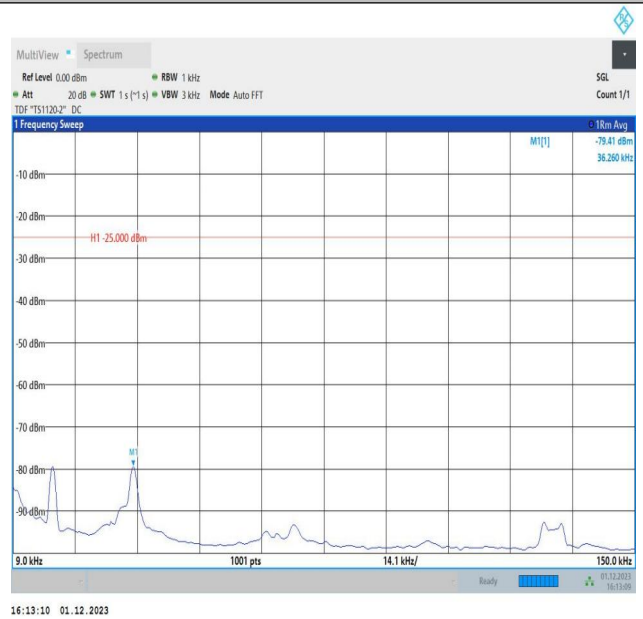
7-7-15MHz-15MHz-64QAM-64QAM-21025-21175-75RB#0-75 RB#0-0.009~0.15MHz-PASS
