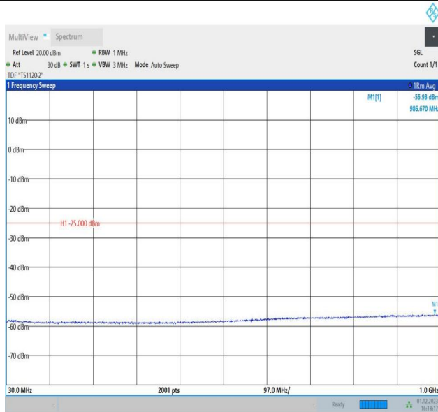
7-7-15MHz-15MHz-QPSK-QPSK-21225-21375-1RB#0-1RB#7 4-30~1000MHz-PASS
