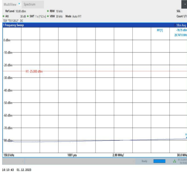
7-7-15MHz-15MHz-16QAM-16QAM-21025-21175-1RB#0-1RB #74-0.15~30MHz-PASS
