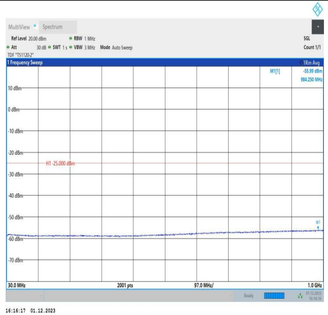
7-7-15MHz-15MHz-QPSK-QPSK-21225-21375-1RB#74-0RB# 0-30~1000MHz-PASS
