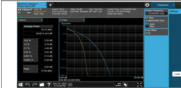
Band4-20MHz-QPSK-20175-100RB#0-PASS
