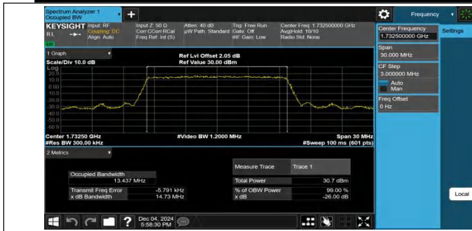
Band4-15MHz-QPSK-20175-75RB#0-PASS
