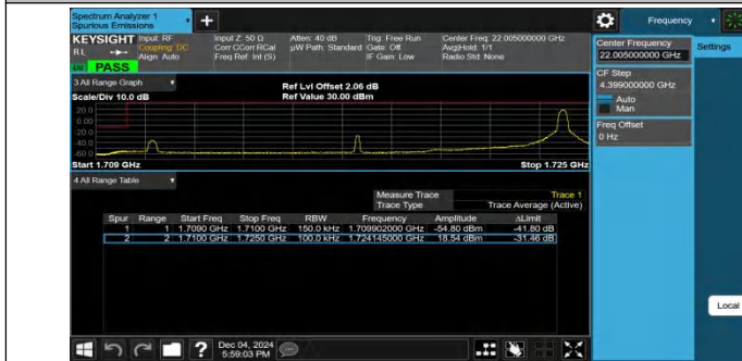
Band4-15MHz-QPSK-20025-1RB#74-PASS
