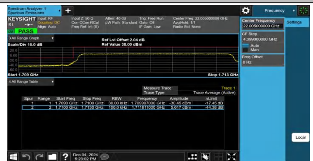
Band4-3MHz-QPSK-19965-15RB#0-PASS
