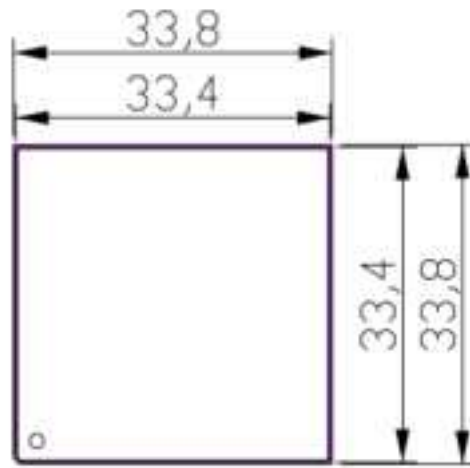
Figure 5-1 Top View
