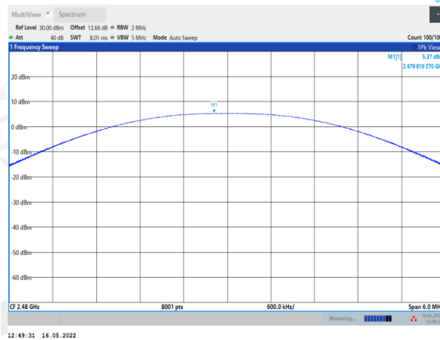
BLE_1M_Ant1_2480
