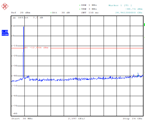
Conducted spurious emission: GFSK, Ch78, 30MHz~26GHz
