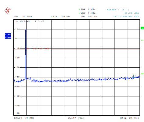
Conducted spurious emission: \pi/4 DQPSK, Ch78, 30MHz~26GHz
