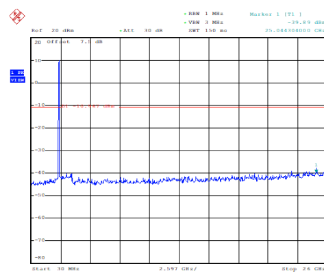
Conducted spurious emission: \pi/4 DQPSK, Ch0, 30MHz~26GHz
