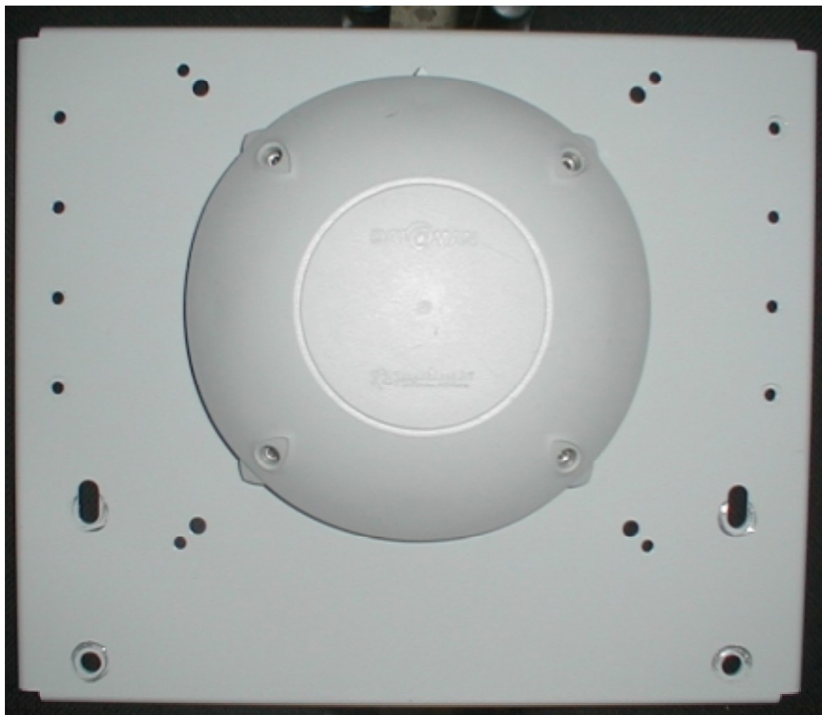
RSC auxiliary antenna front view
