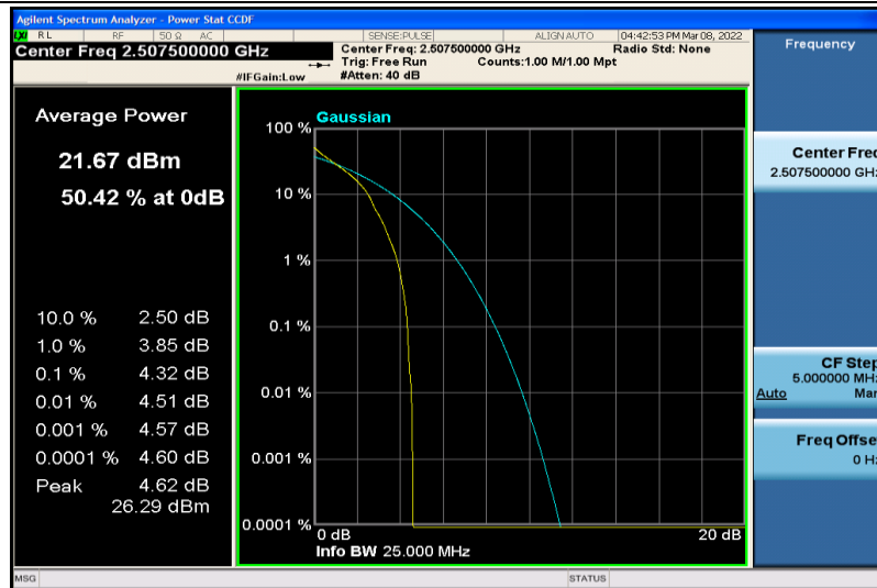
Band7-15MHz-64QAM-20825-1RB#0
