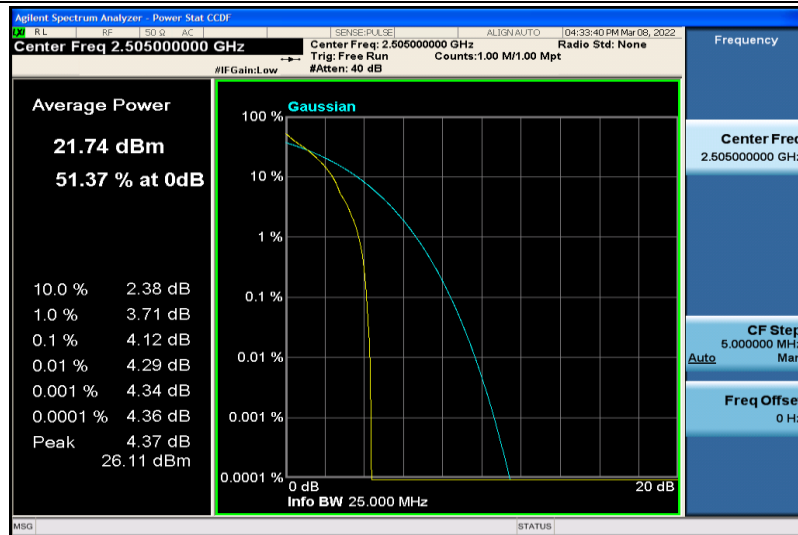
Band7-10MHz-64QAM-20800-1RB#0
