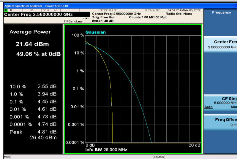
Band7-20MHz-64QAM-21350-1RB#0
