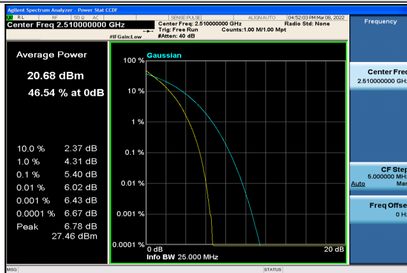
Band7-20MHz-64QAM-20850-100RB#0
