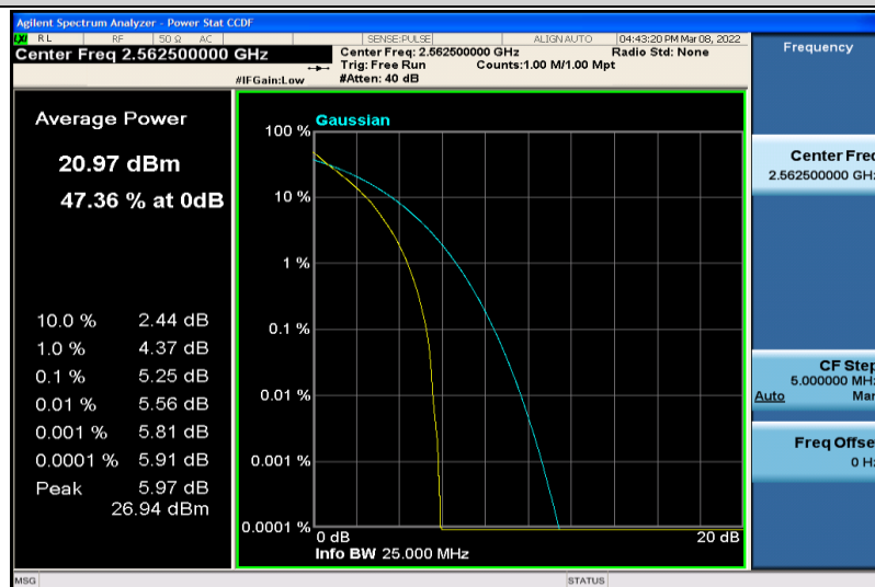
Band7-15MHz-64QAM-21375-75RB#0
