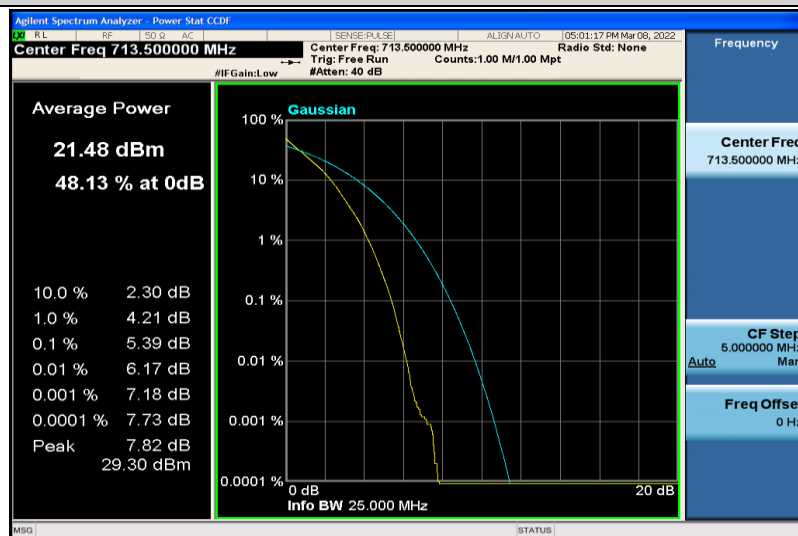
Band17-5MHz-64QAM-23825-25RB#0
