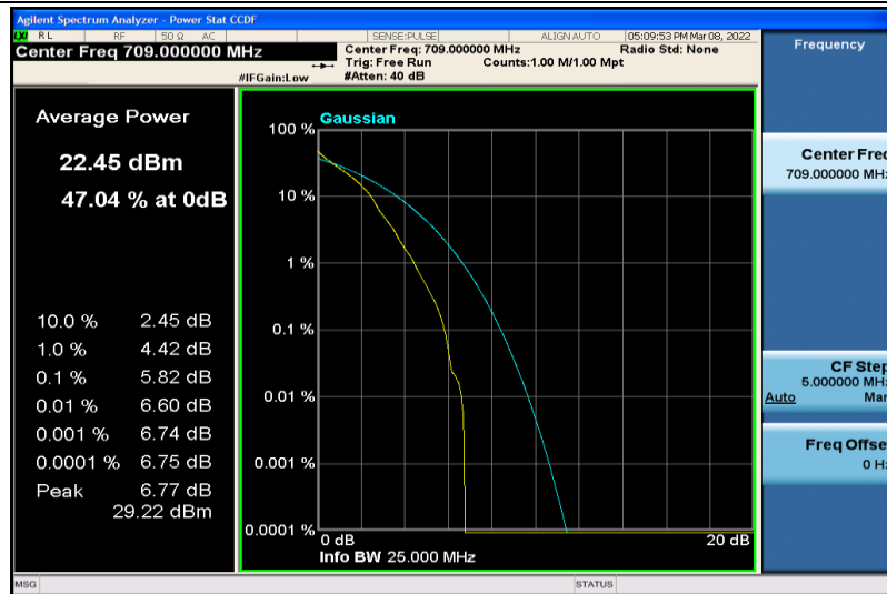
Band17-10MHz-64QAM-23780-1RB#0
