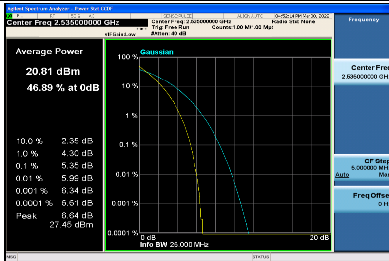
Band7-20MHz-64QAM-21100-100RB#0
