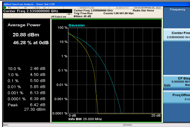
Band7-15MHz-64QAM-21100-75RB#0
