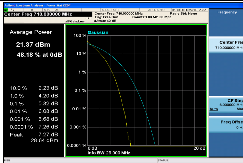
Band17-10MHz-64QAM-23790-50RB#0
