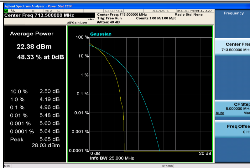
Band17-5MHz-64QAM-23825-1RB#0
