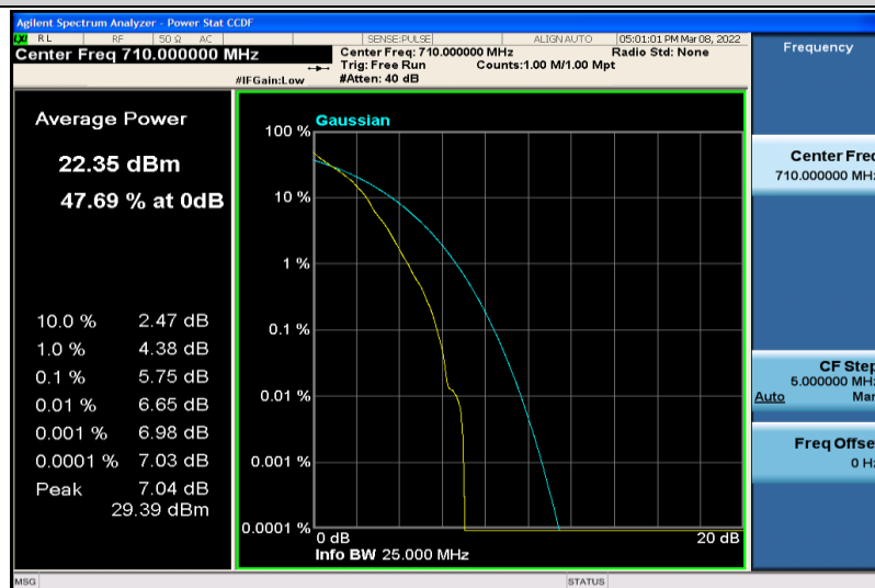
Band17-5MHz-64QAM-23790-1RB#0
