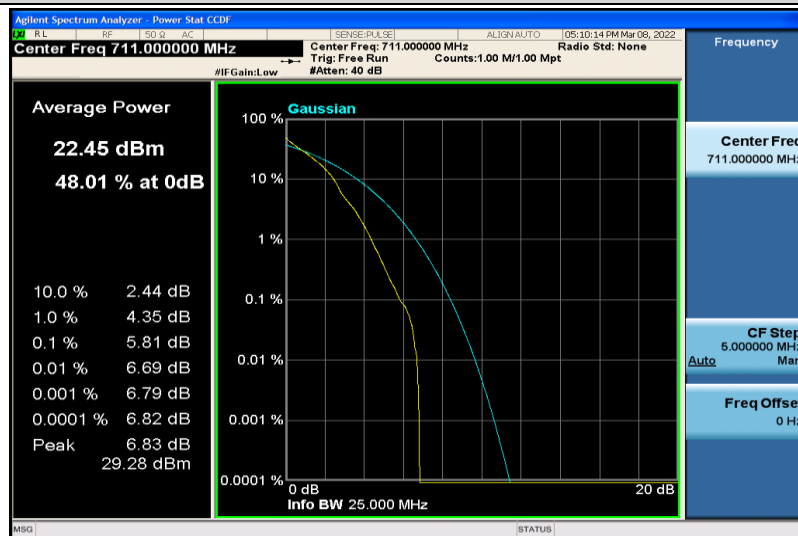
Band17-10MHz-64QAM-23800-1RB#0
