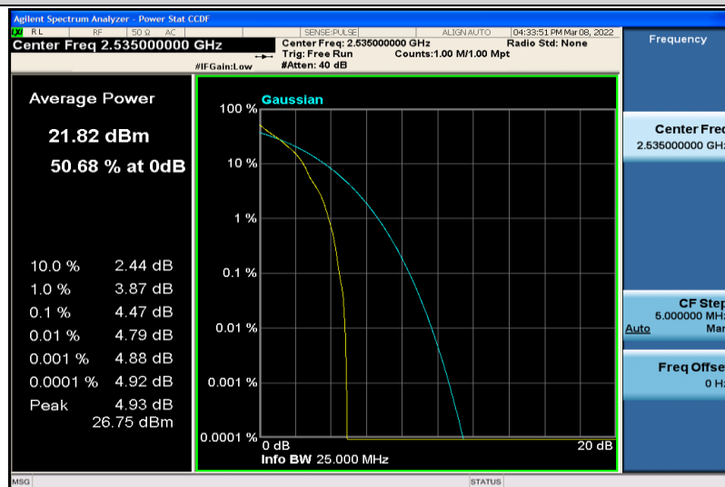
Band7-10MHz-64QAM-21100-1RB#0
