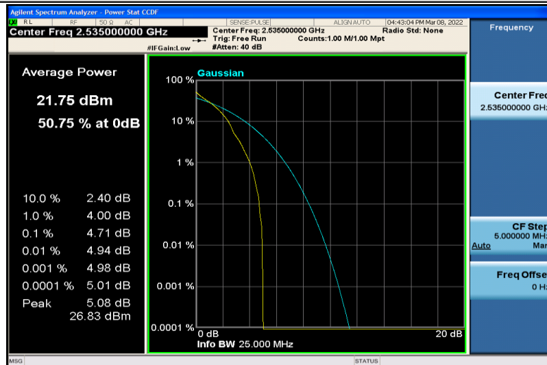
Band7-15MHz-64QAM-21100-1RB#0
