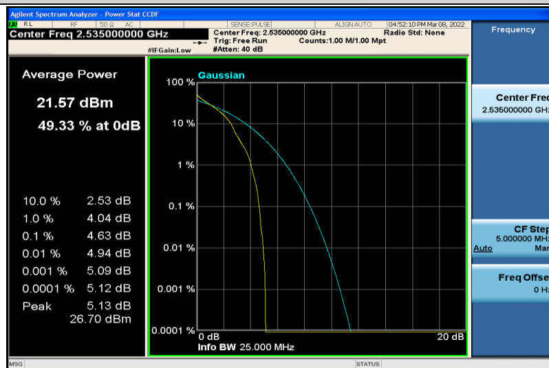
Band7-20MHz-64QAM-21100-1RB#0
