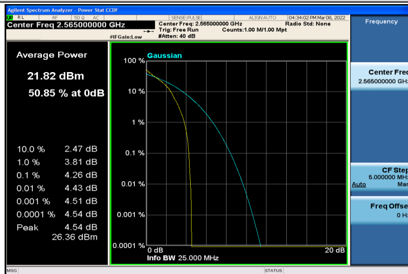
Band7-10MHz-64QAM-21400-1RB#0
