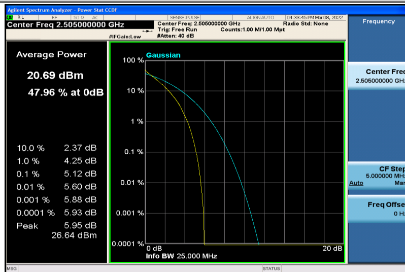
Band7-10MHz-64QAM-20800-50RB#0
