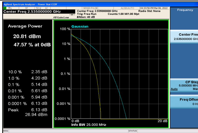
Band7-10MHz-64QAM-21100-50RB#0
