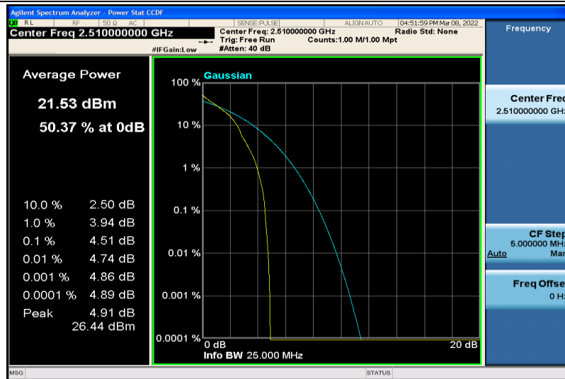
Band7-20MHz-64QAM-20850-1RB#0
