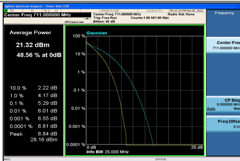
Band17-10MHz-64QAM-23800-50RB#0
