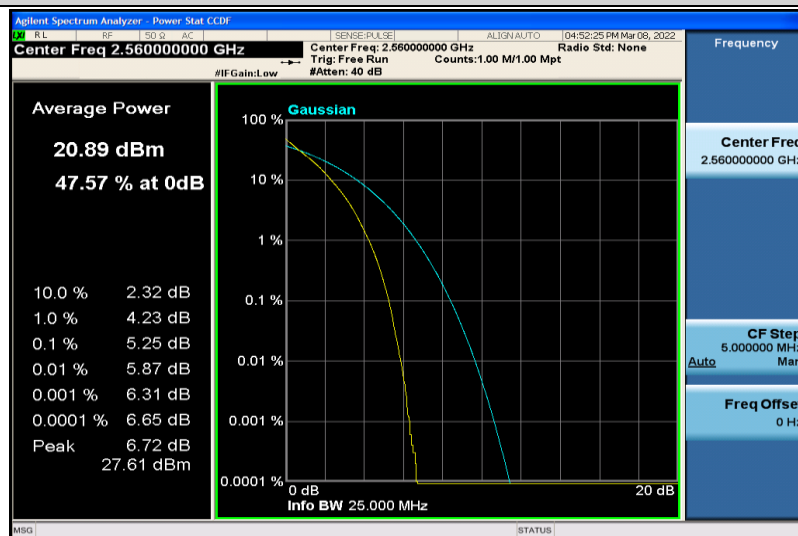
Band7-20MHz-64QAM-21350-100RB#0
