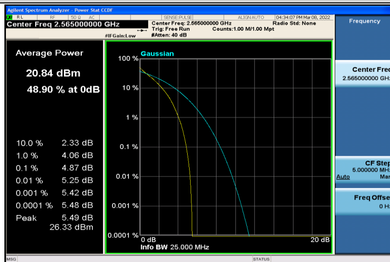
Band7-10MHz-64QAM-21400-50RB#0
