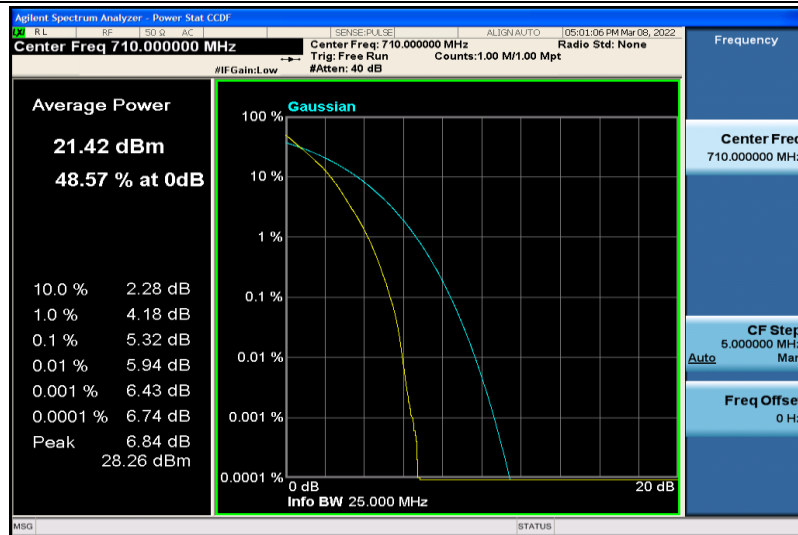
Band17-5MHz-64QAM-23790-25RB#0
