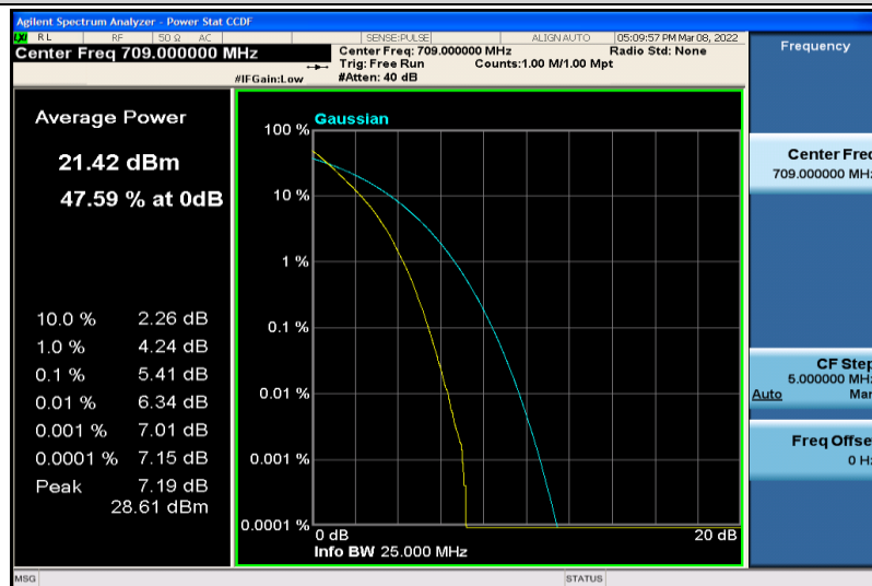
Band17-10MHz-64QAM-23780-50RB#0
