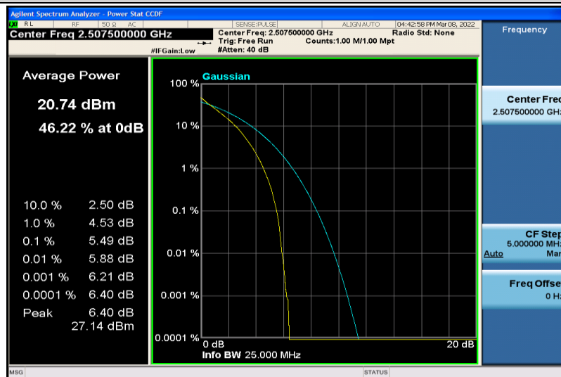
Band7-15MHz-64QAM-20825-75RB#0
