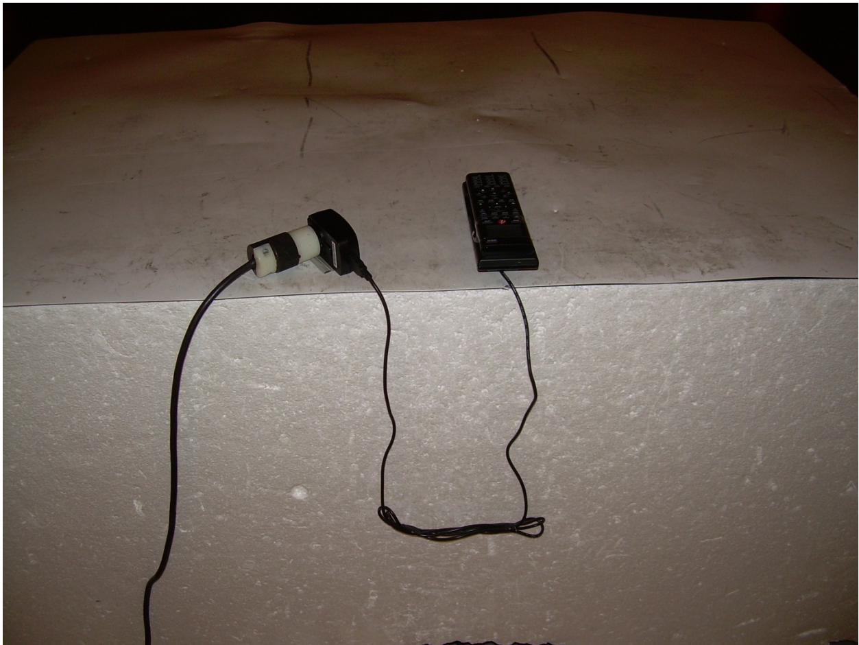
Photograph 2 – Back View Radiated Disturbance Configuration in C4-SRRS
