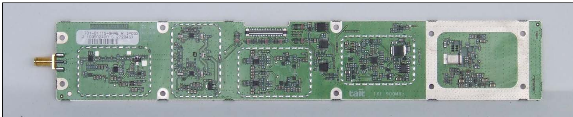
Photograph 09: TXF PCB – Top. Shields Removed
