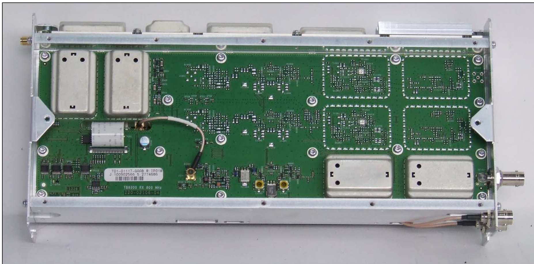
Photograph 04: Rx PCB - Top
