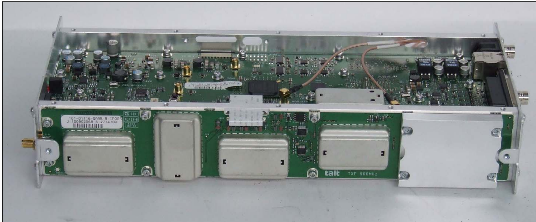
Photograph 08: TXF PCB – Top
