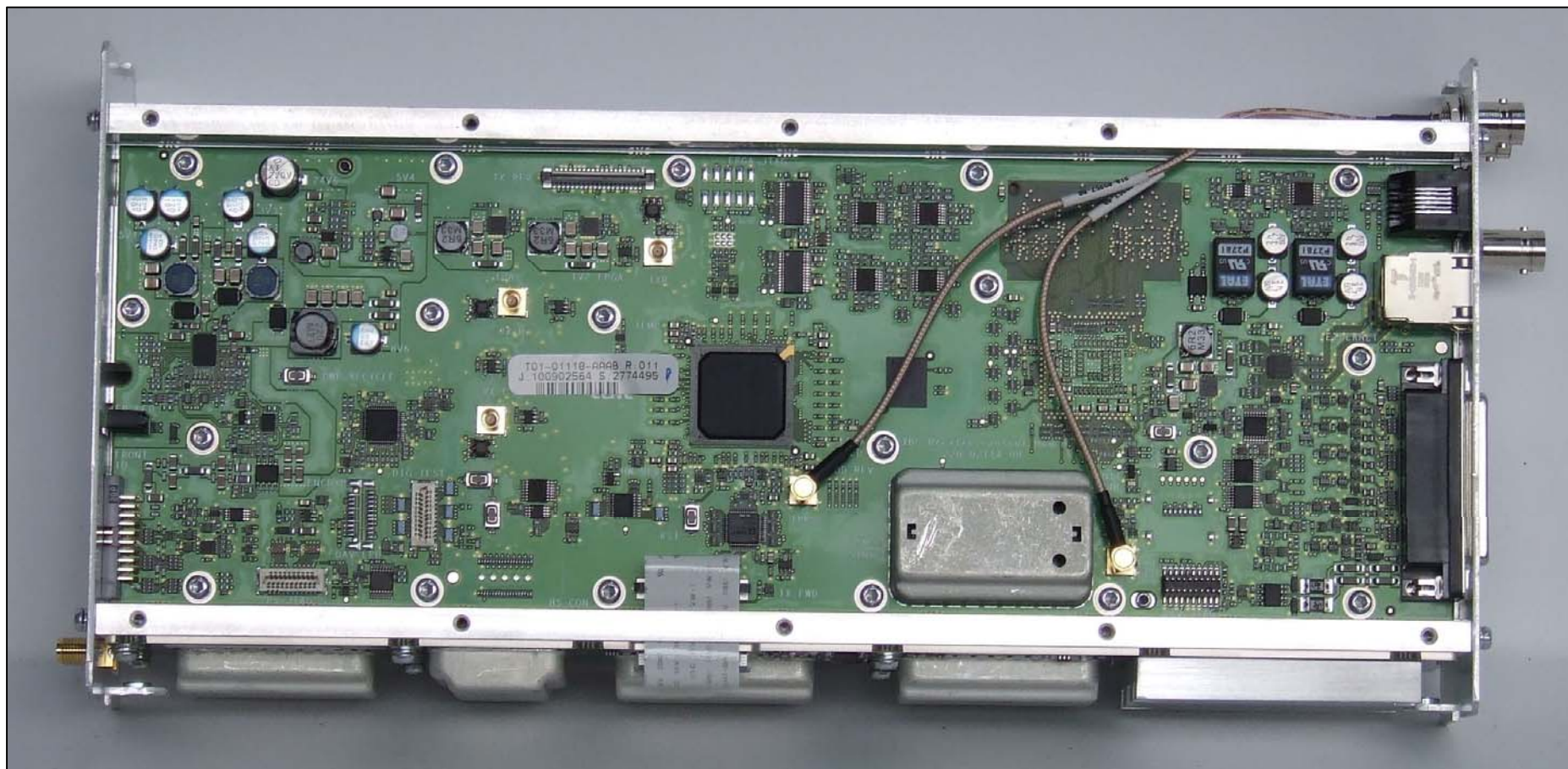
Photograph 06: Control PCB - Top
