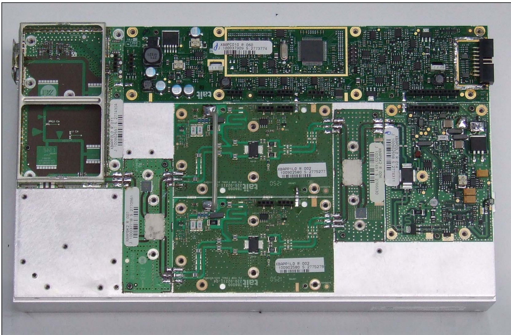
Photograph 02: 100W PA modules – Top. Shields Removed
