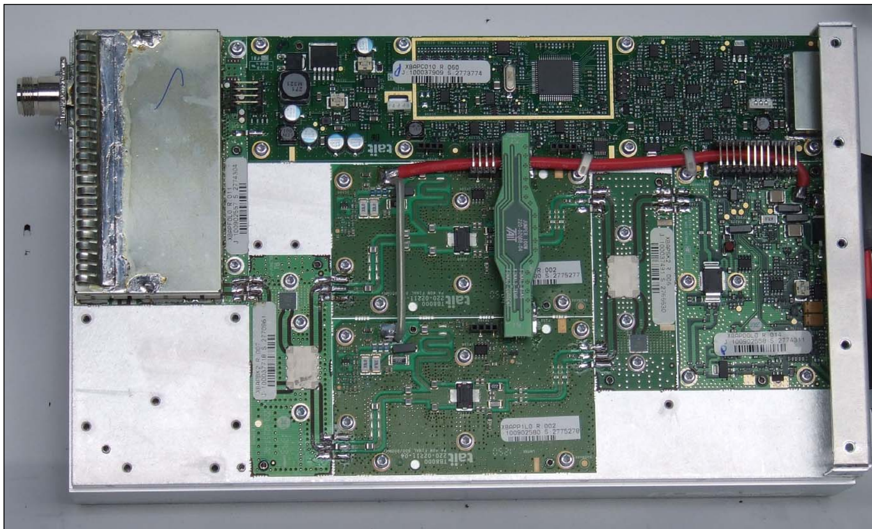
Photograph 01: 100W PA modules – Internal view
