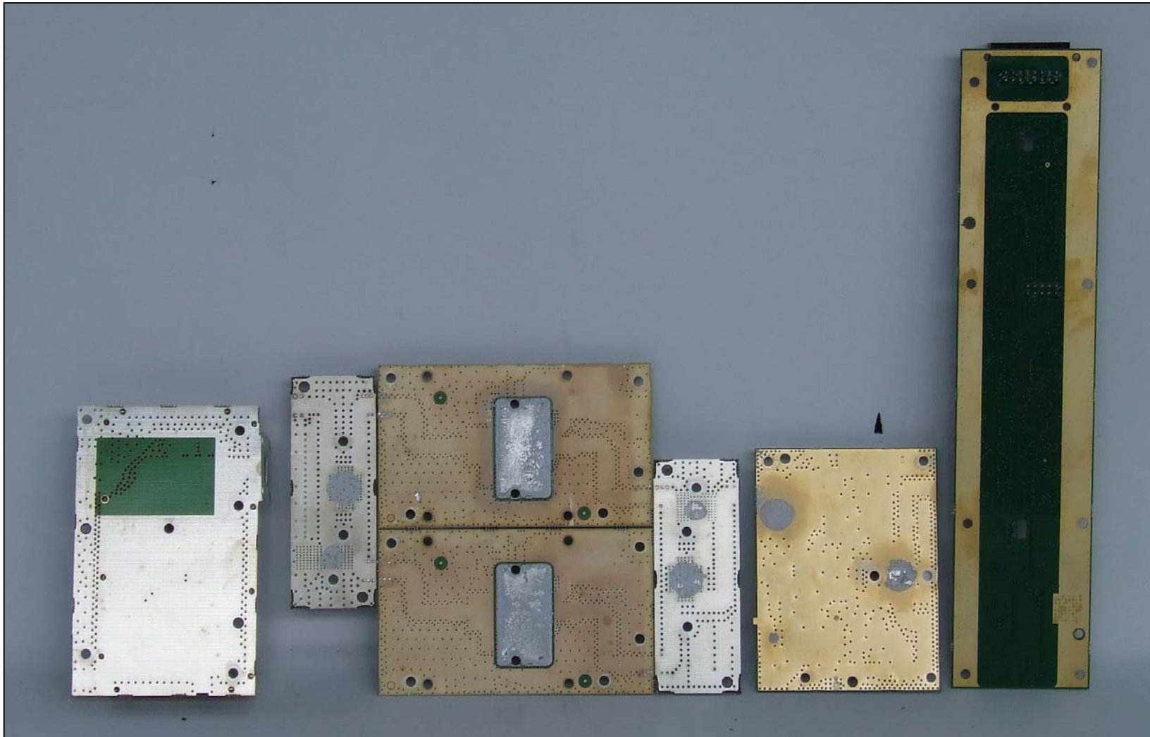
Photograph 03: 100W PA modules - Bottom
