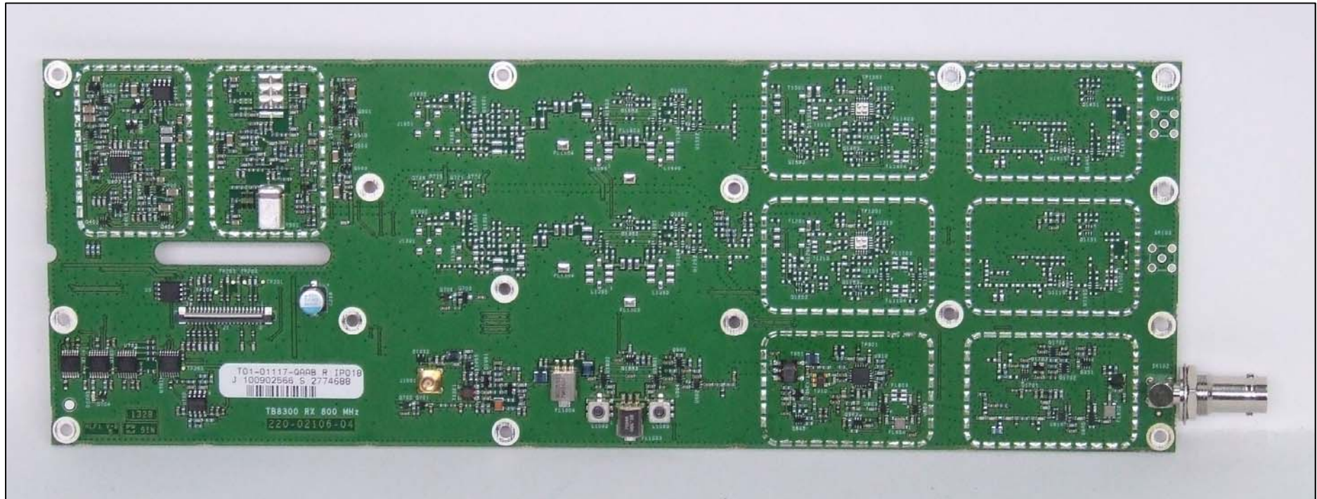
Photograph 05: Rx PCB – Top. Shields Removed
