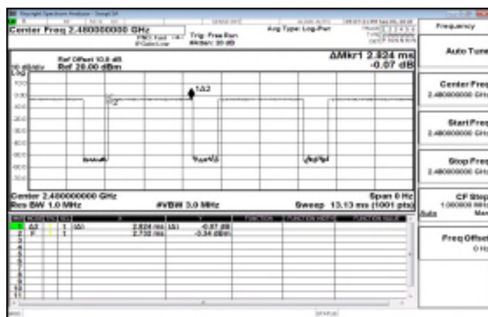
Dwell Time_π4DQPSK_2M_DH5_2480MHz
