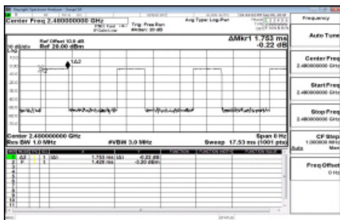
Dwell Time_π4DQPSK_2M_DH3_2480MHz
