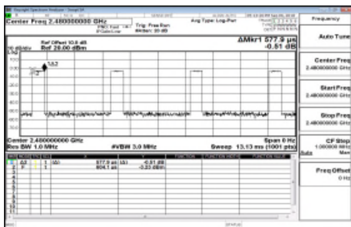
Dwell Time_8DPSK_3M_DH1_2480MHz
