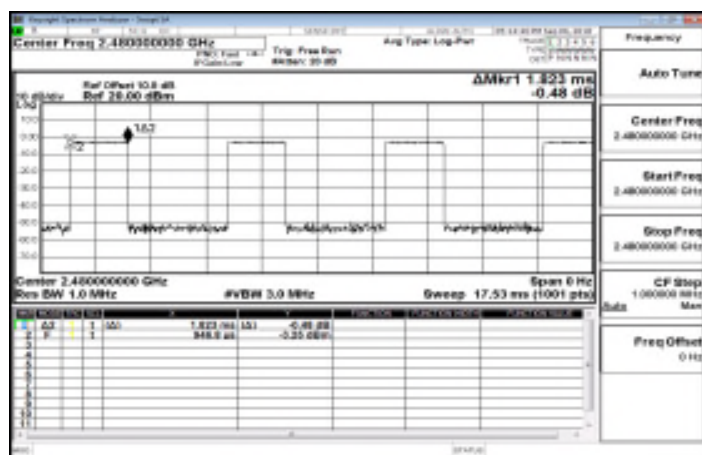
Dwell Time_8DPSK_3M_DH3_2480MHz
