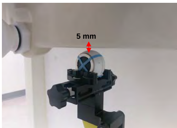
Fig.8 EUT Top-Right side to flat phantom
