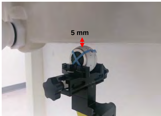
Fig.9 EUT Right-Bottom side to flat phantom
