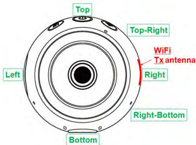
Fig.10 EUT front view (include WLAN/BT antennal location and surface definition)
