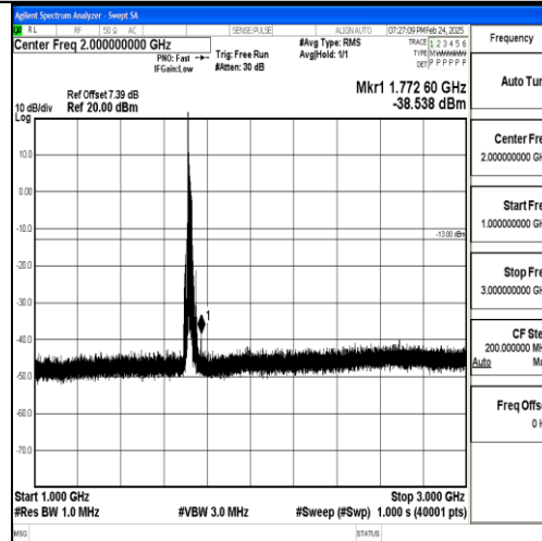
Band4_20MHz_16QAM_20050_1RB#0_1000~3000_1000~3000
