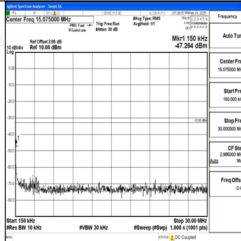
Band4_20MHz_16QAM_20050_1RB#0_0.15~30_0.15~30
