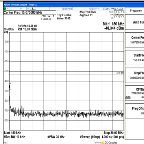
Band4_15MHz_QPSK_20175_1RB#0_0.15~30_0.15~30
