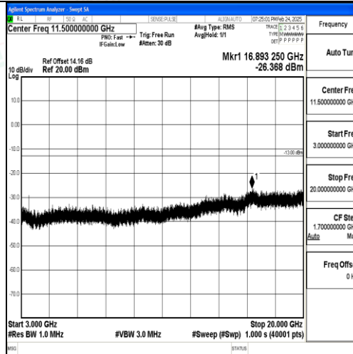
Band4_15MHz_QPSK_20325_1RB#0_3000~20000_3000~20000
