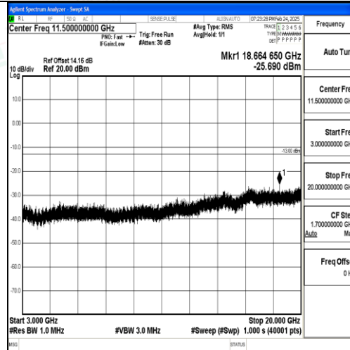
Band4_15MHz_16QAM_20025_1RB#0_3000~20000_3000~20000
