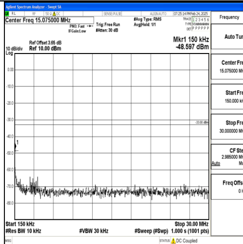
Band4_15MHz_16QAM_20325_1RB#0_0.15~30_0.15~30
