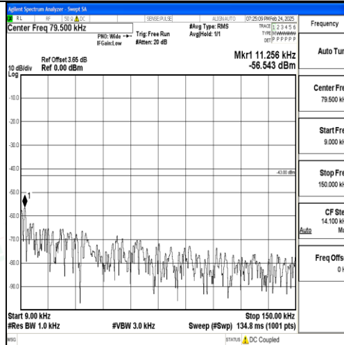
Band4_15MHz_16QAM_20325_1RB#0_0.009~0.15_0.009~0.15
