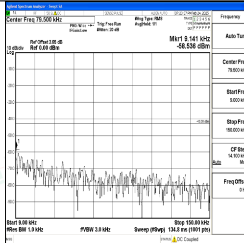
Band4_15MHz_QPSK_20175_1RB#0_0.009~0.15_0.009~0.15
