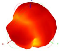
2500.0MHz H+V, Ef: 15.2%
