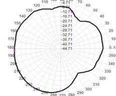
Total(H+V), Max=-4.71dB, Crd=14.53
