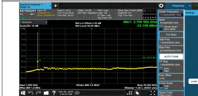
Band41-5MHz-QPSK-41565-1RB#24-1000~20000-PASS
