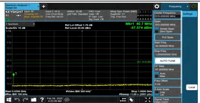
Band41-20MHz-QPSK-40620-1RB#99-30~1000-PASS
