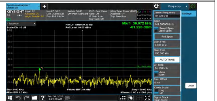
Band 41-20MHz-QPSK-39750-1RB#99-0.009~0.15-PASS
