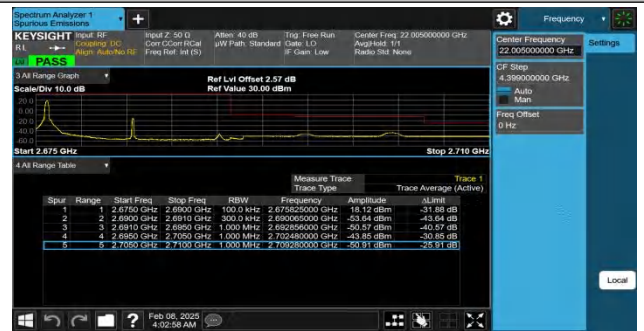
Band41-15MHz-QPSK-41515-1RB#0-PASS
