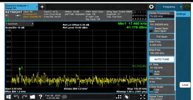
Band41-20MHz-QPSK-40620-1RB#99-0.009~0.15-PASS
