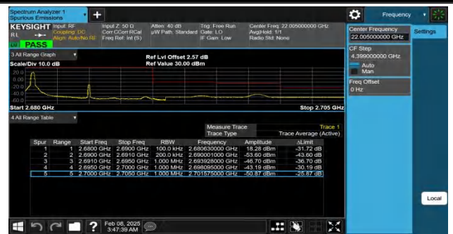
Band41-10MHz-QPSK-41540-1RB#0-PASS
