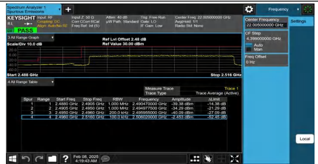
Band41-15MHz-QPSK-39750-100RB#0-PASS
