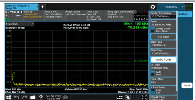
Band41-20MHz-QPSK-41490-1RB#0-0.15~30-PASS
