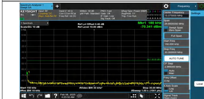
Band41-20MHz-QPSK-40620-1RB#99-0.15~30-PASS
