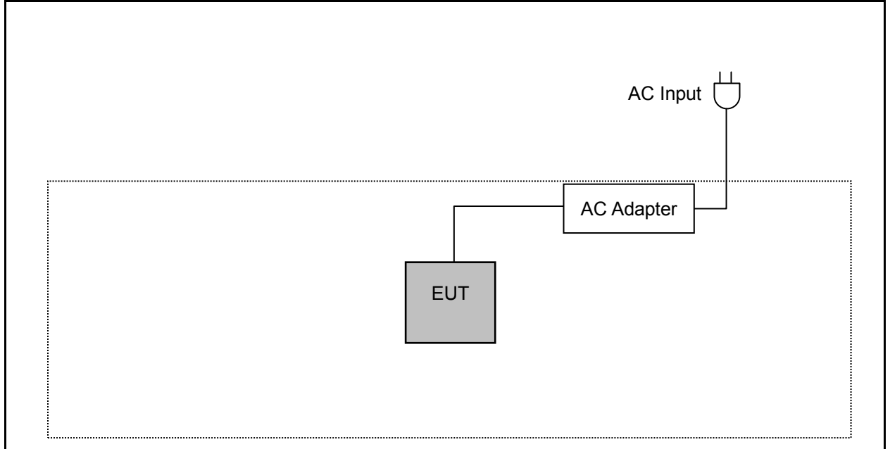
Radiated Emissions
