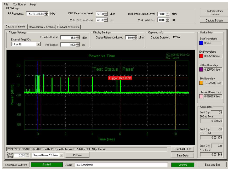
Figure 5-3. Band 2A Move Time and Aggregate Time
