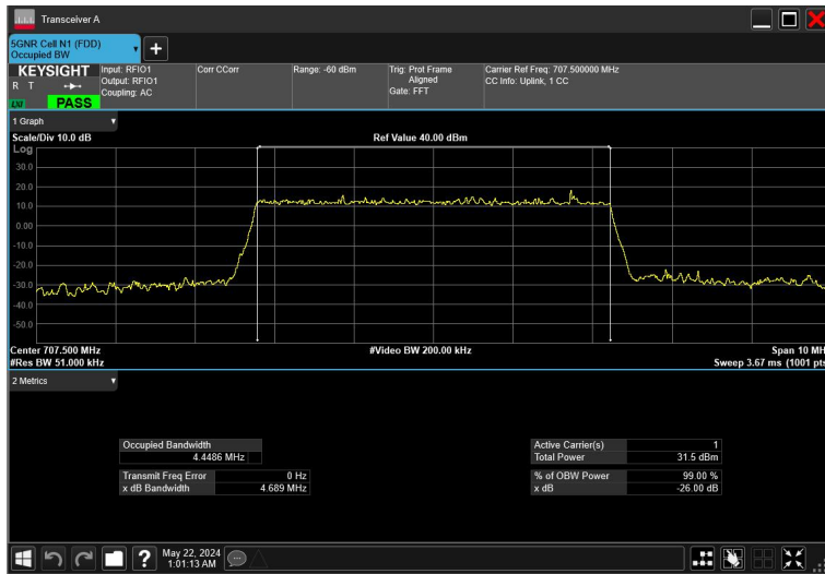
5MHz_15kHz_707.5MHz_DFT-s-OFDM 64 QAM_RB25@0
