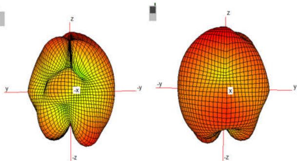
WIFI 6E (6500 MHz)
