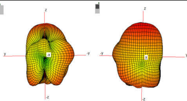
WIFI 5G (5800 MHz)
