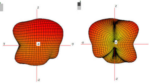
WIFI 5G (5200 MHz)
