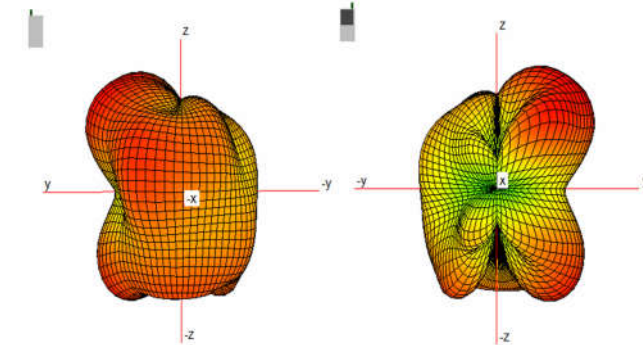
WIFI 6E (6500 MHz)
