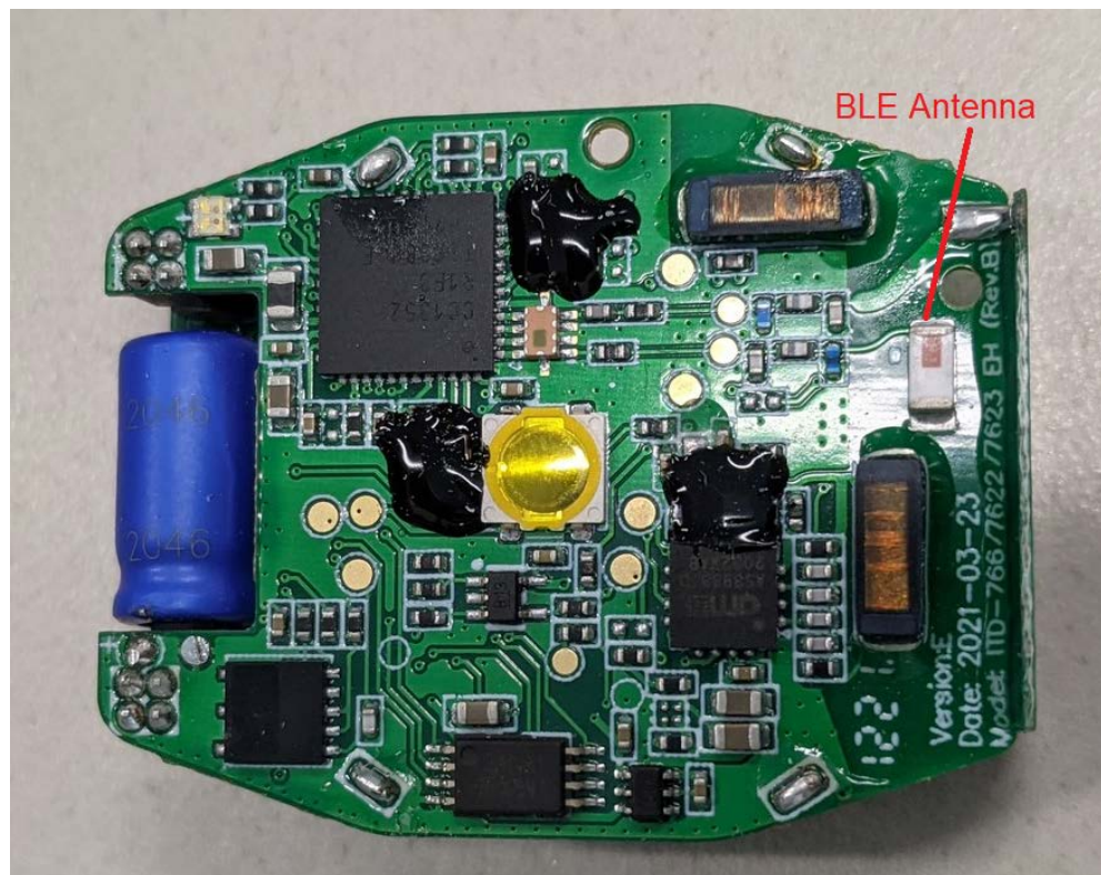
PCB Components Side View
