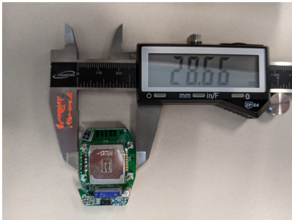
PCB Dimension
