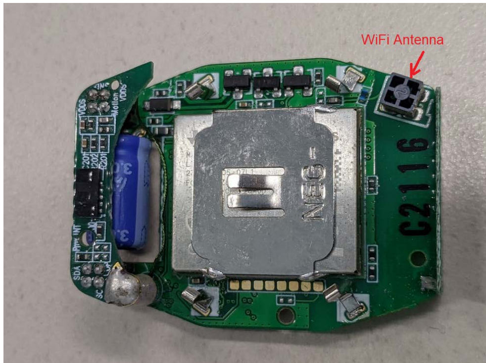
PCB Foil Side View
