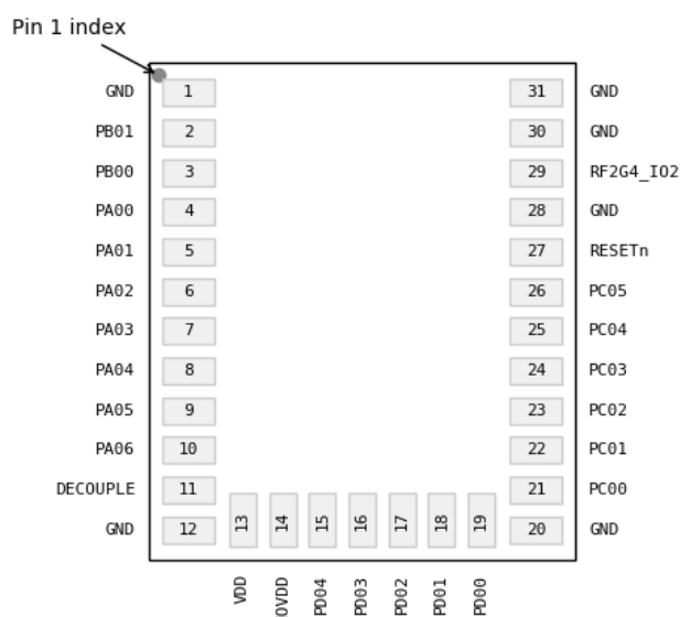
Figure 6.1. MGM210P Module Pinout
