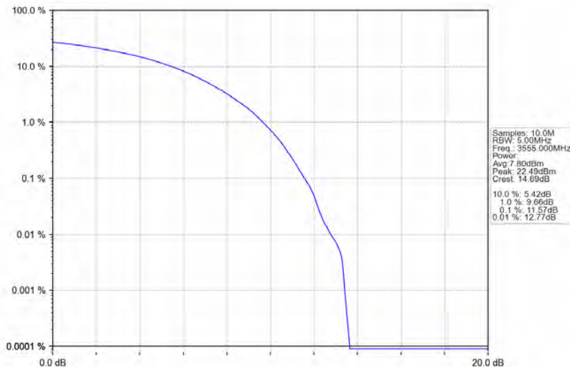
n48_30kHz_MIMO_NTNV_10MHz_CP-OFDM_16_QAM_3555MHz_Outer_Full
