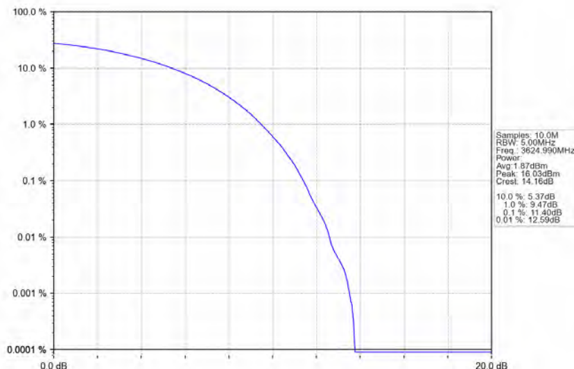
n48_30kHz_MIMO_NTNV_40MHz_CP-OFDM_QPSK_3624.99MHz_Outer_Full
