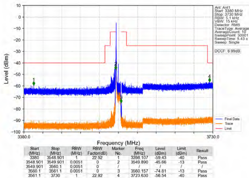
n48_30kHz_MIMO_NTNV_10MHz_CP-OFDM_QPSK_3555MHz_Edge_1RB_Left
