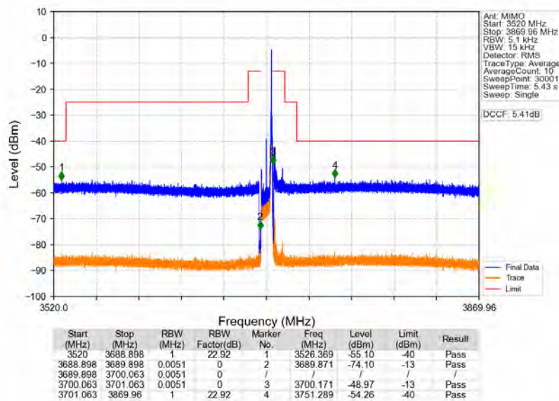
n48_30kHz_MIMO_NTNV_10MHz_CP-OFDM_QPSK_3694.98MHz_Edge_1RB_Right
