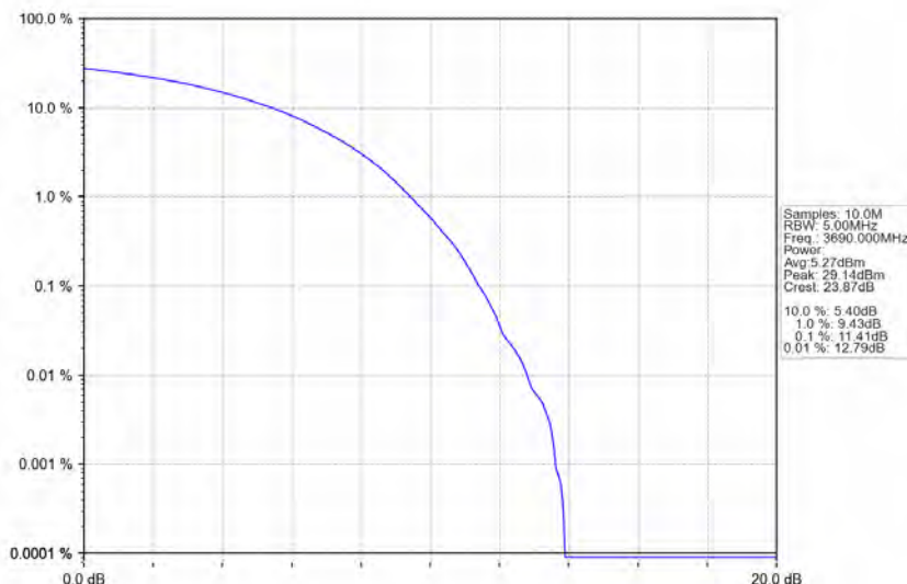
n48_30kHz_MIMO_NTNV_20MHz_CP-OFDM 16 QAM_3690MHz_Outer_Full
