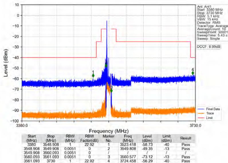
n48_30kHz_MIMO_NTNV_10MHz_CP-OFDM_QPSK_3555MHz_Inner_1RB_Left
