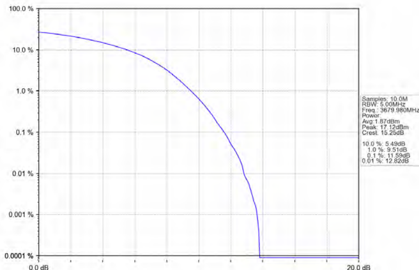
n48_30kHz_MIMO_NTNV_40MHz_CP-OFDM 16 QAM 3679.98MHz_Outer_Full
