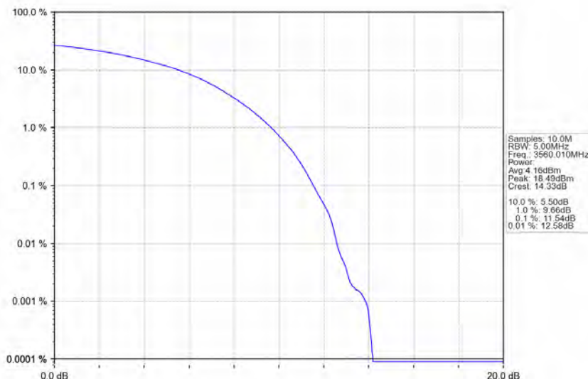
n48_30kHz_MIMO_NTNV_20MHz_CP-OFDM 64 QAM_3560.01MHz_Outer_Full
