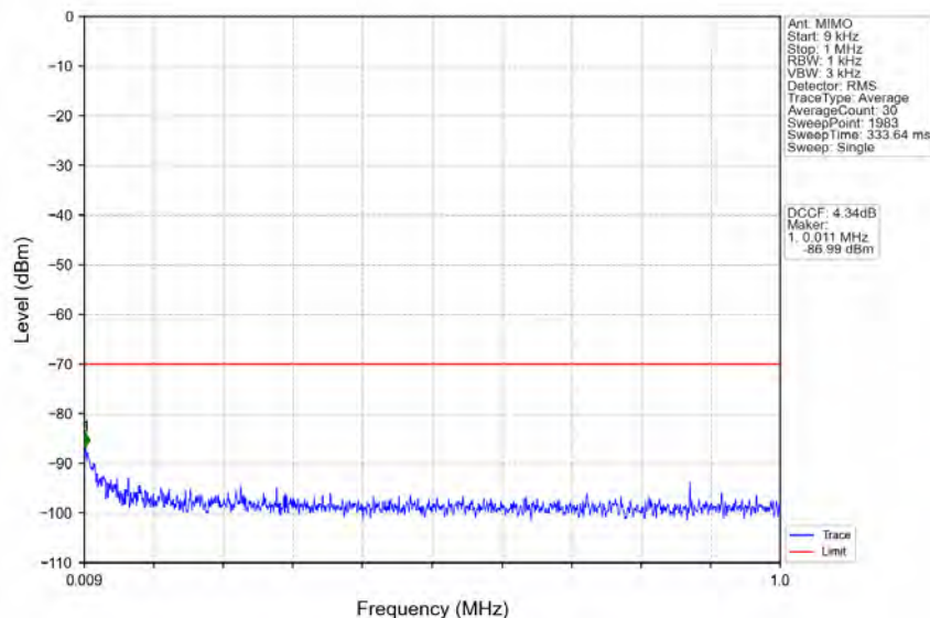
n48_30kHz_MIMO_NTNV_10MHz_CP-OFDM_QPSK_3694.98MHz_Inner_1RB_Right
