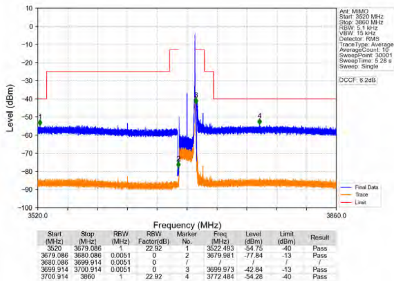
n48_30kHz_MIMO_NTNV_20MHz_CP-OFDM_QPSK_3690MHz_Edge_1RB_Right
