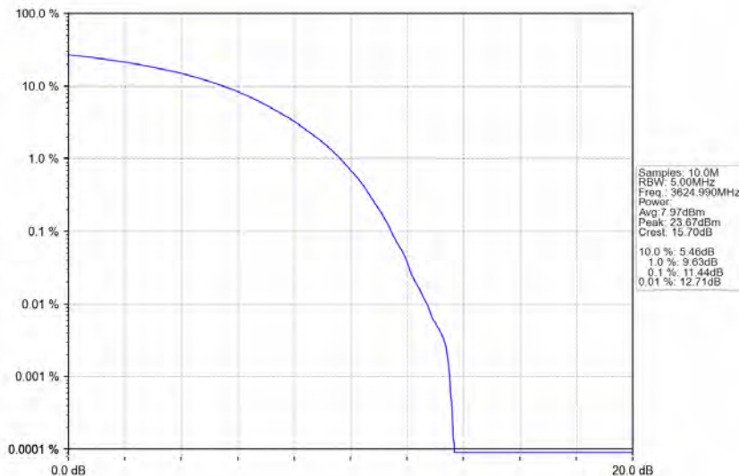
n48_30kHz_MIMO_NTNV_10MHz_CP-OFDM_16_QAM_3624.99MHz_Outer_Full
