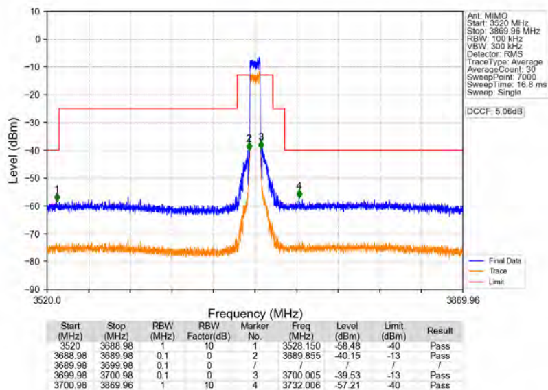
n48_30kHz_MIMO_NTNV_10MHz_CP-OFDM_QPSK_3694.98MHz_Outer_Full
