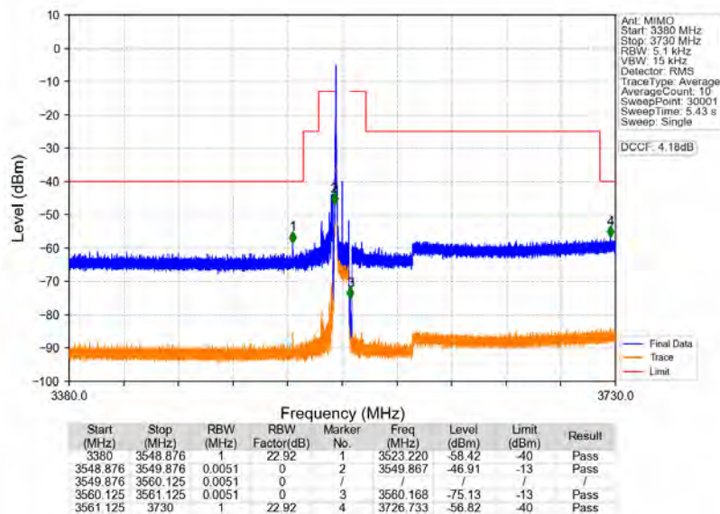
n48_30kHz_MIMO_NTNV_10MHz_CP-OFDM_QPSK_3555MHz_Edge_1RB_Left
