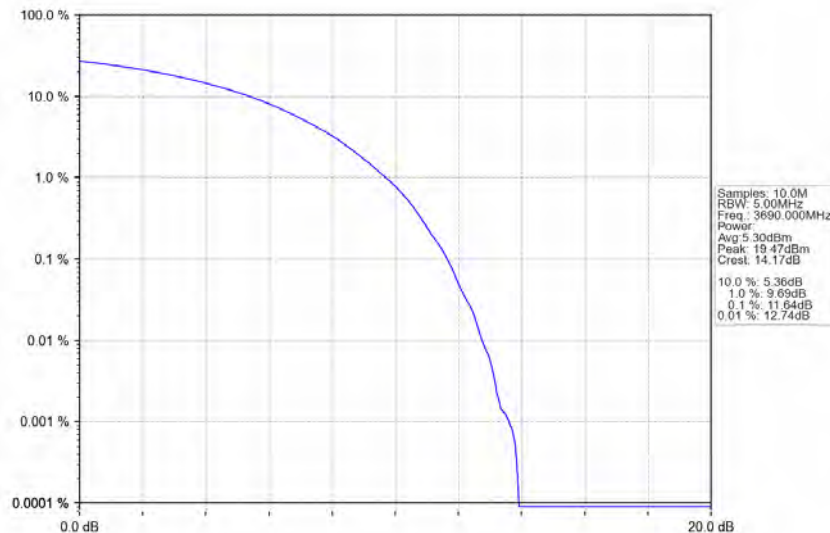
n48_30kHz_MIMO_NTNV_20MHz_CP-OFDM_QPSK_3690MHz_Outer_Full
