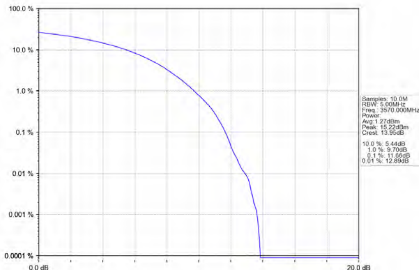
n48_30kHz_MIMO_NTNV_40MHz_CP-OFDM 64 QAM 3570MHz_Outer_Full
