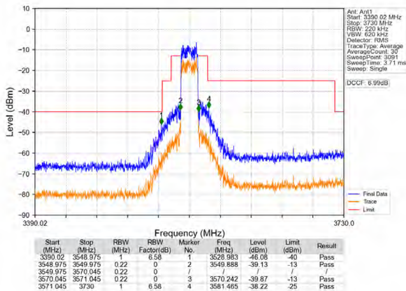
n48_30kHz_MIMO_NTNV_20MHz_CP-OFDM_QPSK_3560.01MHz_Outer_Full
