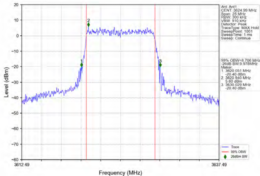
n48_30kHz_MIMO_NTNV_10MHz_CP-OFDM_256_QAM_3624.99MHz_Outer_Full
