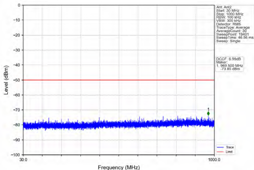
n48_30kHz_MIMO_NTNV_20MHz_CP-OFDM_QPSK_3560.01MHz_Edge_1RB_Left
