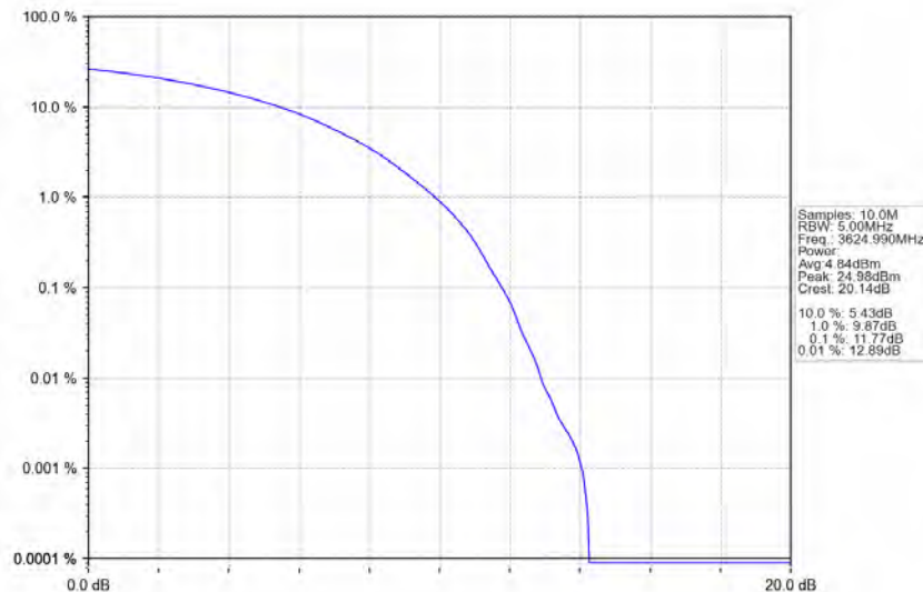
n48_30kHz_MIMO_NTNV_20MHz_CP-OFDM_QPSK_3624.99MHz_Outer_Full
