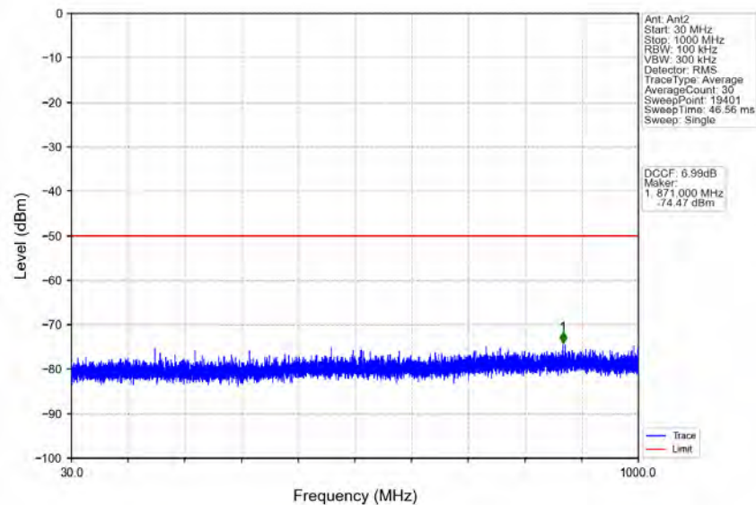
n48_30kHz_MIMO_NTNV_10MHz_CP-OFDM_QPSK_3694.98MHz_Outer_Full
