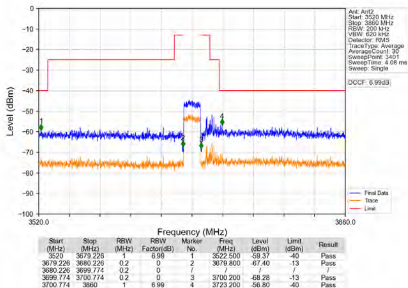
n48_30kHz_MIMO_NTNV_20MHz_CP-OFDM_QPSK_3690MHz_Outer_Full
