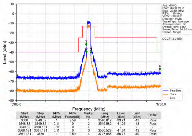
n48_30kHz_MIMO_NTNV_10MHz_CP-OFDM_QPSK_3555MHz_Outer_Full
