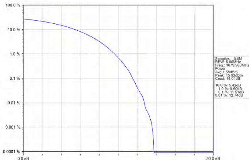
n48_30kHz_MIMO_NTNV_40MHz_CP-OFDM_QPSK_3679.98MHz_Outer_Full
