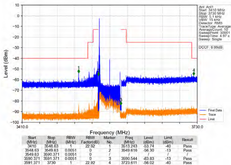
n48_30kHz_MIMO_NTNV_40MHz_CP-OFDM_QPSK_3570MHz_Edge_1RB_Left
