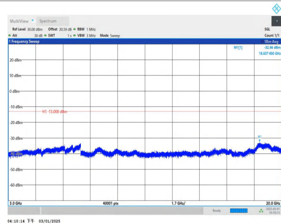
Band4_10MHz_QPSK_20175_1RB#0_3000~20000_3000~2000
