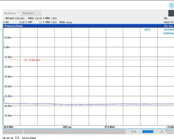
Band4_20MHz_QPSK_20300_1RB#0_30~1000_30~1000
