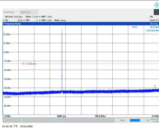
Band4_1.4MHz_QPSK_20393_1RB#0_1000~3000_1000~3000 00
