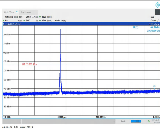
Band4_10MHz_QPSK_20175_1RB#0_1000~3000_1000~3000
