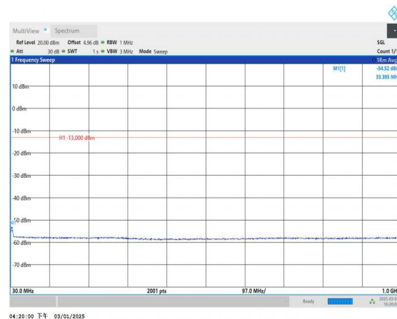
Band4_15MHz_QPSK_20325_1RB#0_30~1000_30~1000
