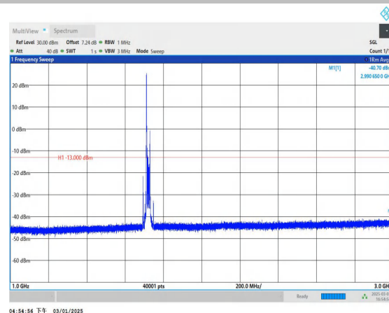
Band4_20MHz_QPSK_20050_1RB#0_1000~3000_1000~3000
