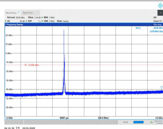
Band4_10MHz_QPSK_20350_1RB#0_1000~3000_1000~3000
