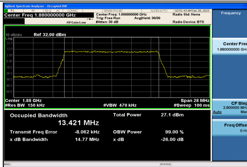
Band2-15MHz-QPSK-18900-75RB#0-13.421
