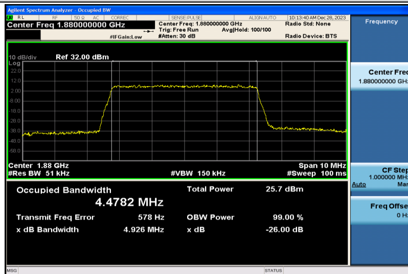
Band2-5MHz-16QAM-18900-25RB#0-4.4782
