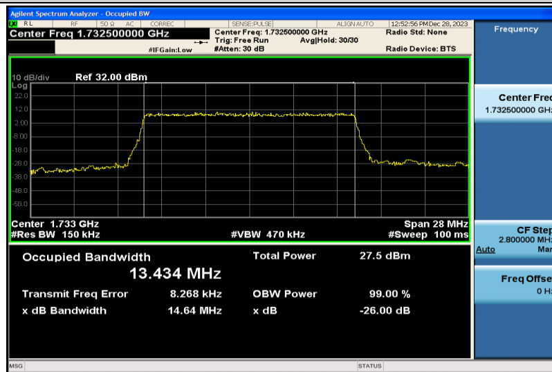
Band4-15MHz-QPSK-20175-75RB#0-13.434
