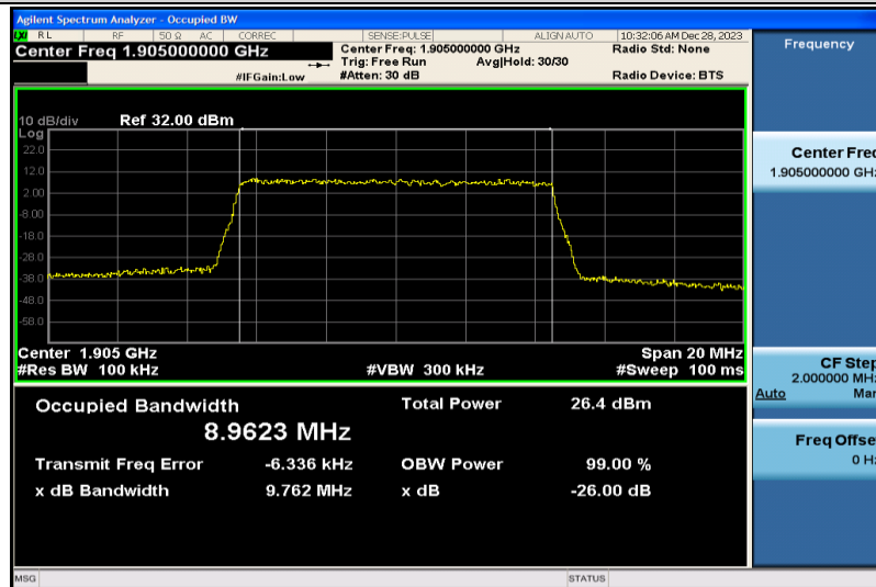
Band2-10MHz-QPSK-19150-50RB#0-8.9623
