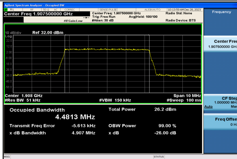
Band2-5MHz-QPSK-19175-25RB#0-4.4813
