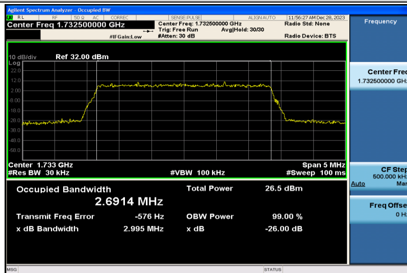
Band4-3MHz-16QAM-20175-15RB#0-2.6914
