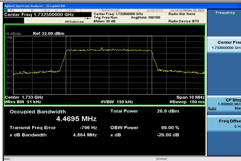
Band4-5MHz-16QAM-20175-25RB#0-4.4695
