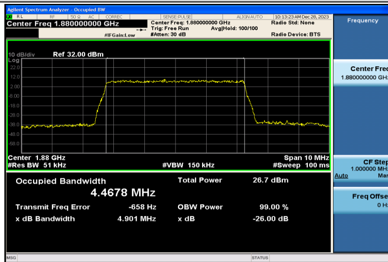
Band2-5MHz-QPSK-18900-25RB#0-4.4678
