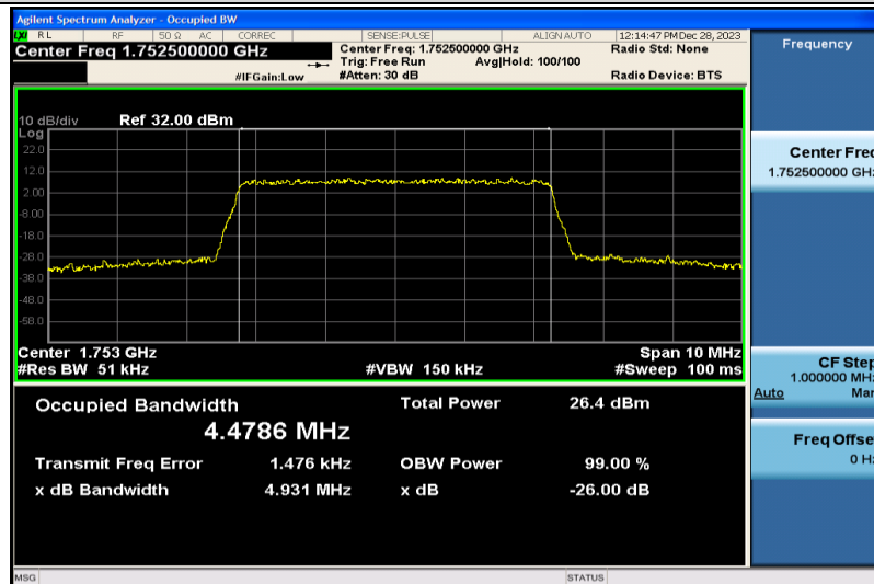
Band4-5MHz-16QAM-20375-25RB#0-4.4786
