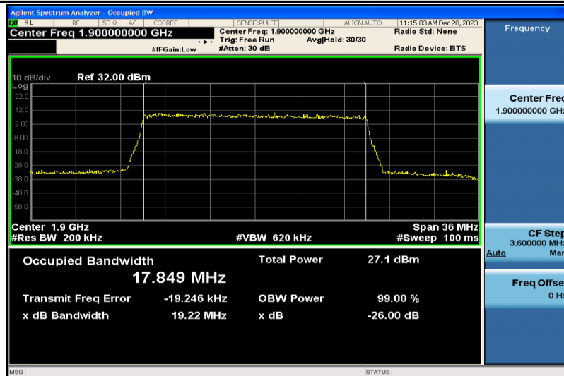
Band2-20MHz-QPSK-19100-100RB#0-17.849
