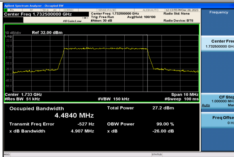
Band4-5MHz-QPSK-20175-25RB#0-4.4840
