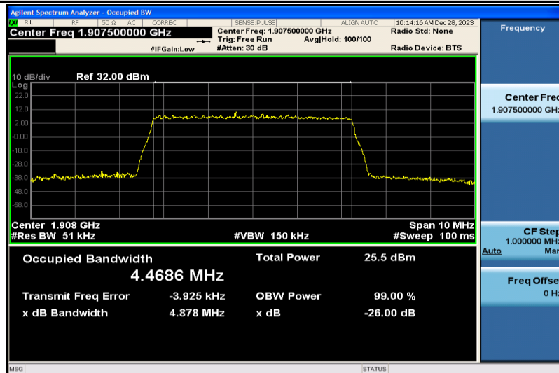
Band2-5MHz-16QAM-19175-25RB#0-4.4686
