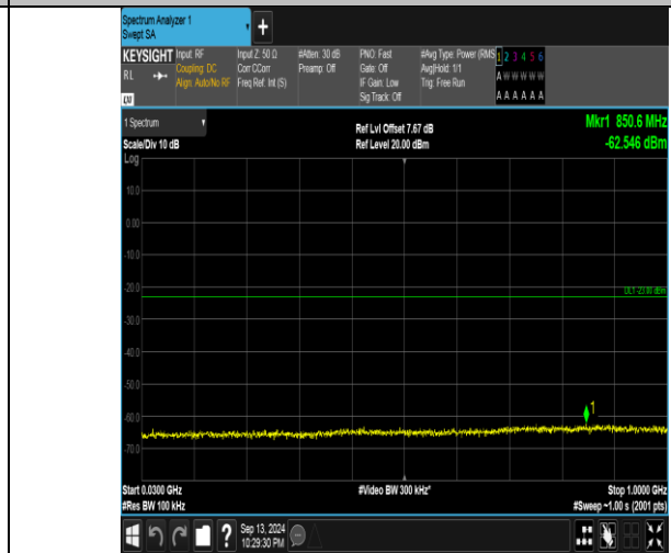
Band66_5MHz_16QAM_131997_25RB#0_30~1000_30~1000
