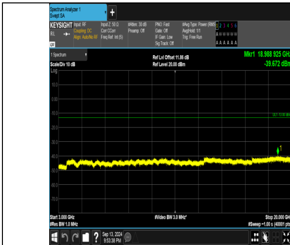
Band66_3MHz_QPSK_132657_15RB#0_3000~20000_3000~20000
