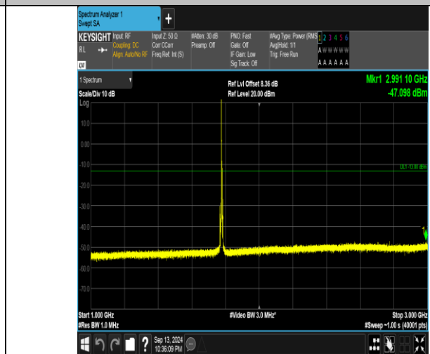
Band66_5MHz_QPSK_132647_1RB#0_1000~3000_1000~3000
