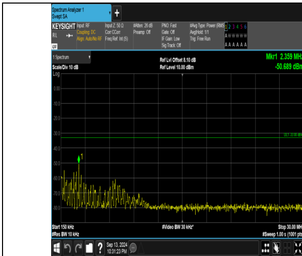
Band66_5MHz_16QAM_132322_1RB#0_0.15~30_0.15~30
