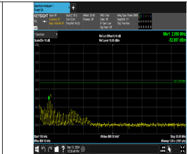
Band66_5MHz_QPSK_132647_1RB#0_0.15~30_0.15~30
