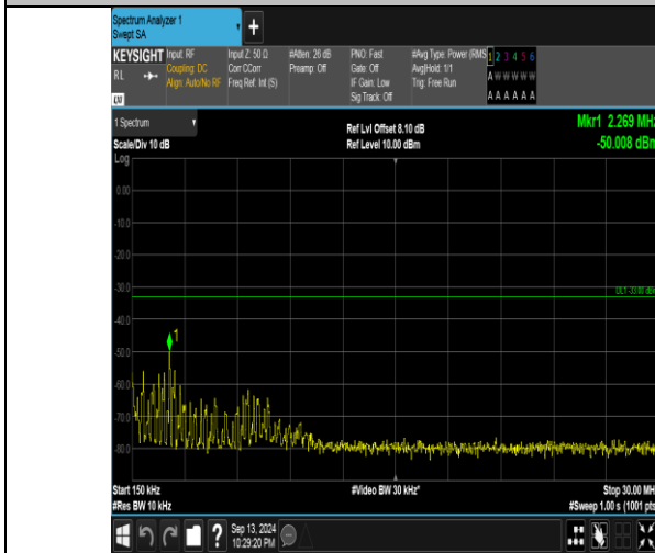
Band66_5MHz_16QAM_131997_25RB#0_0.15~30_0.15~30
