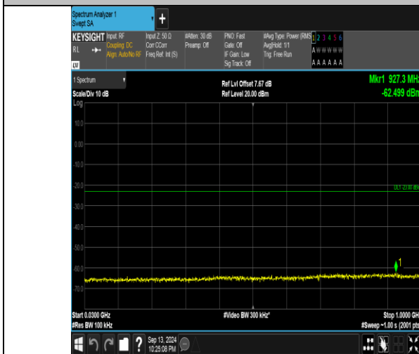
Band66_5MHz_QPSK_131997_1RB#0_30~1000_30~1000
