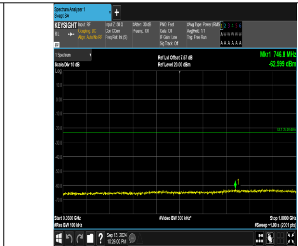
Band66_5MHz_16QAM_131997_1RB#0_30~1000_30~1000
