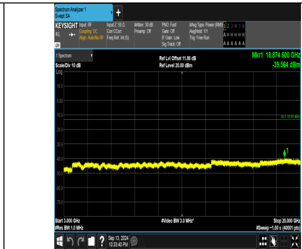
Band66_5MHz_16QAM_132322_1RB#24_3000~20000_3000~20000
