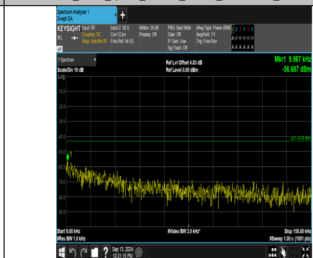
Band66_5MHz_16QAM_132322_1RB#0_0.009~0.15_0.009~0.15
