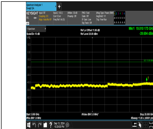
Band66_5MHz_QPSK_131997_25RB#0_3000~20000_3000~20000
