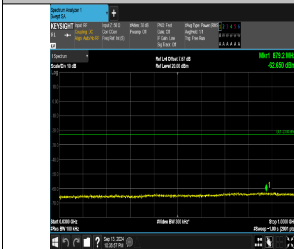
Band66_5MHz_QPSK_132647_1RB#0_30~1000_30~1000
