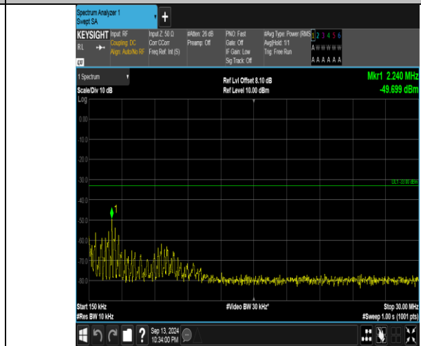
Band66_5MHz_QPSK_132322_25RB#0_0.15~30_0.15~30
