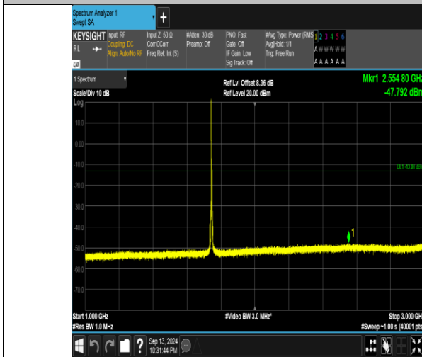
Band66_5MHz_16QAM_132322_1RB#0_1000~3000_1000~3000
