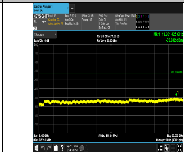
Band66_3MHz_16QAM_132657_15RB#0_3000~20000_3000~20000
