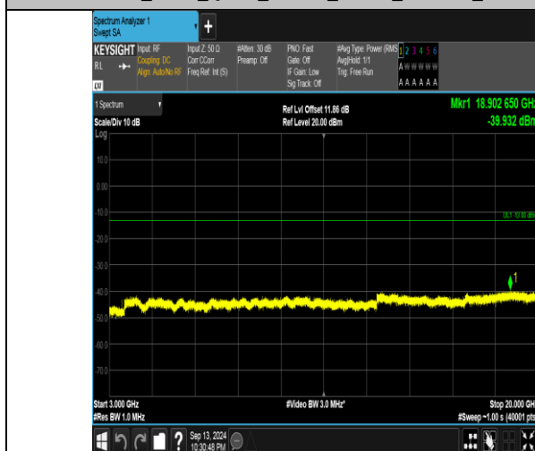
Band66_5MHz_QPSK_132322_1RB#0_3000~20000_3000~20000
