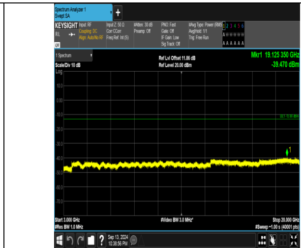
Band66_5MHz_16QAM_132647_1RB#24_3000~20000_3000~20000
