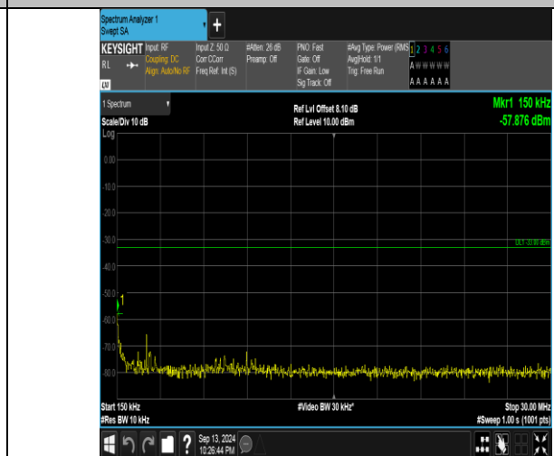
Band66_5MHz_QPSK_131997_1RB#24_0.15~30_0.15~30
