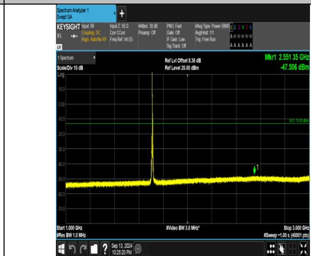
Band66_5MHz_QPSK_131997_1RB#0_1000~3000_1000~3000
