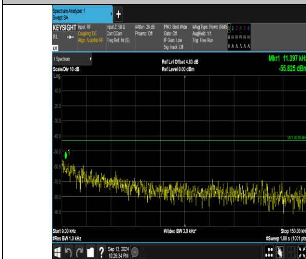
Band66_5MHz_QPSK_131997_1RB#24_0.009~0.15_0.009~0.15
