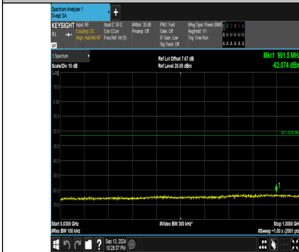
Band66_5MHz_QPSK_131997_25RB#0_30~1000_30~1000
