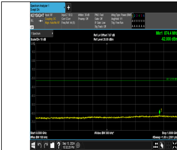
Band66_5MHz_QPSK_132322_1RB#24_30~1000_30~1000
