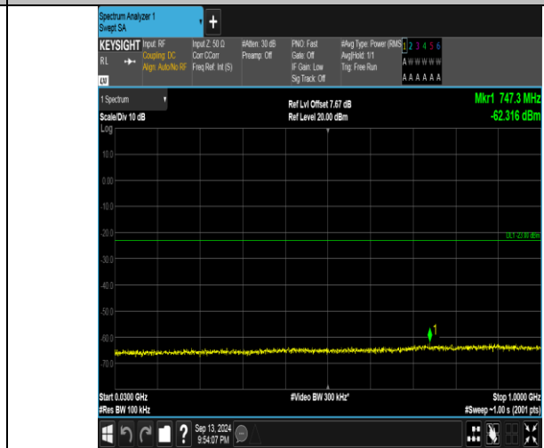
Band66_3MHz_16QAM_132657_15RB#0_30~1000_30~1000
