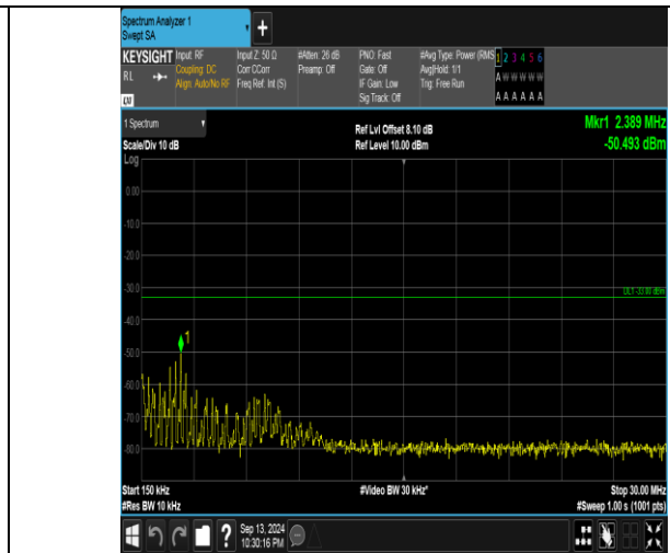
Band66_5MHz_QPSK_132322_1RB#0_0.15~30_0.15~30
