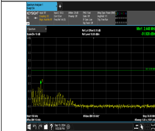
Band66_3MHz_16QAM_132657_15RB#0_0.15~30_0.15~30
