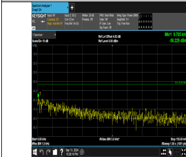
Band66_5MHz_QPSK_131997_25RB#0_0.009~0.15_0.009~0.15
