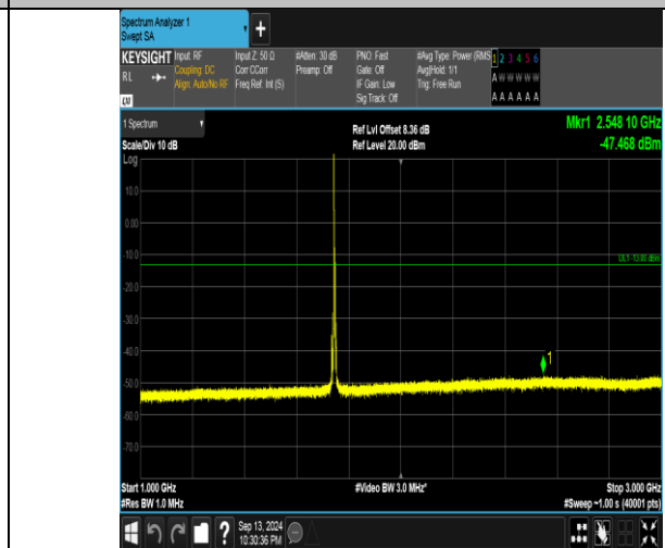
Band66_5MHz_QPSK_132322_1RB#0_1000~3000_1000~3000
