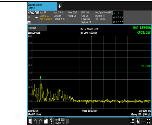
Band66_5MHz_QPSK_131997_1RB#0_0.15~30_0.15~30
