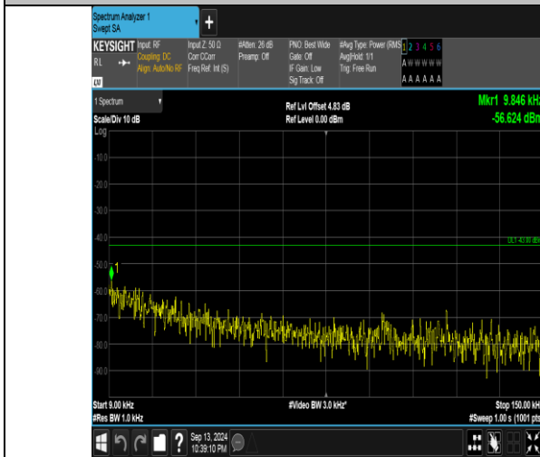
Band66_5MHz_QPSK_132647_25RB#0_0.009~0.15_0.009~0.15
