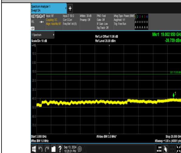
Band66_5MHz_QPSK_131997_1RB#0_3000~20000_3000~20000
