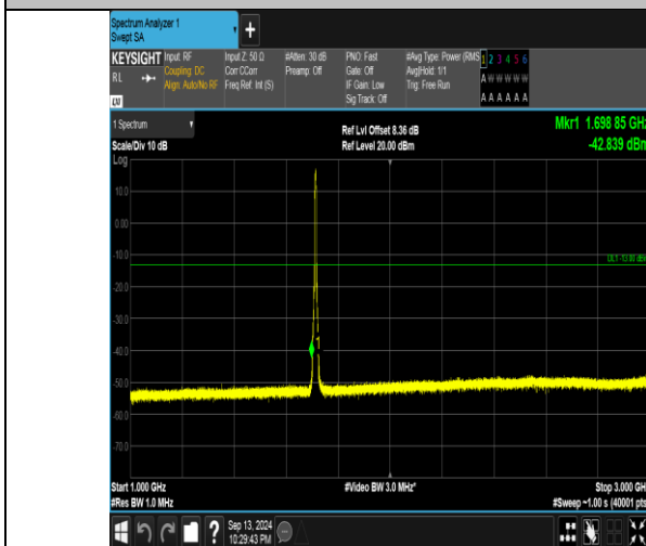
Band66_5MHz_16QAM_131997_25RB#0_1000~3000_1000~3000
