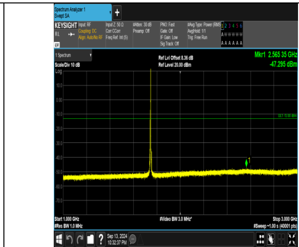
Band66_5MHz_QPSK_132322_1RB#24_1000~3000_1000~3000
