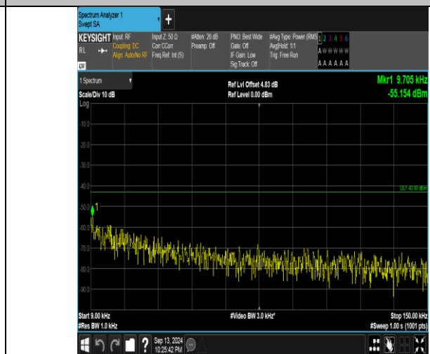
Band66_5MHz_16QAM_131997_1RB#0_0.009~0.15_0.009~0.15
