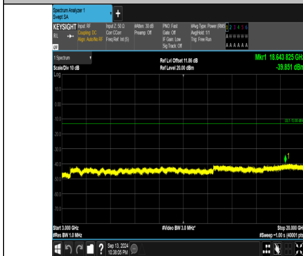
Band66_5MHz_QPSK_132647_1RB#24_3000~20000_3000~20000
