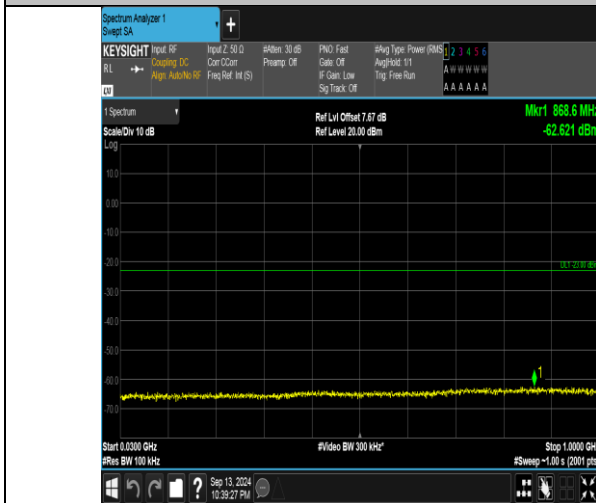
Band66_5MHz_QPSK_132647_25RB#0_30~1000_30~1000
