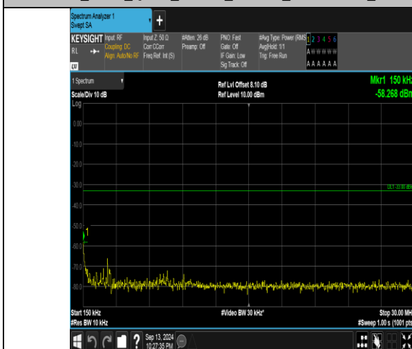
Band66_5MHz_16QAM_131997_1RB#24_0.15~30_0.15~30
