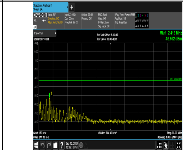
Band66_5MHz_QPSK_132647_25RB#0_0.15~30_0.15~30
