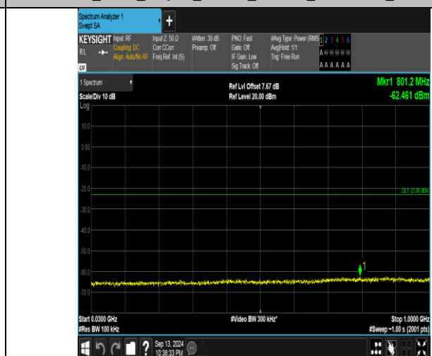
Band66_5MHz_16QAM_132647_1RB#24_30~1000_30~1000
