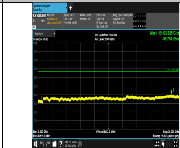
Band66_5MHz_16QAM_131997_1RB#0_3000~20000_3000~20000
