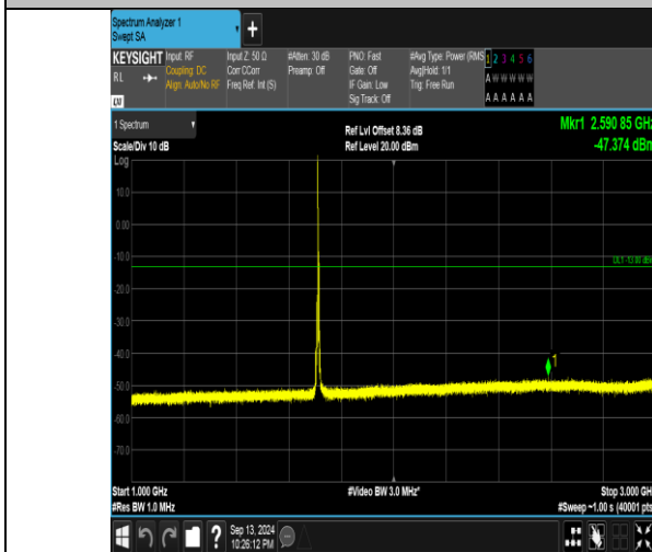
Band66_5MHz_16QAM_131997_1RB#0_1000~3000_1000~3000
