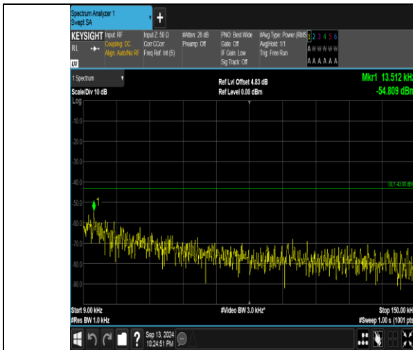
Band66_5MHz_QPSK_131997_1RB#0_0.009~0.15_0.009~0.15
