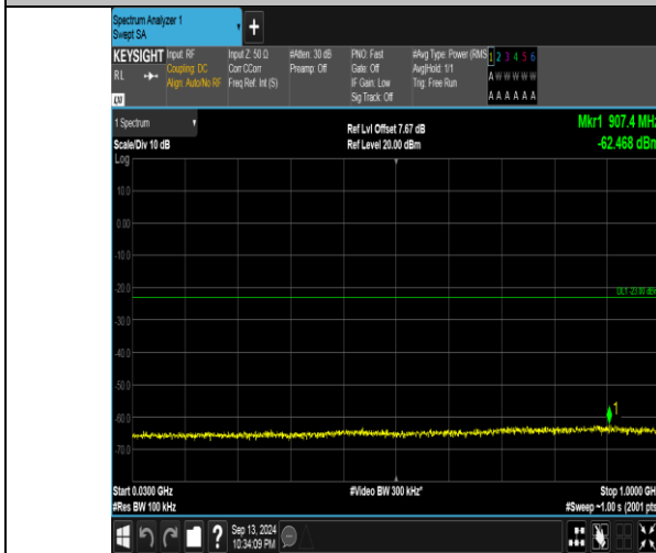
Band66_5MHz_QPSK_132322_25RB#0_30~1000_30~1000
