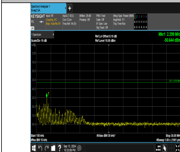
Band66_5MHz_16QAM_132322_1RB#24_0.15~30_0.15~30
