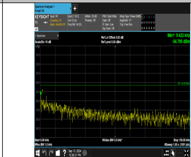
Band66_5MHz_16QAM_132647_1RB#0_0.009~0.15_0.009~0.15
