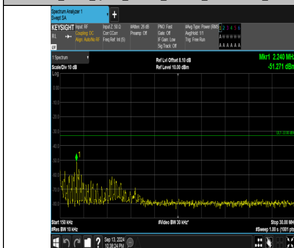
Band66_5MHz_16QAM_132647_1RB#24_0.15~30_0.15~30
