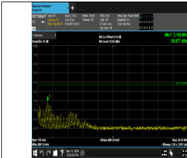
Band66_5MHz_16QAM_131997_1RB#0_0.15~30_0.15~30
