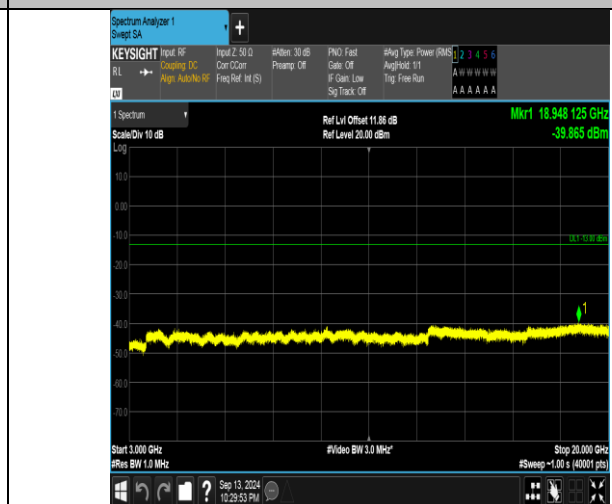
Band66_5MHz_16QAM_131997_25RB#0_3000~20000_3000~20000
