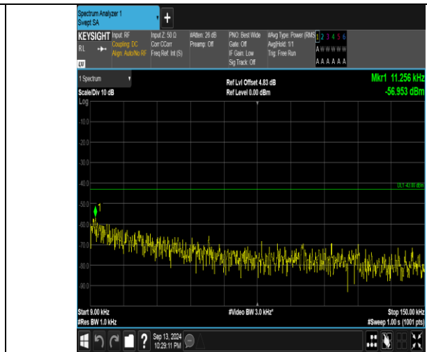
Band66_5MHz_16QAM_131997_25RB#0_0.009~0.15_0.009~0.15
