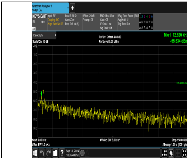
Band66_5MHz_QPSK_132647_1RB#0_0.009~0.15_0.009~0.15
