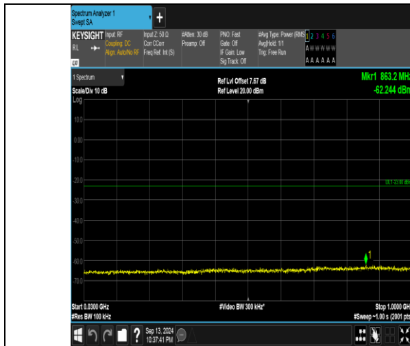
Band66_5MHz_QPSK_132647_1RB#24_30~1000_30~1000
