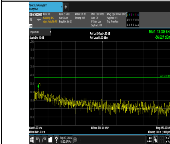
Band66_5MHz_QPSK_132322_1RB#24_0.009~0.15_0.009~0.15
