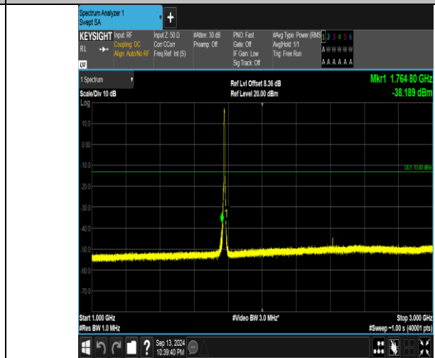
Band66_5MHz_QPSK_132647_25RB#0_1000~3000_1000~3000
