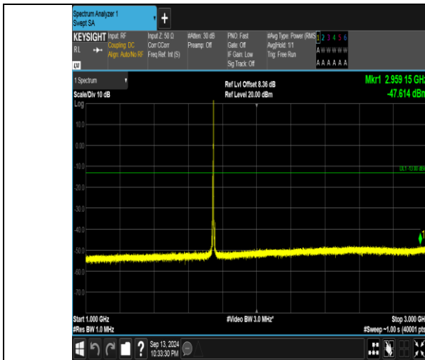
Band66_5MHz_16QAM_132322_1RB#24_1000~3000_1000~3000
