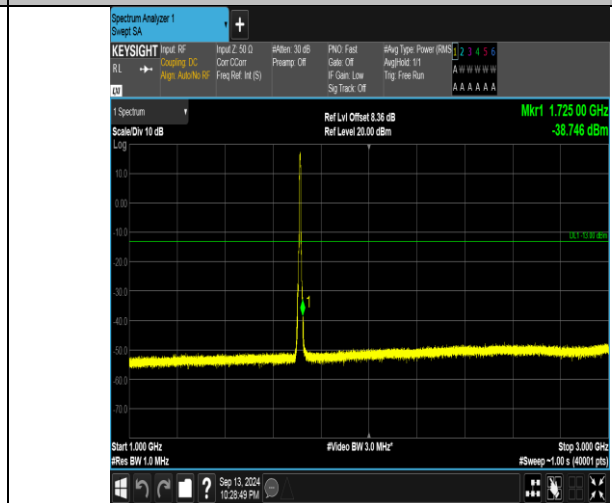
Band66_5MHz_QPSK_131997_25RB#0_1000~3000_1000~3000
