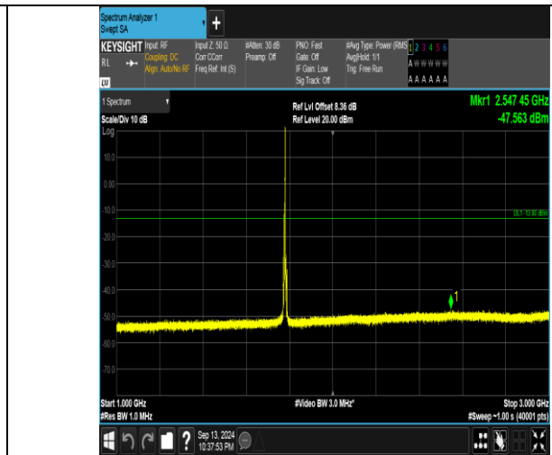
Band66_5MHz_QPSK_132647_1RB#24_1000~3000_1000~3000
