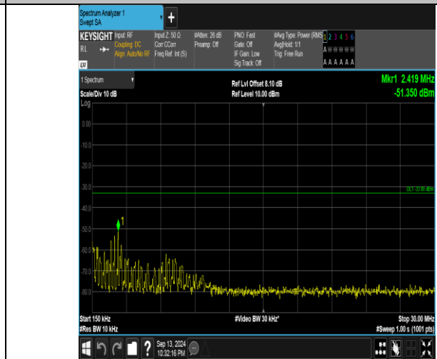
Band66_5MHz_QPSK_132322_1RB#24_0.15~30_0.15~30
