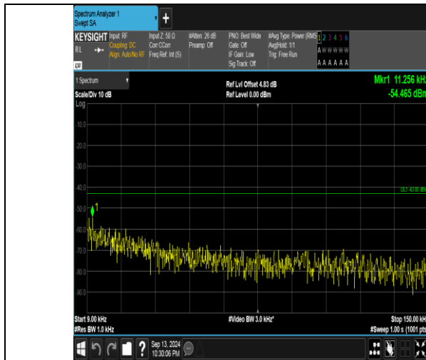
Band66_5MHz_QPSK_132322_1RB#0_0.009~0.15_0.009~0.15
