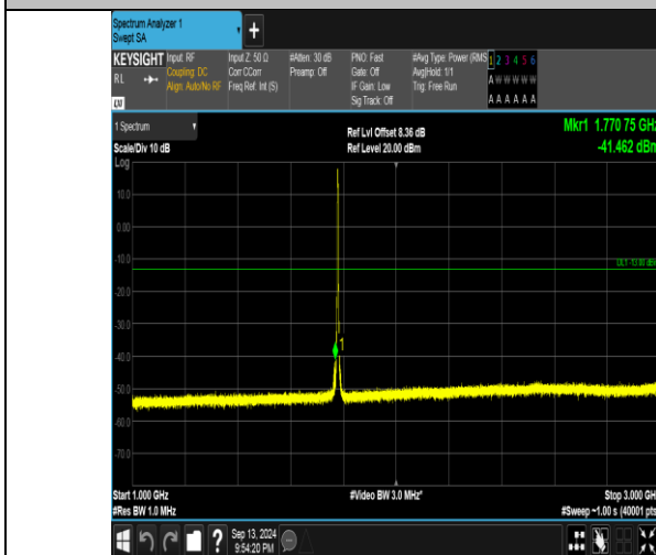
Band66_3MHz_16QAM_132657_15RB#0_1000~3000_1000~3000
