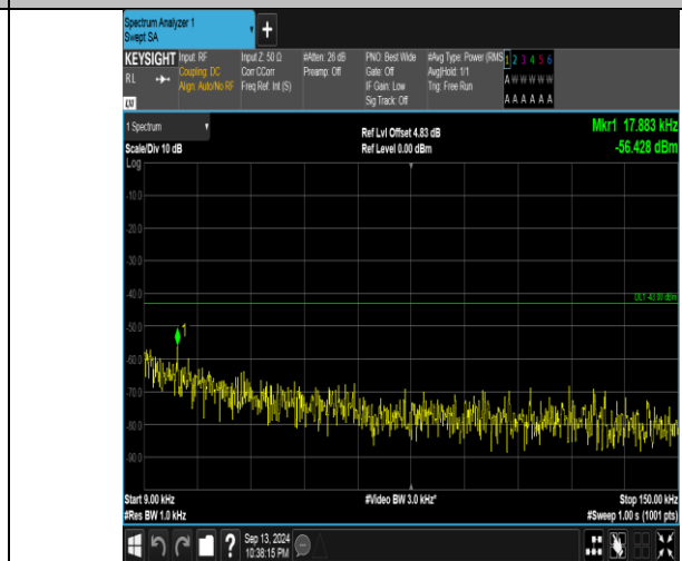
Band66_5MHz_16QAM_132647_1RB#24_0.009~0.15_0.009~0.15
