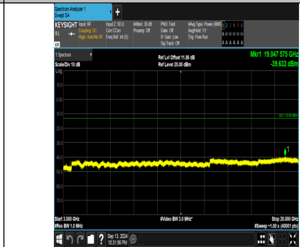
Band66_5MHz_16QAM_132322_1RB#0_3000~20000_3000~20000
