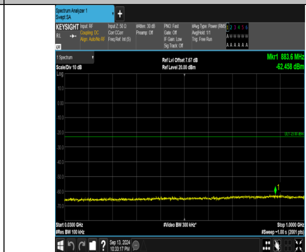
Band66_5MHz_16QAM_132322_1RB#24_30~1000_30~1000
