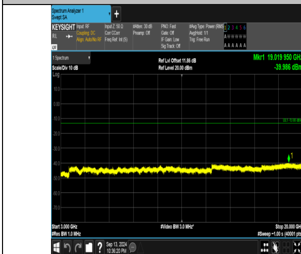
Band66_5MHz_QPSK_132647_1RB#0_3000~20000_3000~20000
