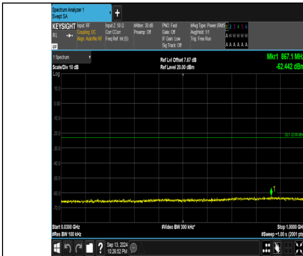
Band66_5MHz_QPSK_131997_1RB#24_30~1000_30~1000
