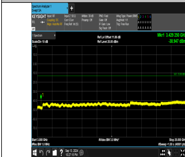
Band66_5MHz_QPSK_131997_1RB#24_3000~20000_3000~20000
