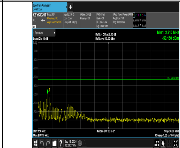
Band66_5MHz_QPSK_131997_25RB#0_0.15~30_0.15~30
