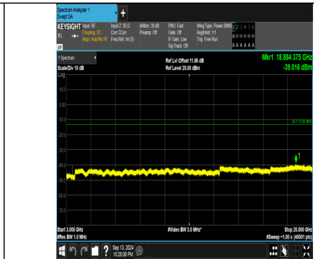
Band66_5MHz_16QAM_131997_1RB#24_3000~20000_3000~20000
