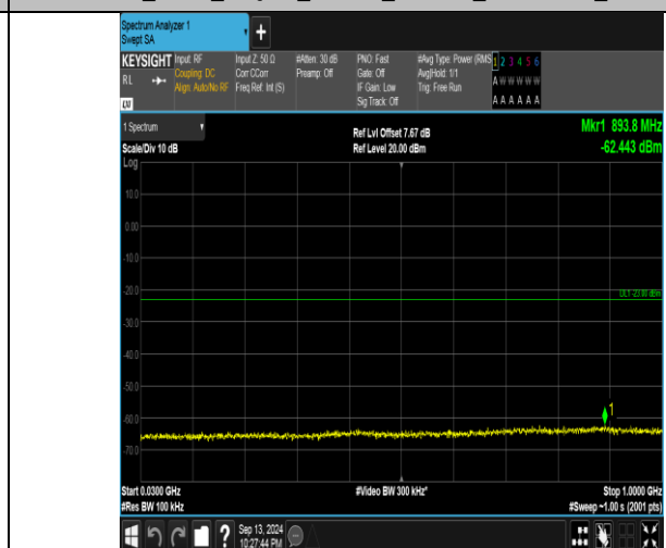
Band66_5MHz_16QAM_131997_1RB#24_30~1000_30~1000
