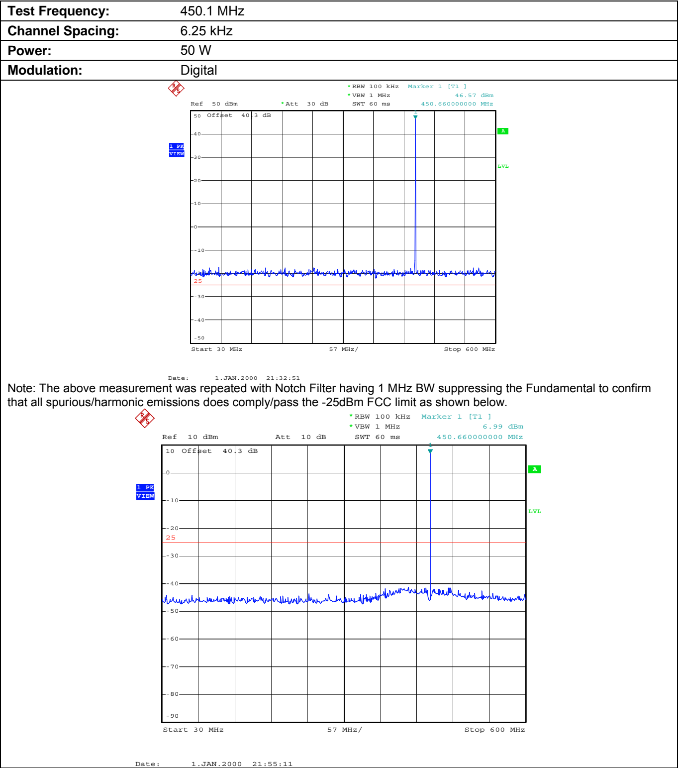
Plot 5.9.4.2.1. Conducted Transmitter Spurious Emissions for 450.1 MHz, High Power, 30 MHz - 600 MHz
