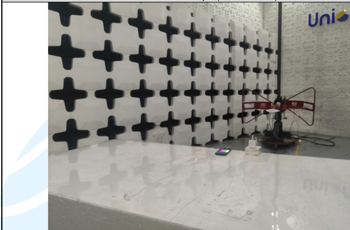
Radiated emission Test Setup-1 (30 MHz~1 GHz)-Mode 5
