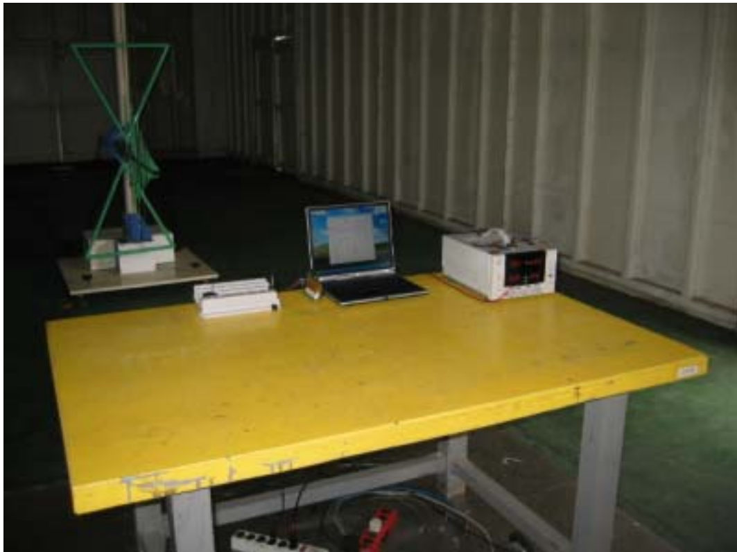
Back View of Radiated Test (Mode 7)
