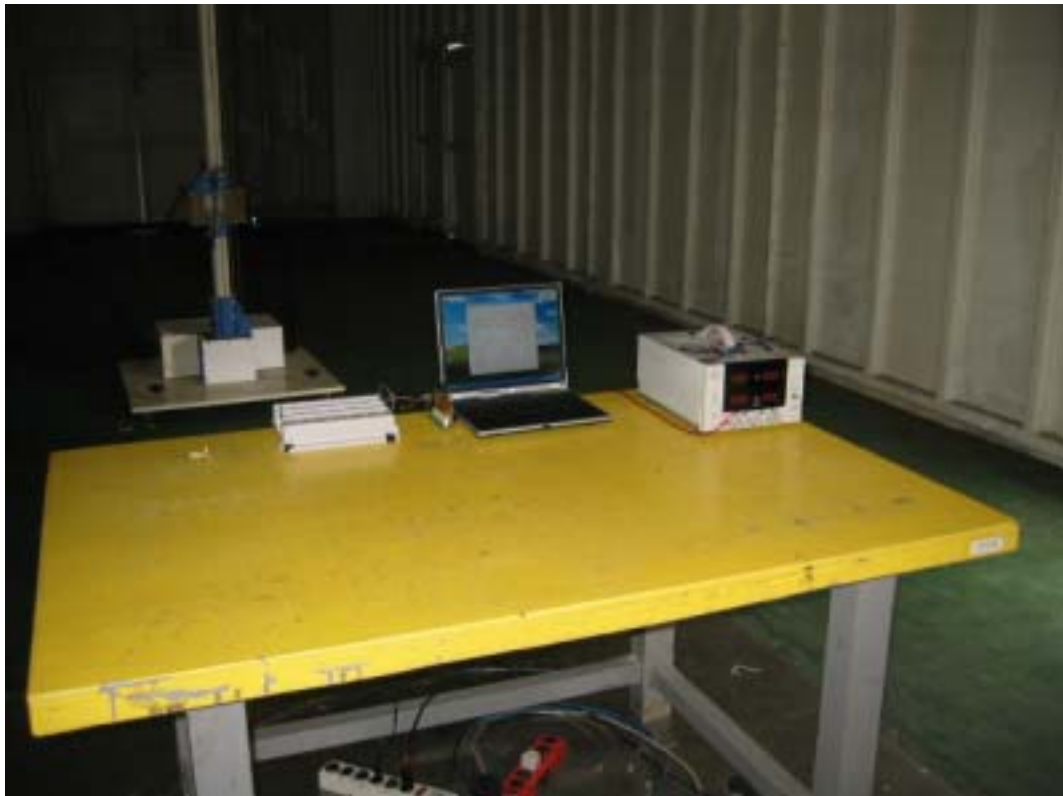
Front View of High Frequency Radiated Test (Mode 4)
