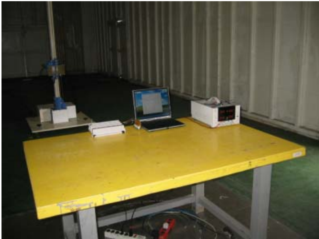
Front View of High Frequency Radiated Test (Mode 9)
