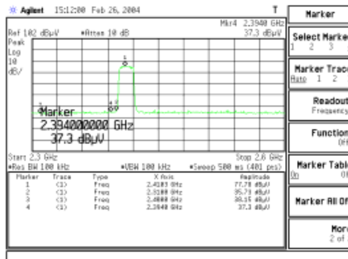
Figure Channel 1: (Vertical)
