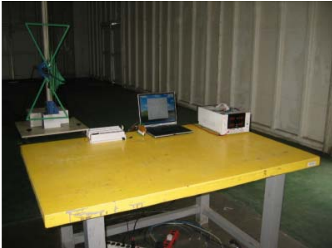
Back View of Radiated Test (Mode 8)
