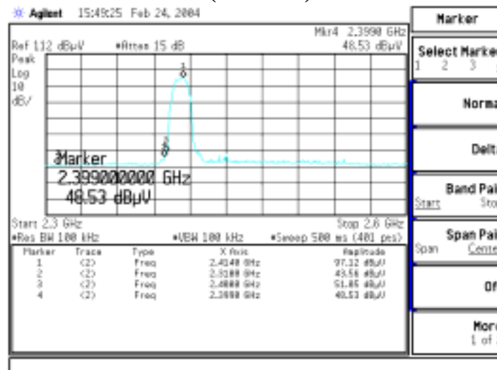
Figure Channel 1: (Horizontal)
