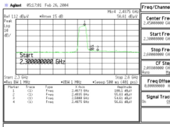
Figure Channel 11: (Vertical)
