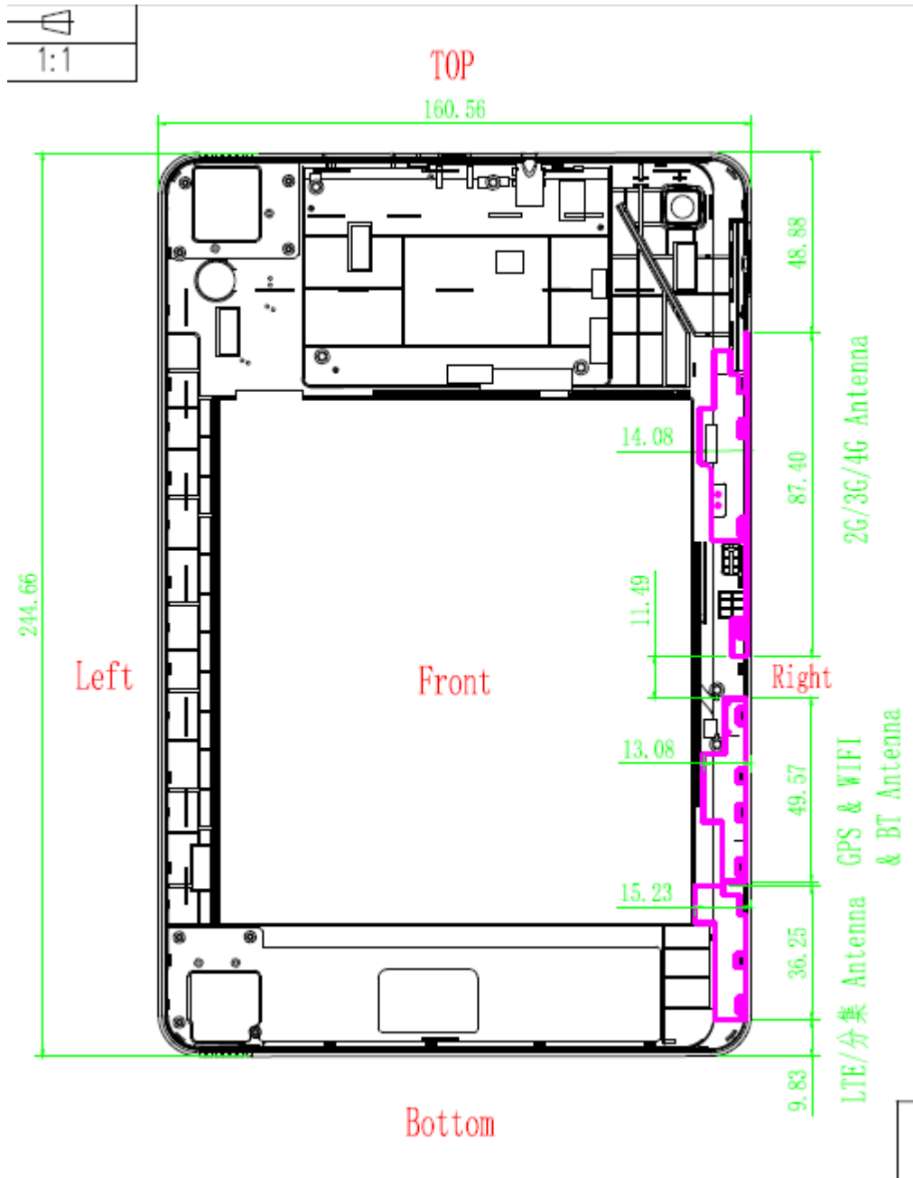
Fig.11.1 EUT Antenna Locations
