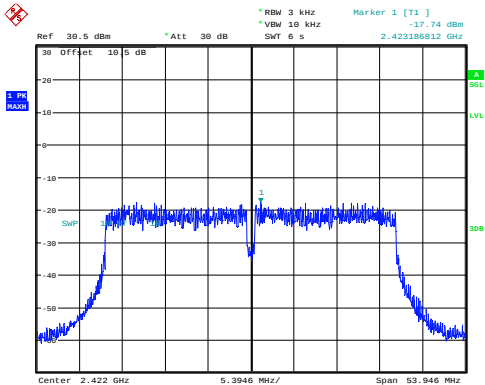
n40_2422MHz_Chain 0 -17.74dBm/3kHz
