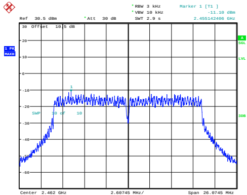
n20_2462MHz_Chain 0 -11.10dBm/3kHz
