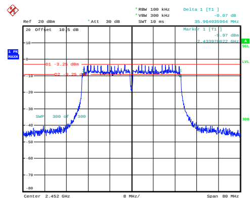
n40_2452MHz_Chain 0 35.964MHz
