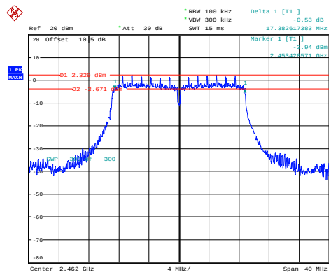
n20_2462MHz_Chain 0 17.383MHz
