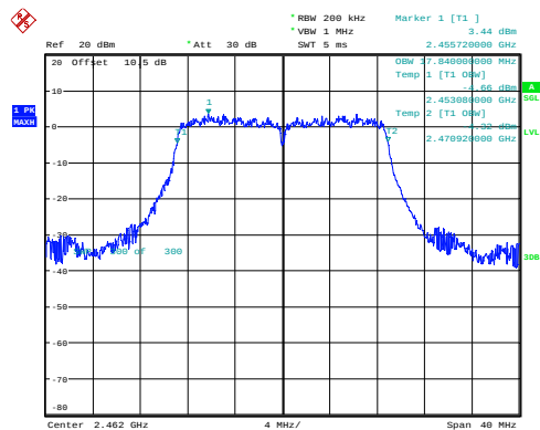
n20_2462MHz_Chain 0 17.840MHz
