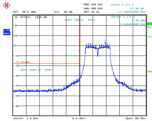
g_2412MHz_Chain 0 34.38dB
