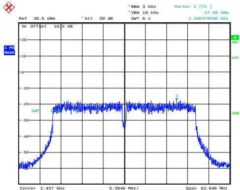
n40_2437MHz_Chain 0 -17.68dBm/3kHz
