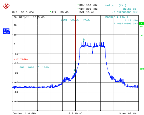
n20_2412MHz_Chain 0 32.63dB
