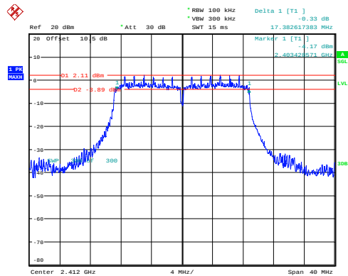
n20_2412MHz_Chain 0 17.383MHz
