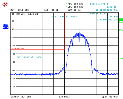
b_2412MHz_Chain 0 41.68dB
