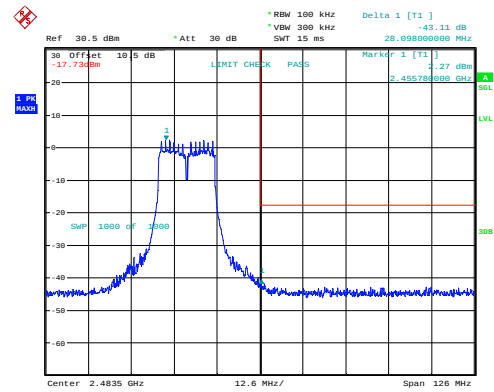
g_2462MHz_Chain 0 43.11dB
