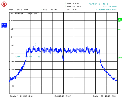
n20_2437MHz_Chain 0 -11.23dBm/3kHz
