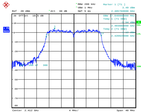
n20_2412MHz_Chain 0 17.840MHz
