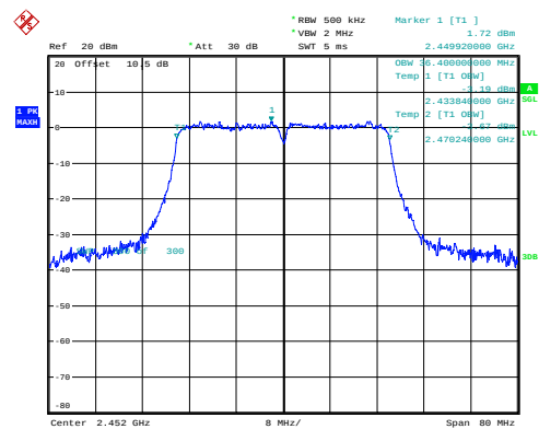
n40_2452MHz_Chain 0 36.400MHz
