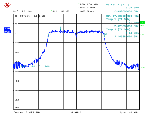
n20_2437MHz_Chain 0 17.800MHz
