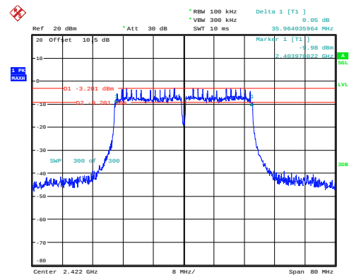
n40_2422MHz_Chain 0 35.964MHz
