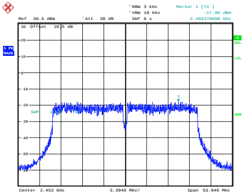
n40_2452MHz_Chain 0 -17.80dBm/3kHz
