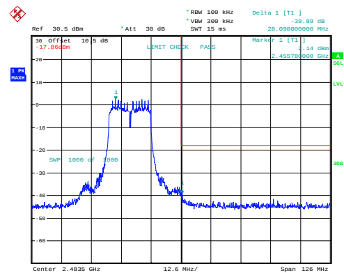
n20_2462MHz_Chain 0 39.89dB
