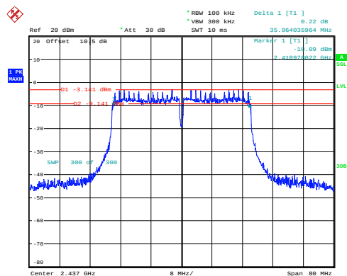
n40_2437MHz_Chain 0 35.964MHz
