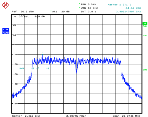
n20_2412MHz_Chain 0 -11.12dBm/3kHz
