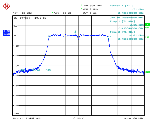
n40_2437MHz_Chain 0 36.400MHz
