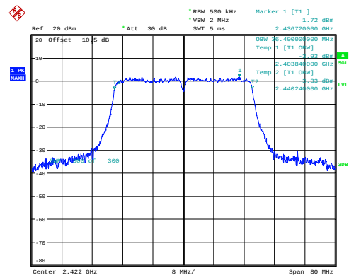
n40_2422MHz_Chain 0 36.400MHz
