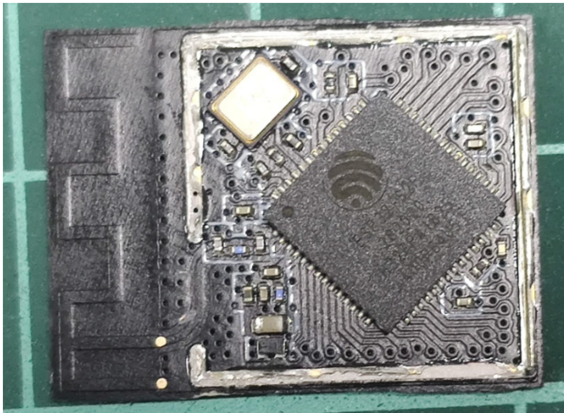
ESP32-S2-MINI-1
