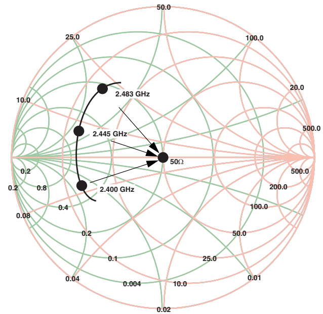
Figure 23. Broadband Match
