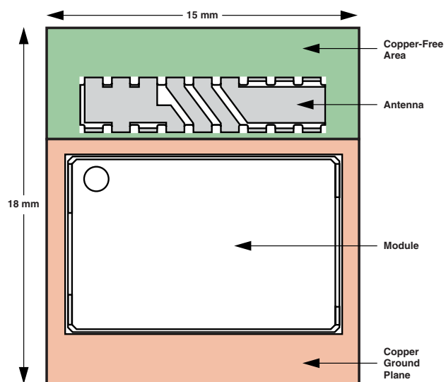
Figure 12. LMX9814/LMX9820 Antenna
