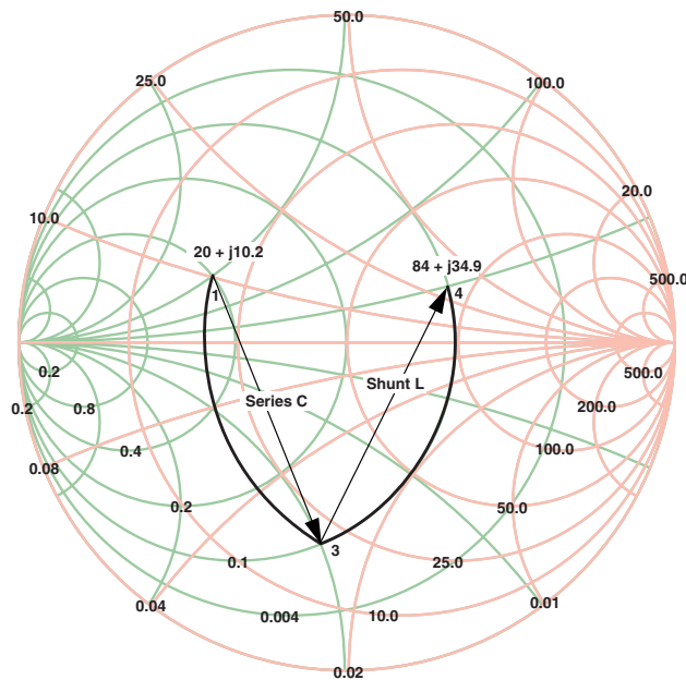
Figure 26. Matching to Non-50Ω Impedance
