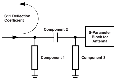
Figure 24. PI Network
