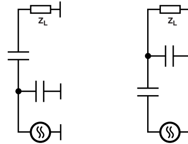
Figure 22. Two Possible Matching Networks
