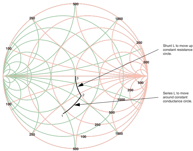
Figure 17. Impedance Transformation
