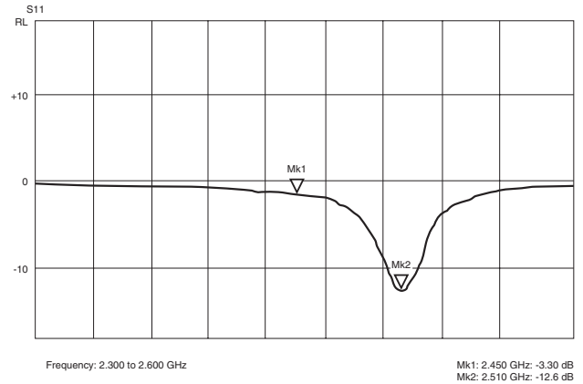
Figure 15. Return Loss, Antenna Connected
