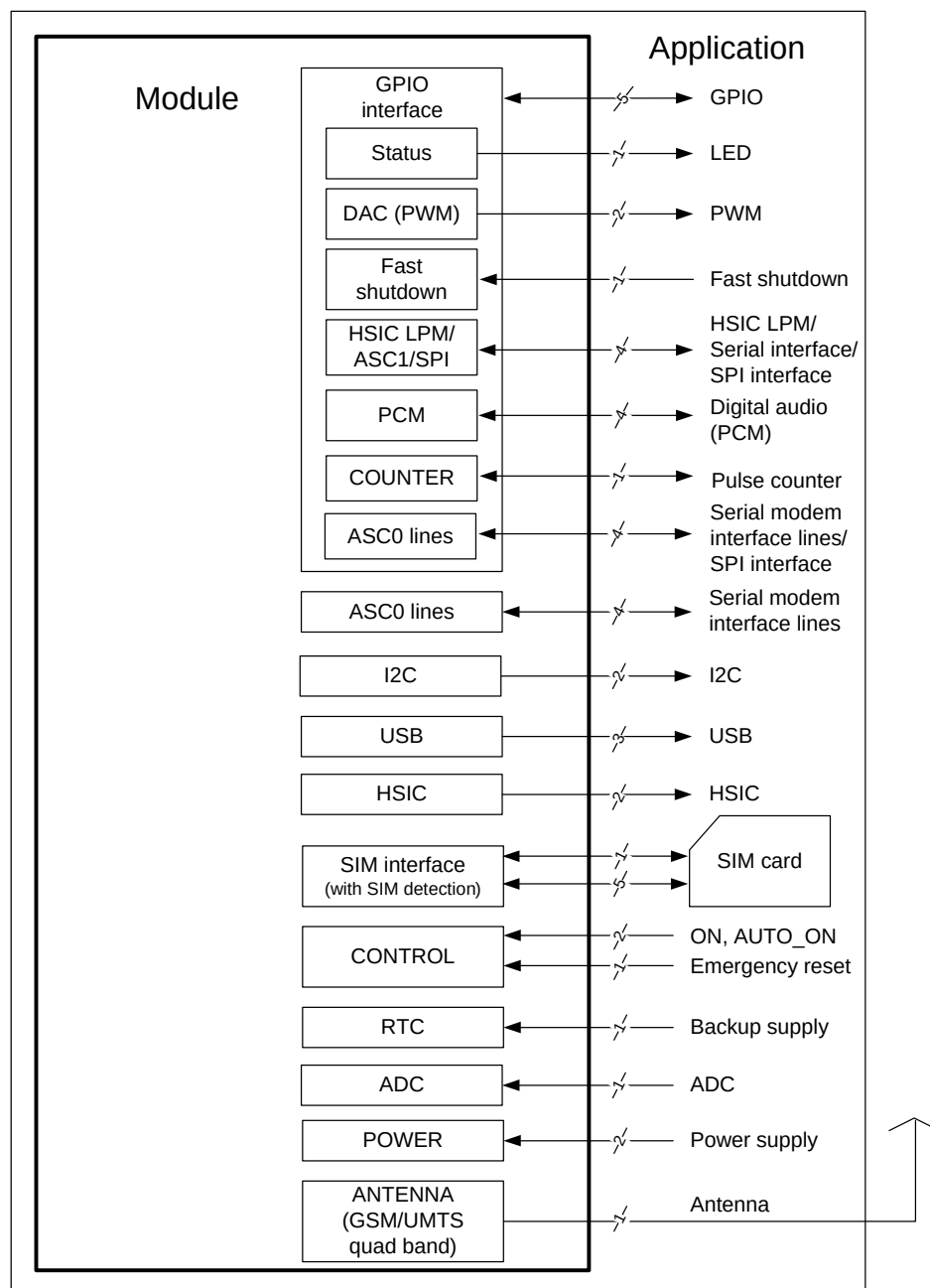
Figure 1: EHS6 system overview
