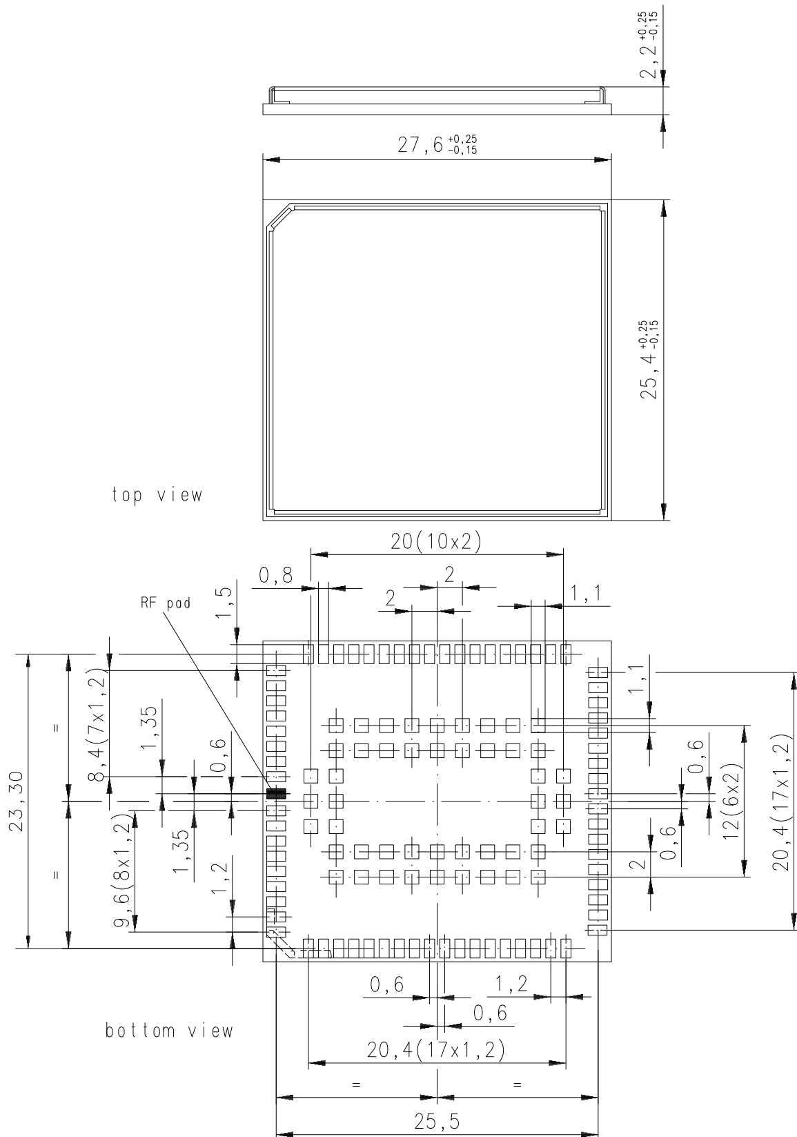
Figure 8: Dimensions of EHS6 (all dimensions in mm)
