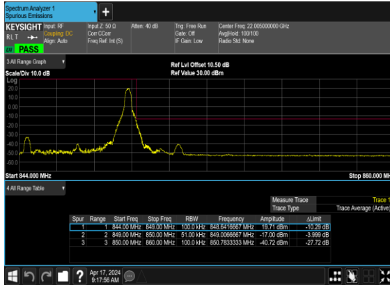
N5(5M)_CP- OFDM_QPSK_Edge_1RB_Right_High_CH
