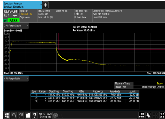
N5(5M)_CP- OFDM_QPSK_Outer_Full_High_CH
