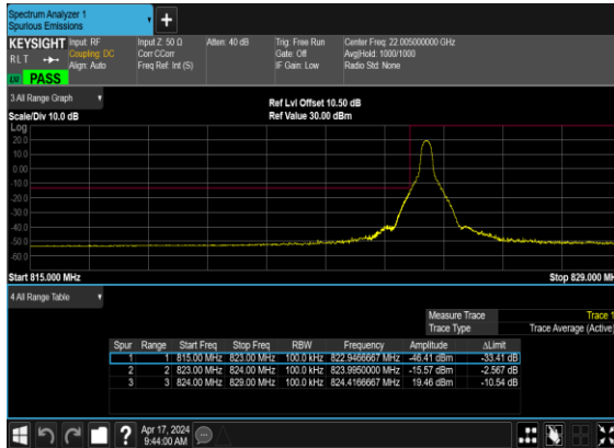
N5(10M)_CP- OFDM_QPSK_Edge_1RB_Left_Low_CH
