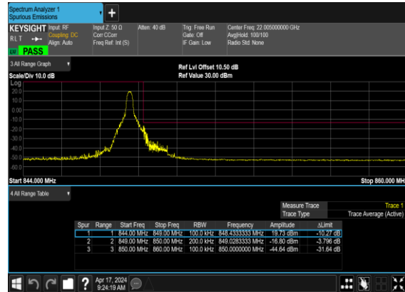
N5(20M)_CP- OFDM_QPSK_Edge_1RB_Right_High_CH
