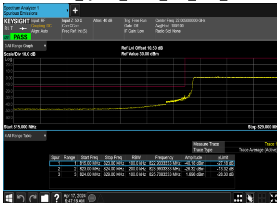
N5(20M)_CP- OFDM_QPSK_Outer_Full_Low_CH
