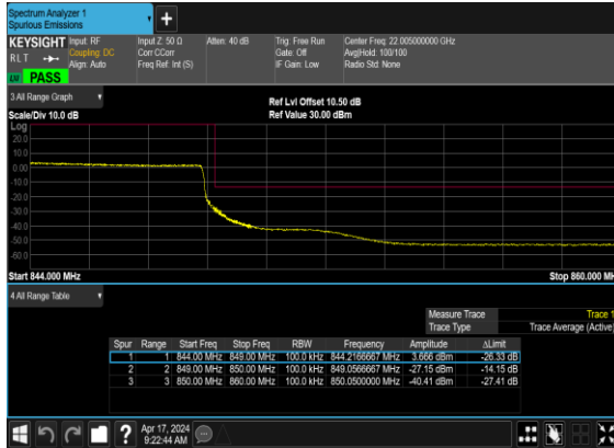
N5(10M)_CP- OFDM_QPSK_Outer_Full_High_CH
