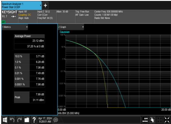
N5(20M)_CP-OFDM_QPSK_Outer_Full_Mid_CH
