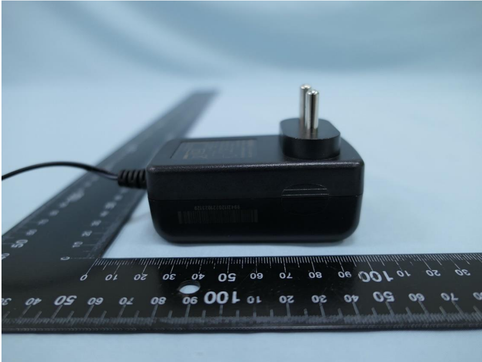
(14) Adapter Photo (MSA-C2000IS12.0-24W-IN)
