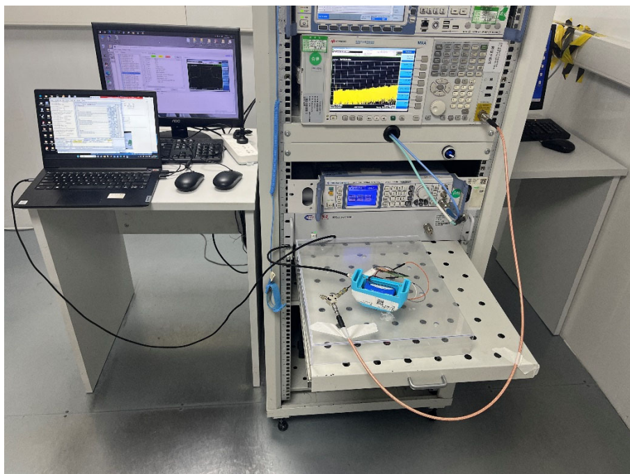
Conducted Test-BLE&LoRa
