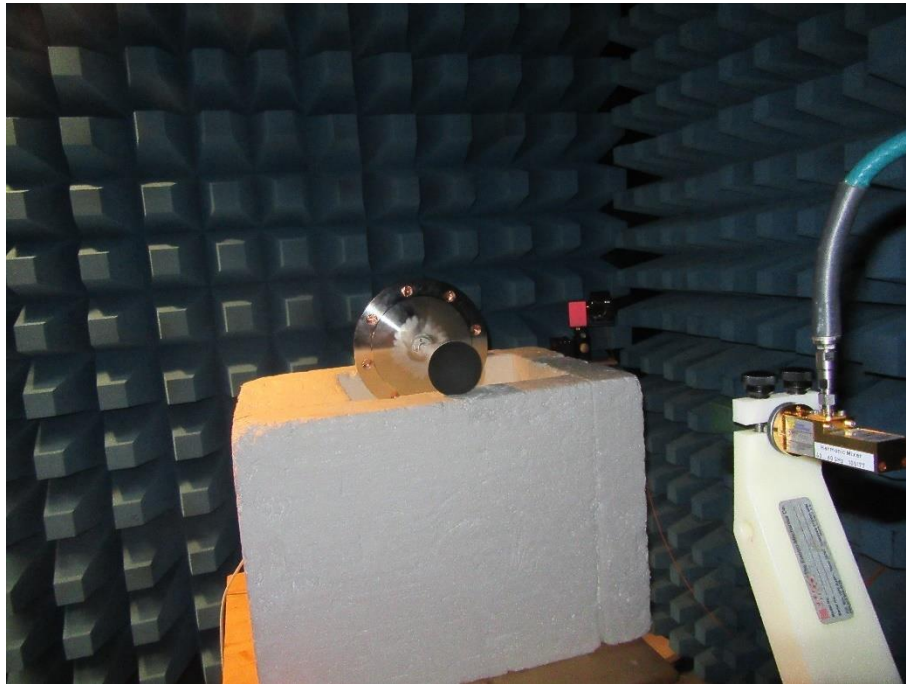
Figure 12 - Test setup for 24.05-29.00 GHz band specific tests
