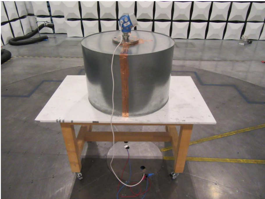
Figure 7 - Test setup for radiated emission on TLPR
