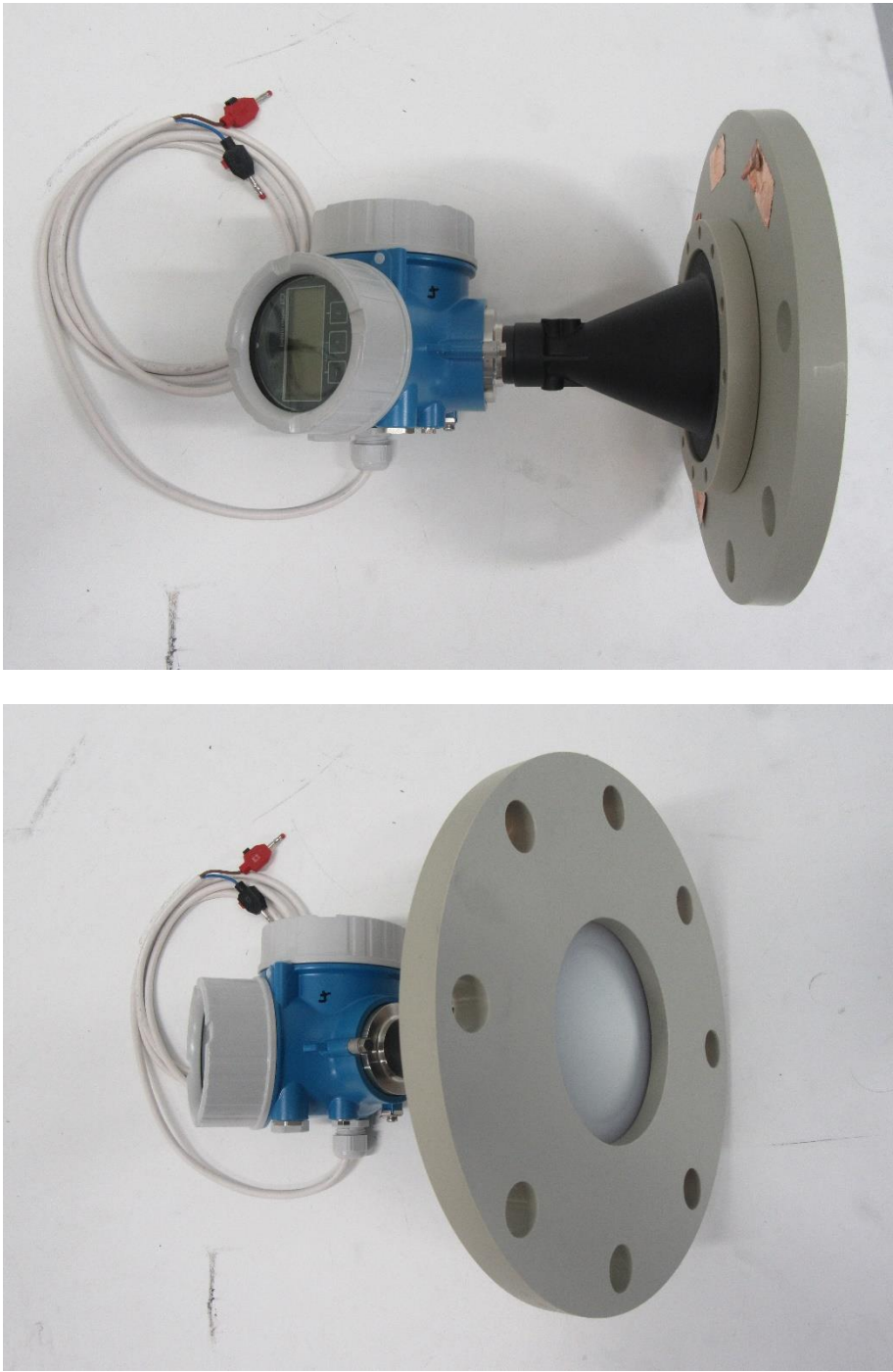
Figure 2 – EUT P4 (FMR51 with antenna Horn 100mm/4")
