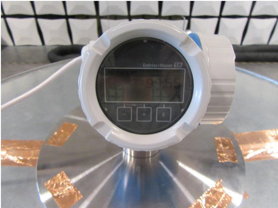
Figure 8 - Test setup for radiated emission on TLPR
