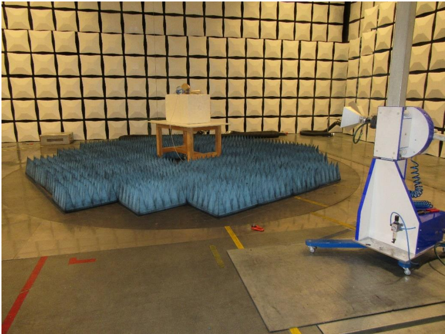
Figure 10 - Test setup for radiated emission on LPR
