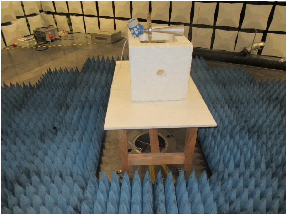
Figure 11 - Test setup for radiated emission on LPR
