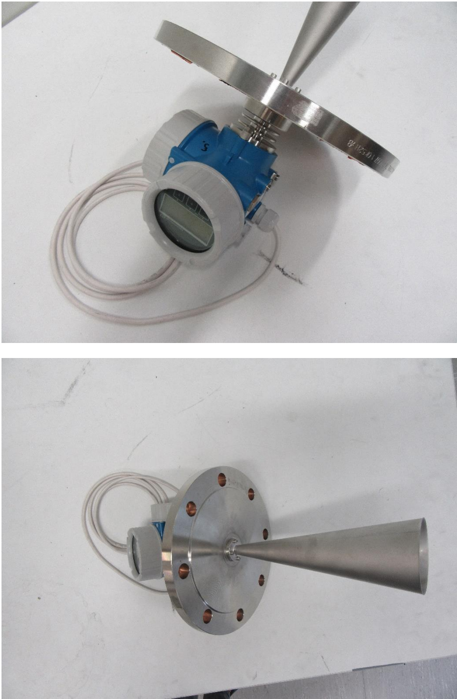
Figure 3 – EUT P5 (FMR52 with antenna Horn 80mm/3" flush mount)
